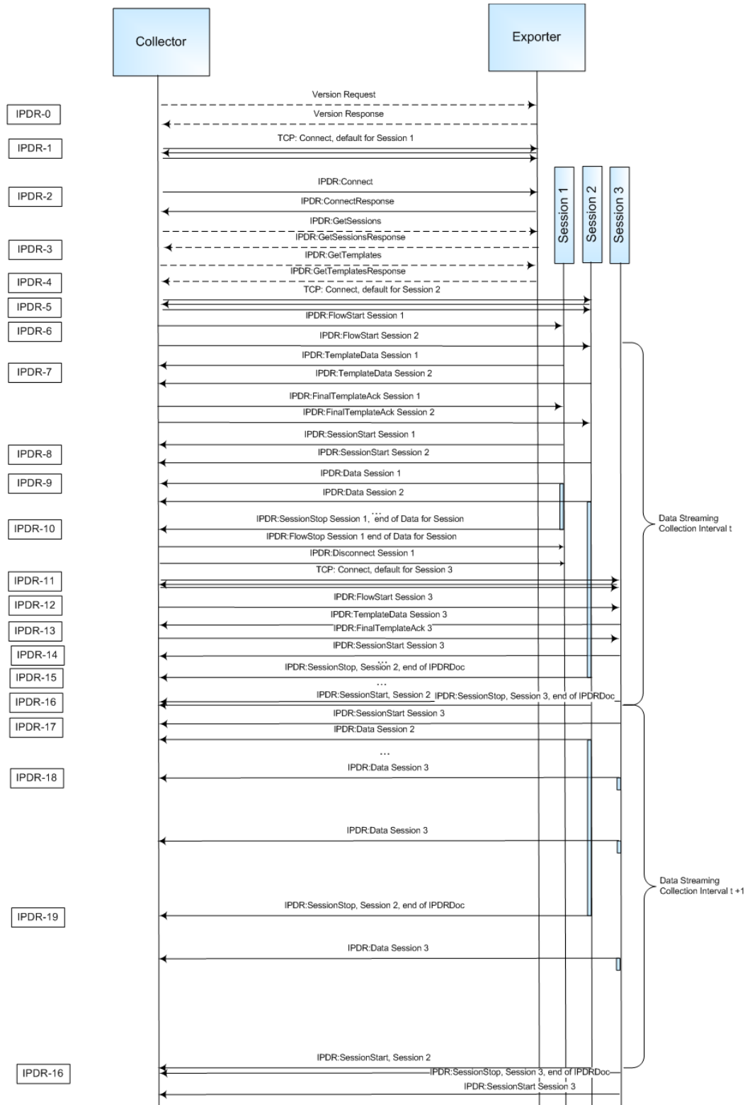
Figure 6-6 - Sequence Diagram for a Multisession Streaming Example 24
