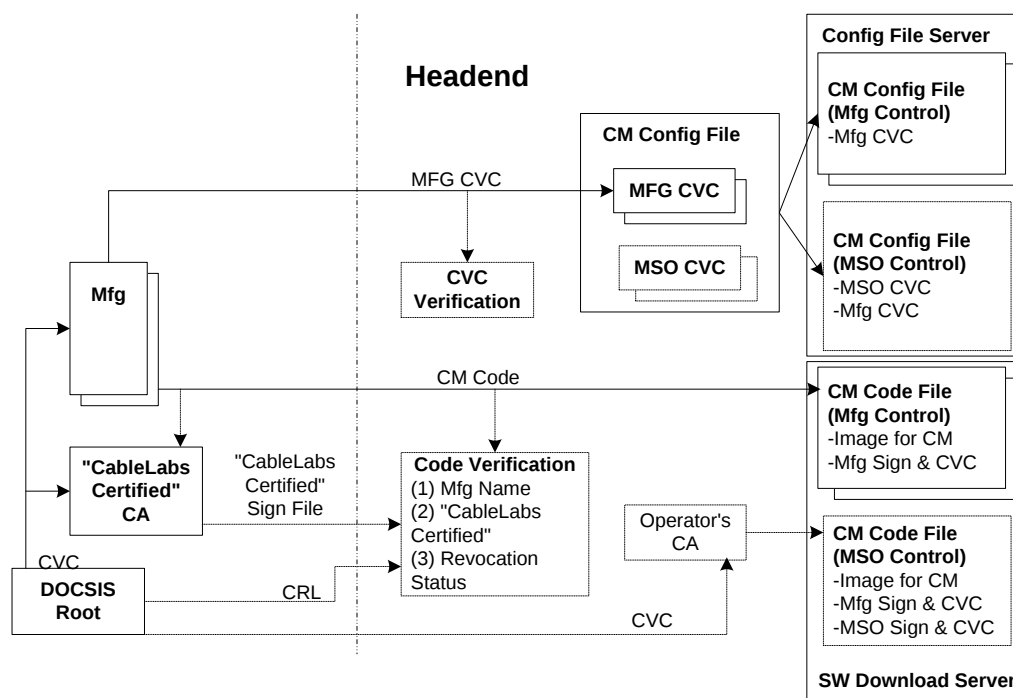
Figure II-1 - Authentication of the Code File for the CM
