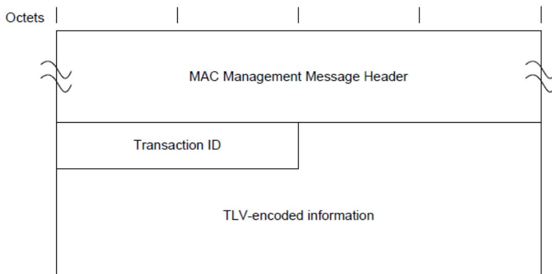
Figure 74 - Dynamic Bonding Change Acknowledge Message
