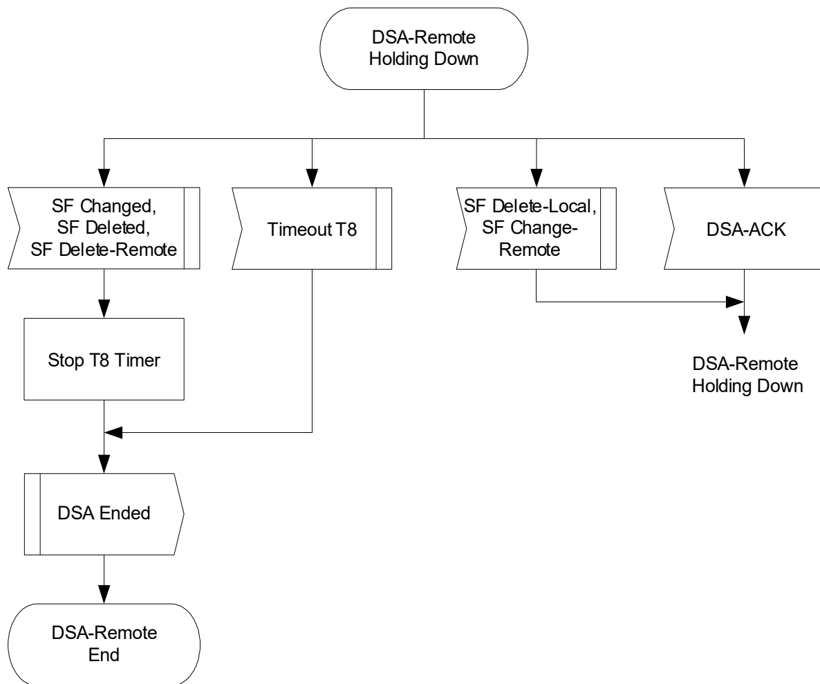
Figure 218 - DSA-Remotely Initiated Transaction Holding Down State Flow Diagram
