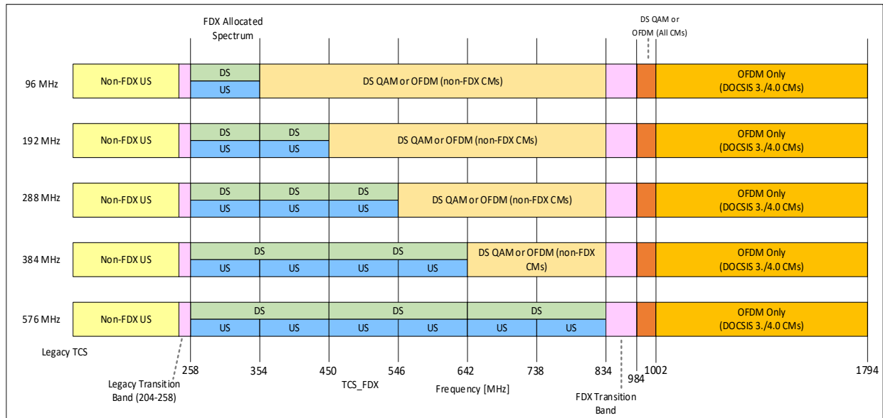
Figure 266 - Configurable FDX Allocated Spectrum Bandwidths for SFDX Band Plan
