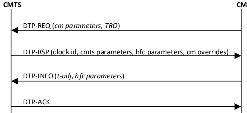
Figure 199 - CM is DTP Master
