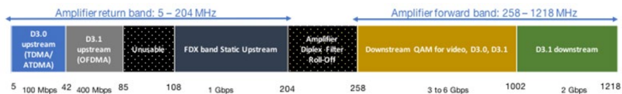
Figure 329 - Static FDX Upstream Spectrum Usage Example
