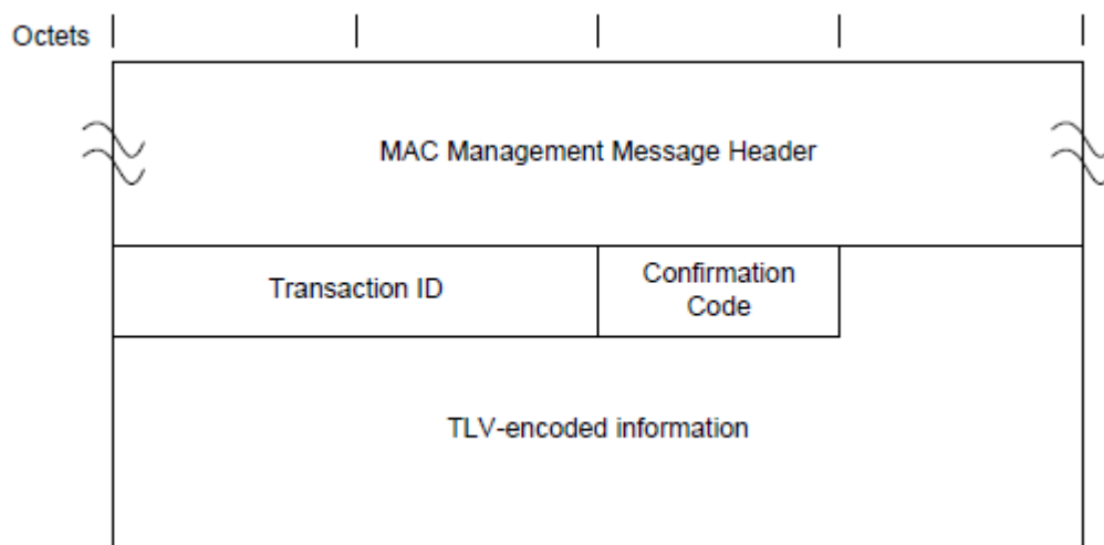
Figure 61 - Dynamic Service Addition - Acknowledge
