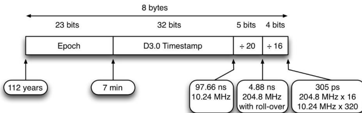
Figure 106 - Extended Timestamp Structure
