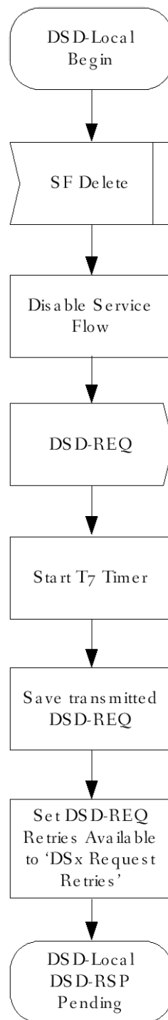
Figure 234 - DSD-Locally Initiated Transaction Begin State Flow Diagram
