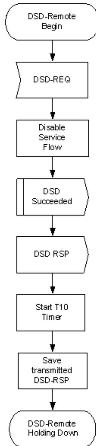
Figure 237 - DSD-Remotely Initiated Transaction Begin State Flow Diagram
