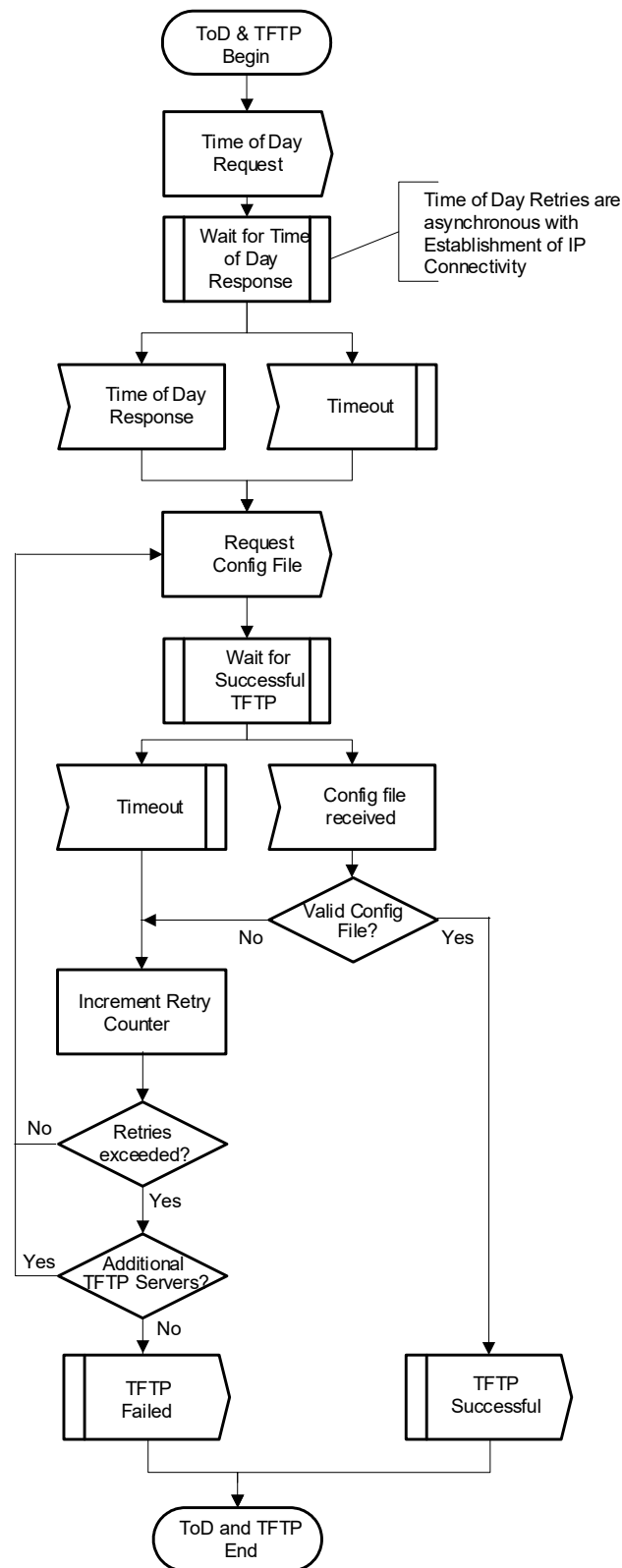
Figure 164 - ToD and TFTP
