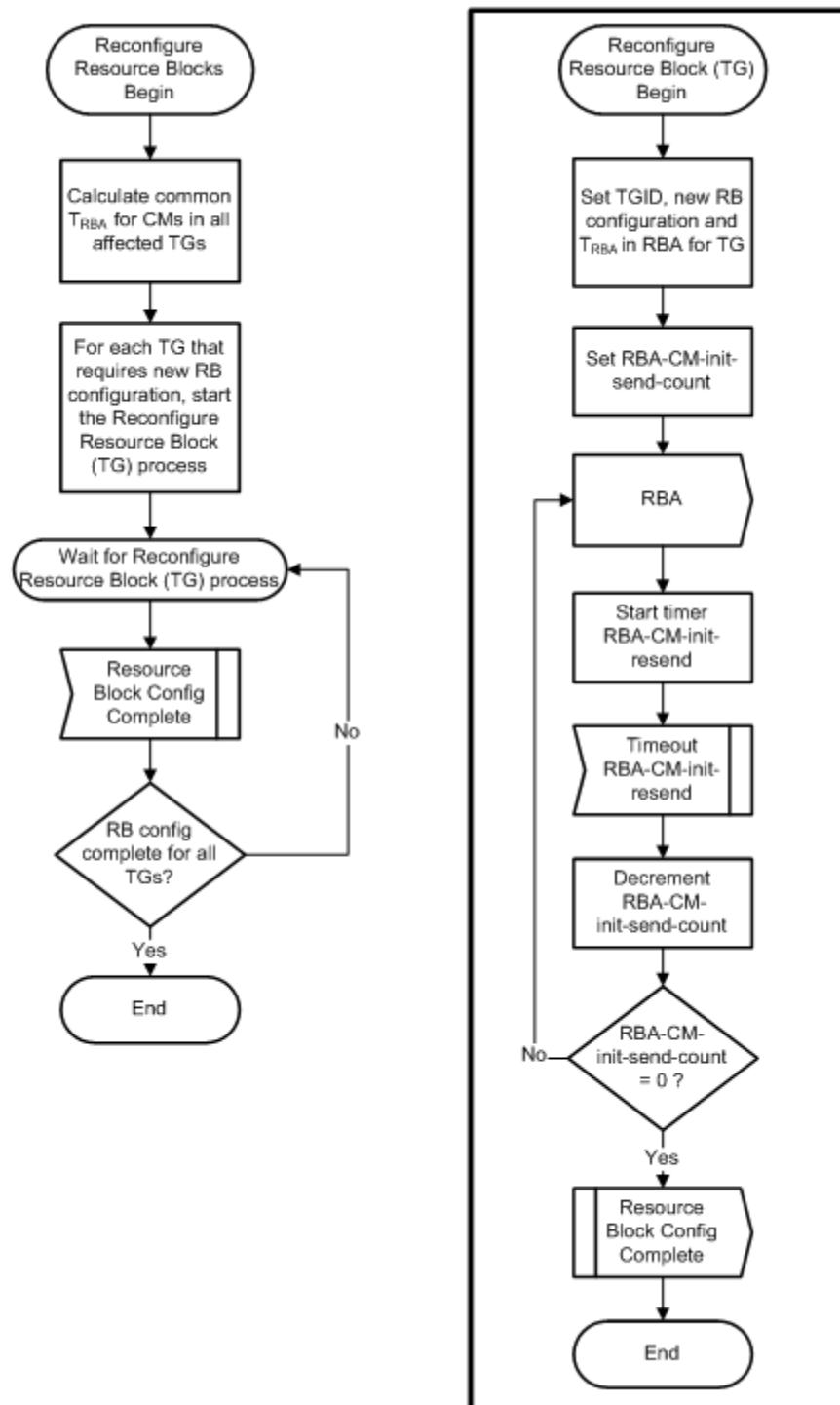
Figure 269 - Reconfigure Resource Blocks
