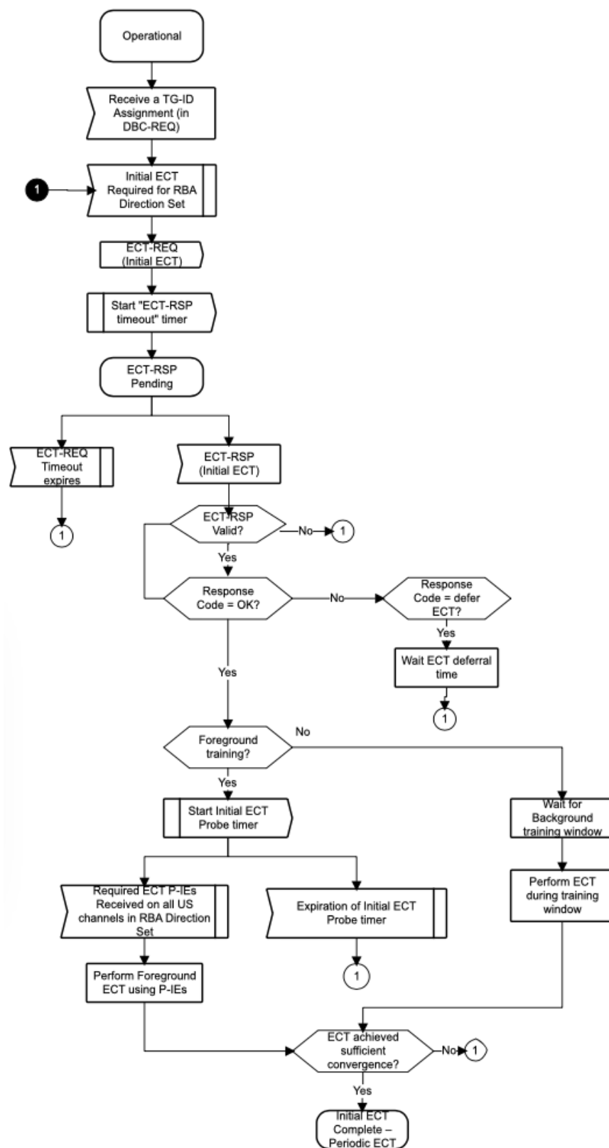
Figure 283 - CM – Initial ECT SDL
