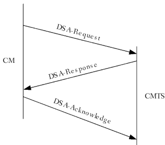
Figure 121 - Dynamic Service Addition Message Flow – CM Initiated
