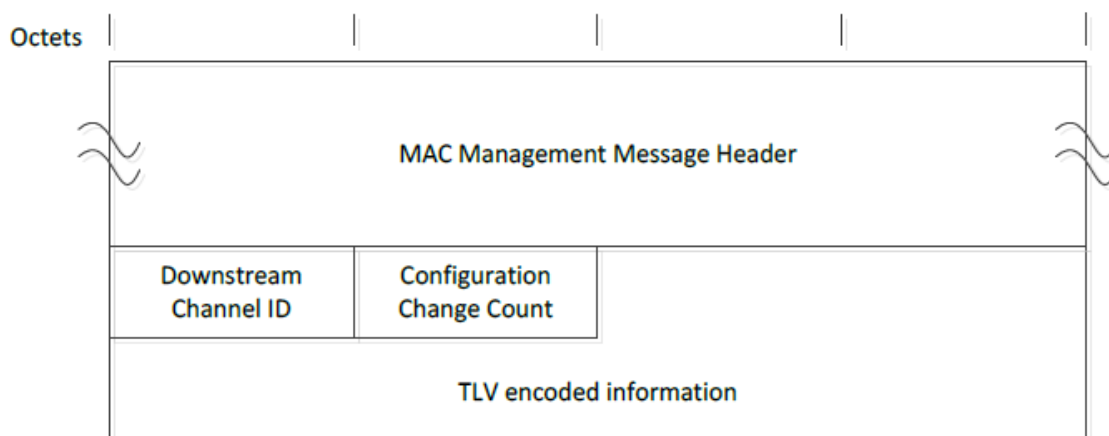
Figure 83 - OFDM Channel Descriptor
