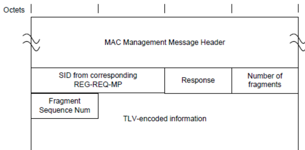
Figure 57 - Multipart Registration Response Format
