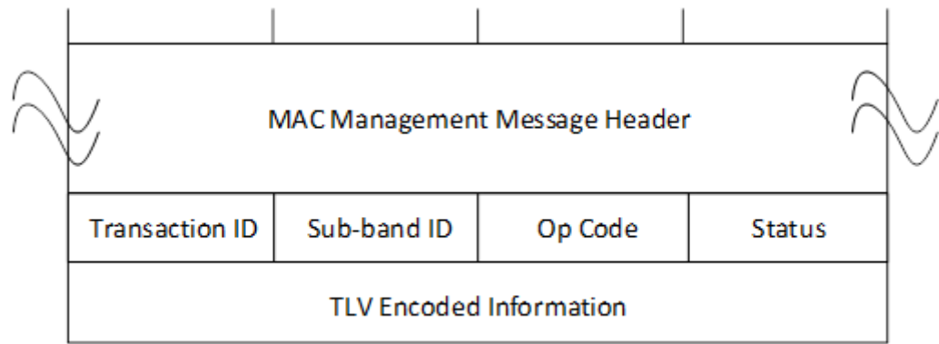
Figure 95 - CW Test Response (CWT-RSP) Message
