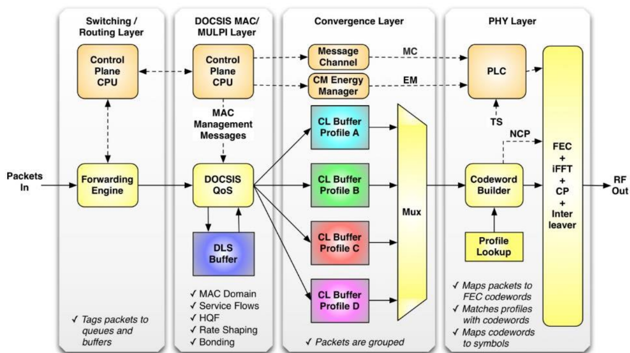
Figure 10 - Downstream Convergence Layer Block Diagram
