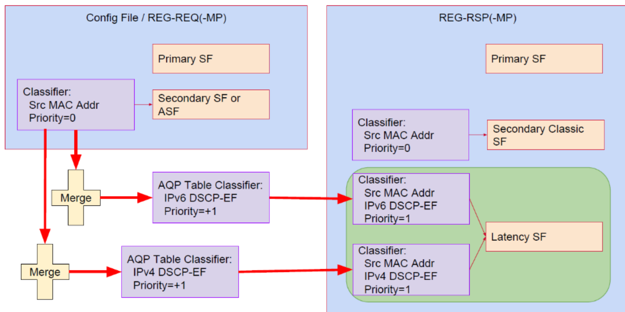
Figure 132 - Classifier Merge Example 2
