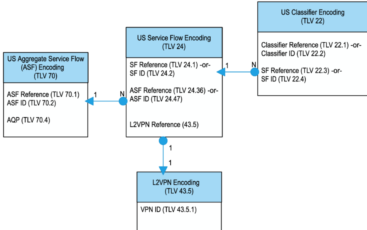
Figure 123 - Relationship of Upstream Classifiers, Service Flows, ASFs and L2VPN
