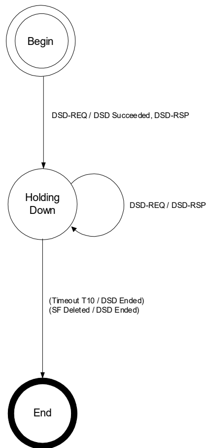
Figure 208 - Dynamic Deletion (DSD)--- Remotely Initiated Transaction State Transition Diagram
