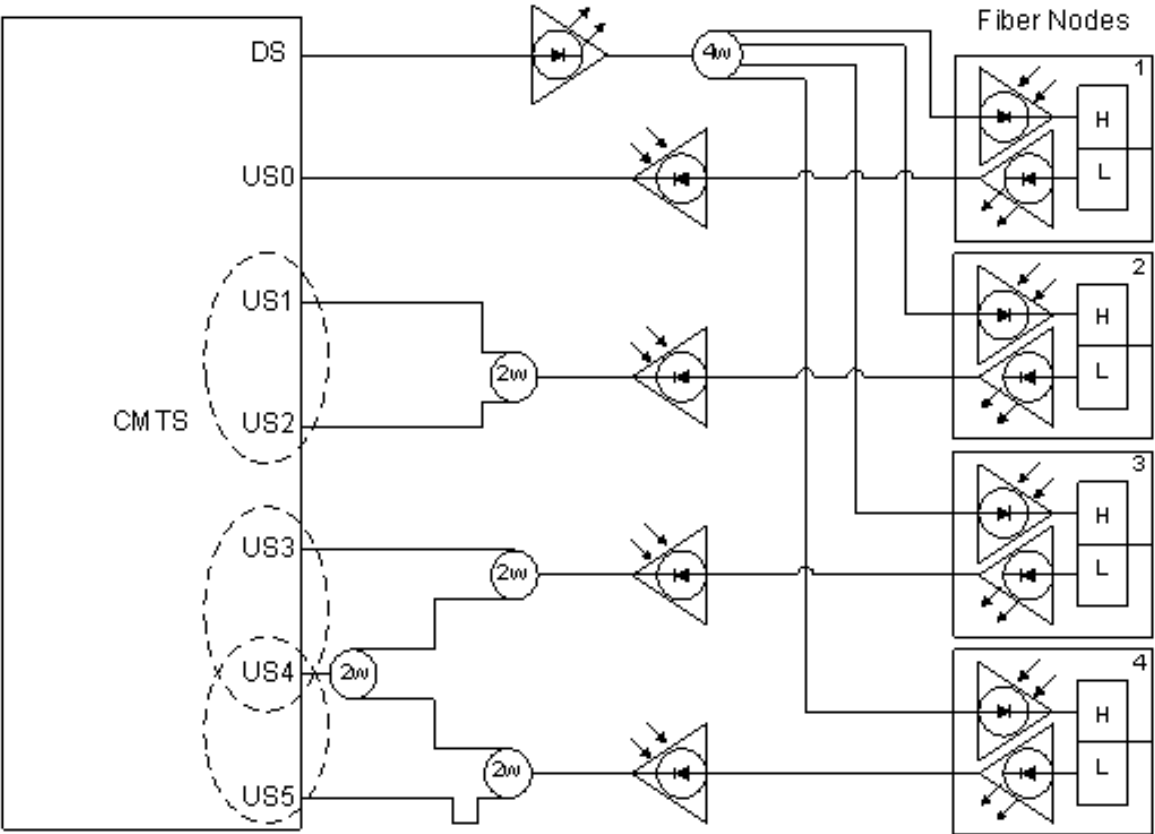
Figure 324 - Example Combining Network 1
