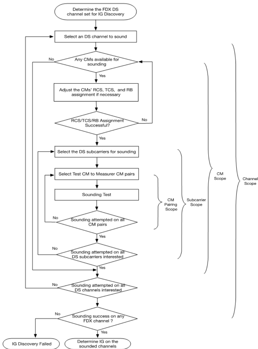
Figure 272 - High-level IG Discovery Transaction Diagram
