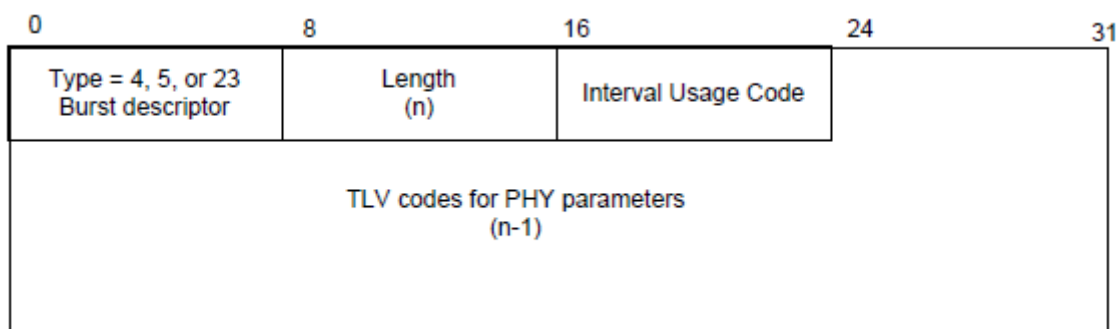
Figure 36 - Top-Level Encoding for Burst Descriptors
