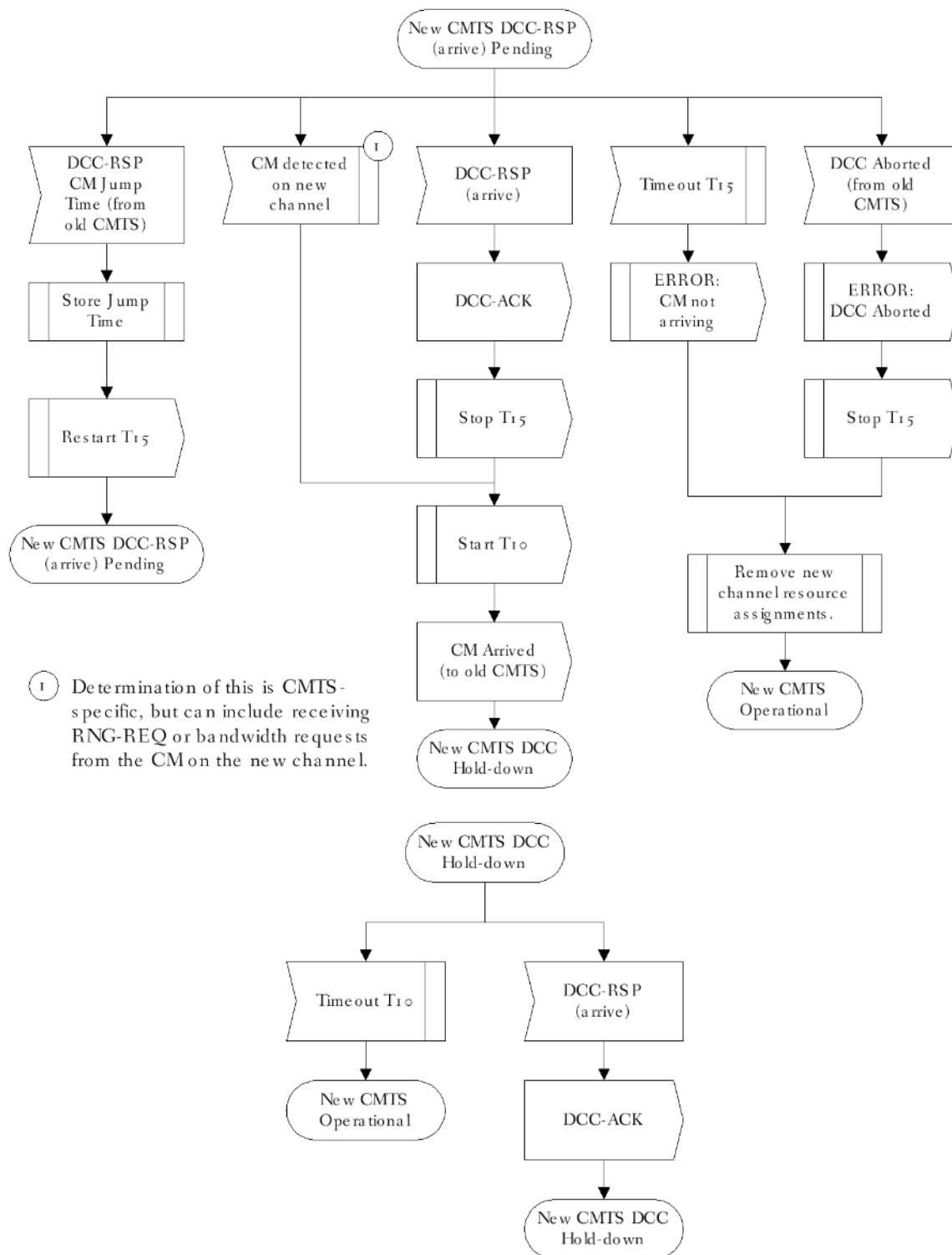
Figure 242 - Dynamically Changing Channels: CMTS View Part 4
