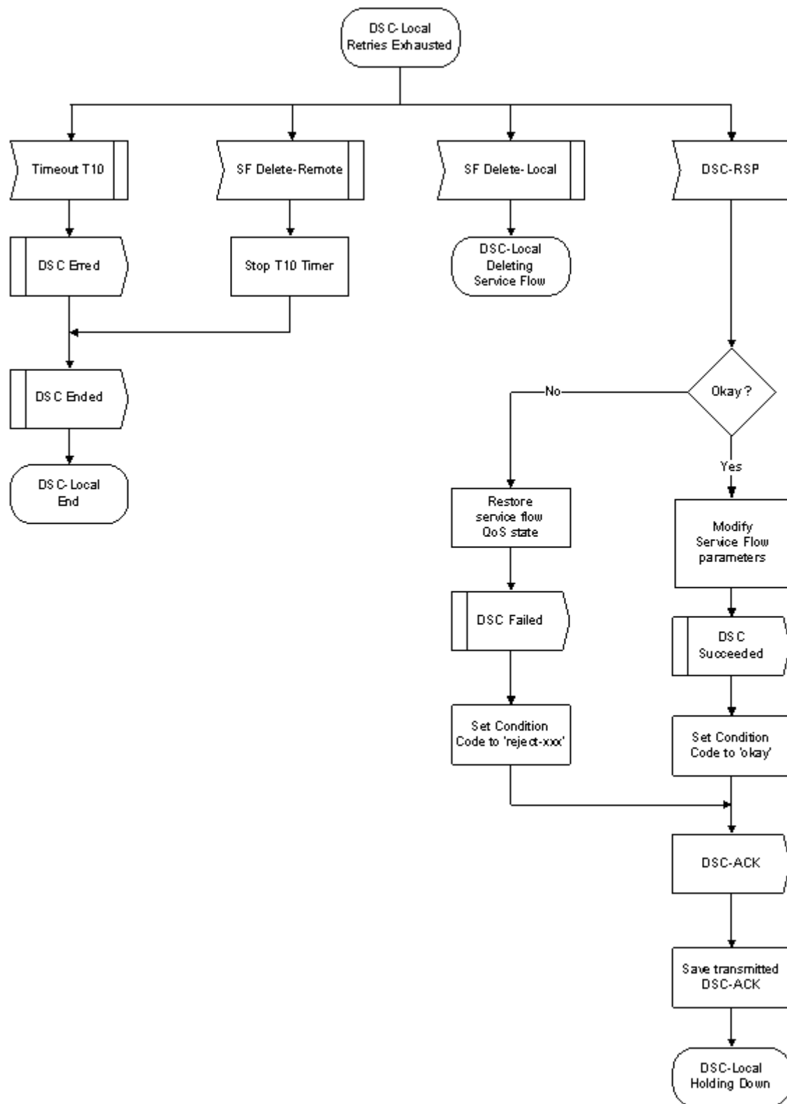
Figure 226 - DSC-Locally Initiated Transaction Retries Exhausted State Flow Diagram
