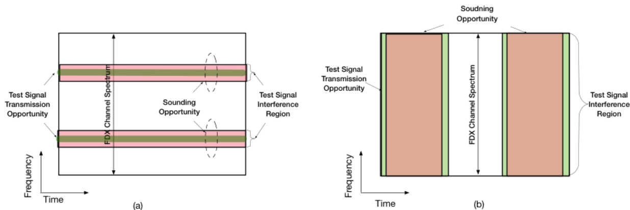
Figure 270 - Sounding Opportunities (a) CWT Sounding (b) OUDP Sounding
