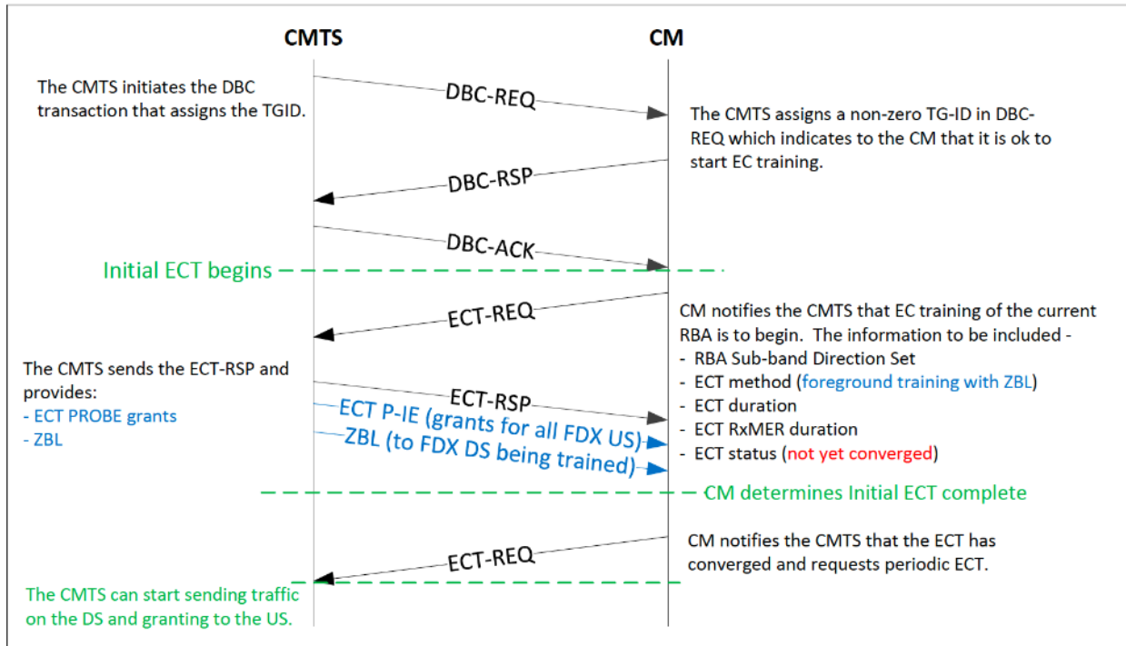
Figure 279 - Initial Foreground Training with ZBL
