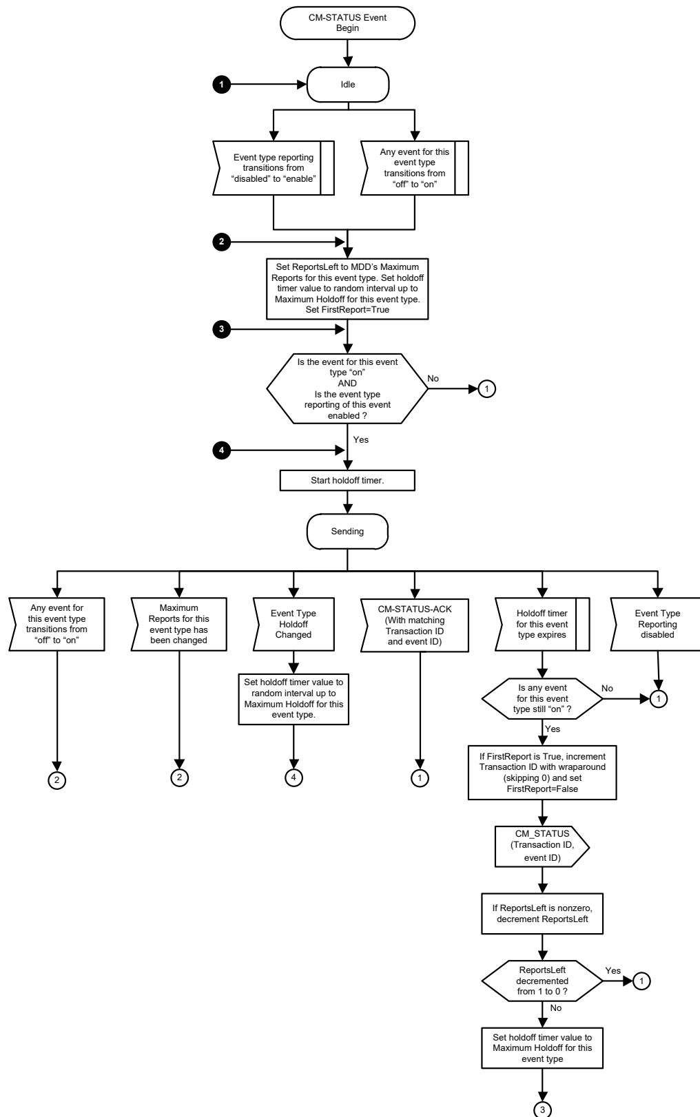
Figure 191 - CM-STATUS Event Type State Machine
