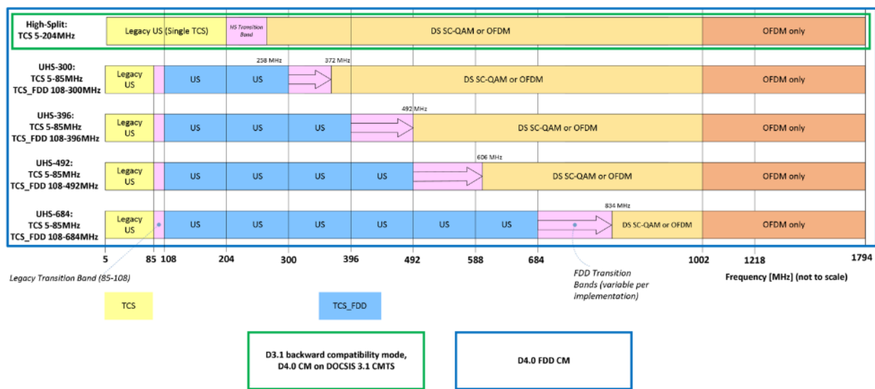
Figure 291 - FDD Spectrum Usage Alternatives: CM View
