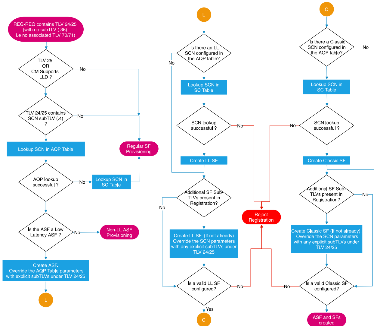
Figure 129 - Service Flow TLV Handling
