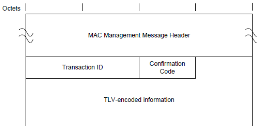
Figure 60 - Dynamic Service Addition - Response
