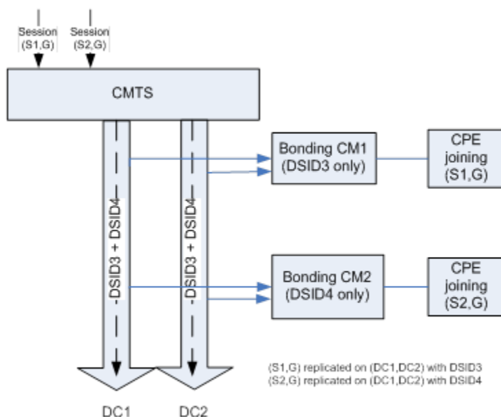
Figure 141 - DSIDs Separate Source-Specific Multicast Sessions
