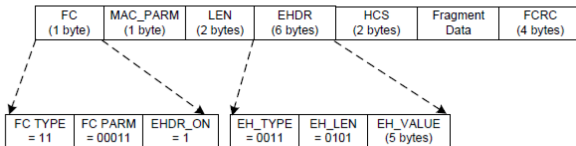
Figure 27 - Fragmentation MAC Header Format
