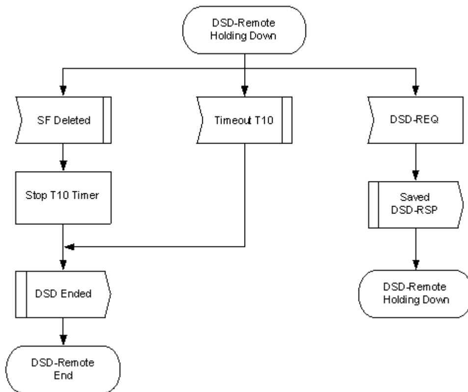
Figure 238 - DSD-Remotely Initiated Transaction Holding Down State Flow Diagram
