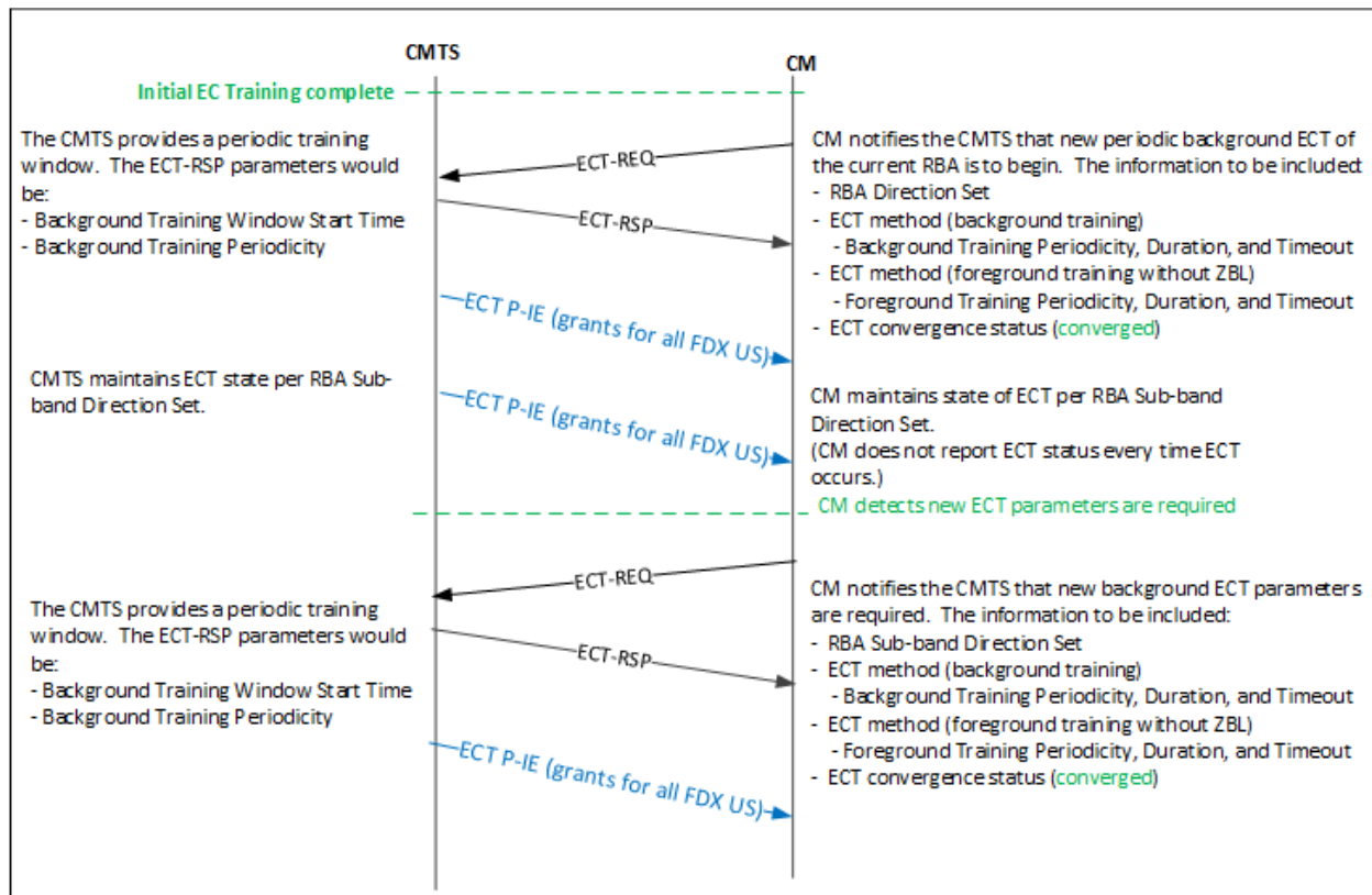
Figure 282 - Periodic EC Training of Background Training and Foreground Training Without ZBL
