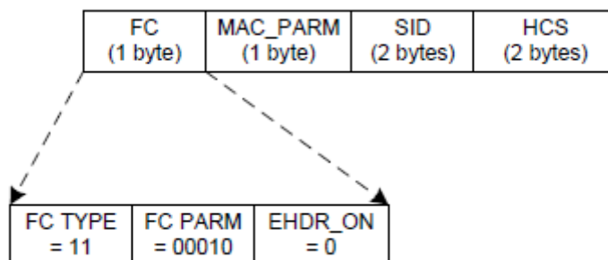
Figure 26 - Request Frame Format
