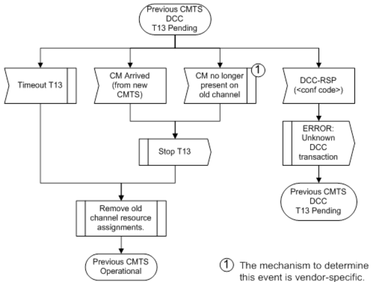
Figure 241 - Dynamically Changing Channels: CMTS View Part 3
