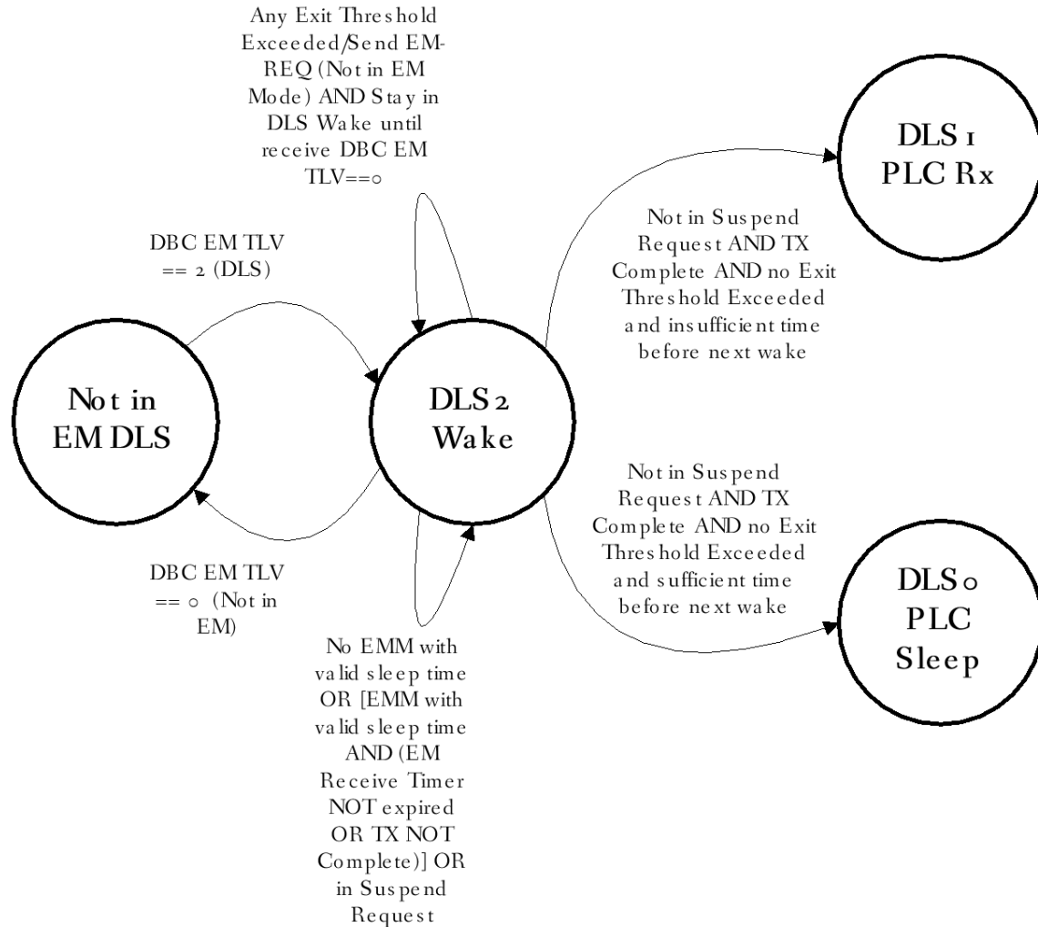
Figure 261 - Wake Substate Transitions for DLS Mode
