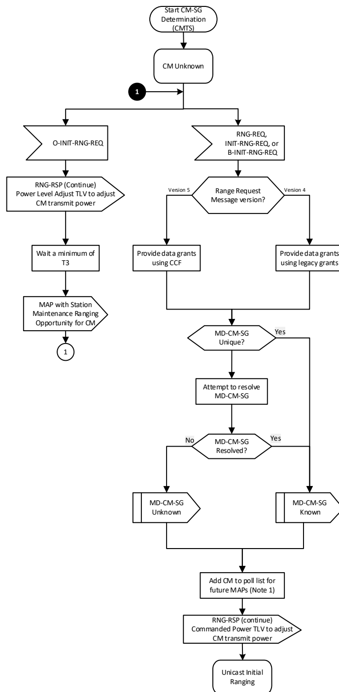
Figure 157 - CM-SG Determination - CMTS
