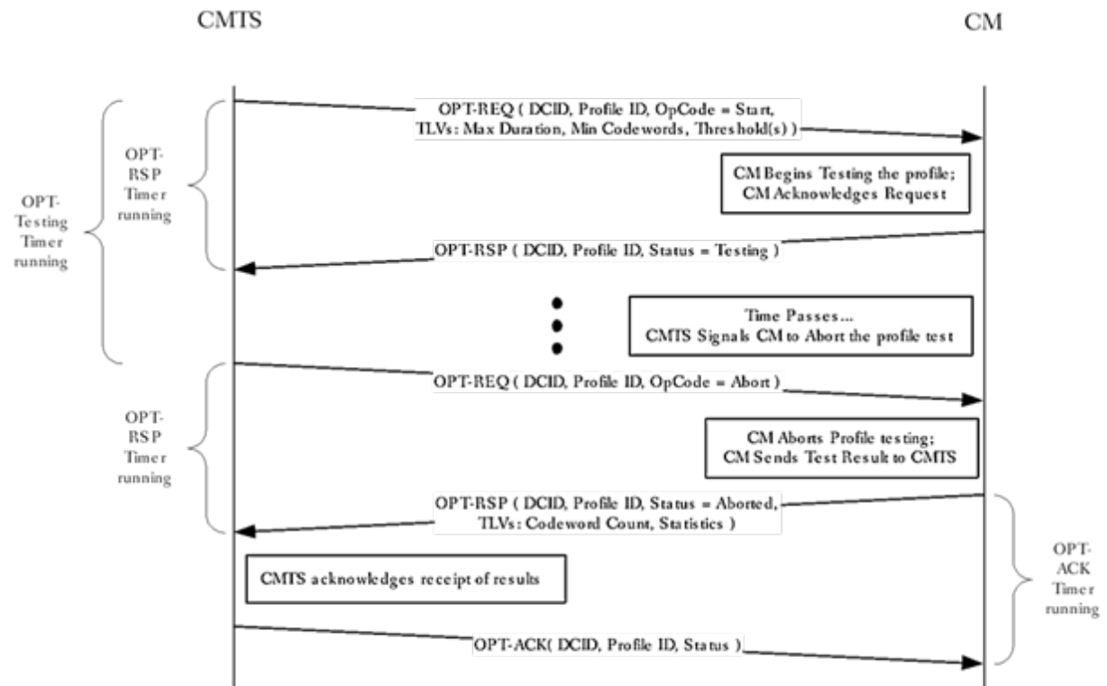
Figure 181 - Aborted OFDM Profile Test Transaction
