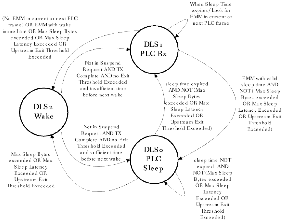
Figure 262 - PLC Rx and PLC Sleep Substate Transitions for DLS Mode
