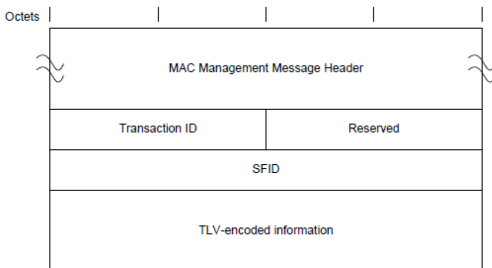
Figure 65 - Dynamic Service Deletion - Request
