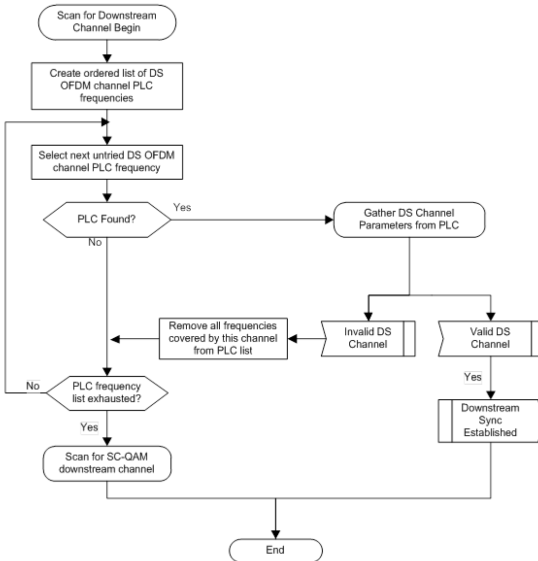
Figure 144 - Scan for Downstream Channel
