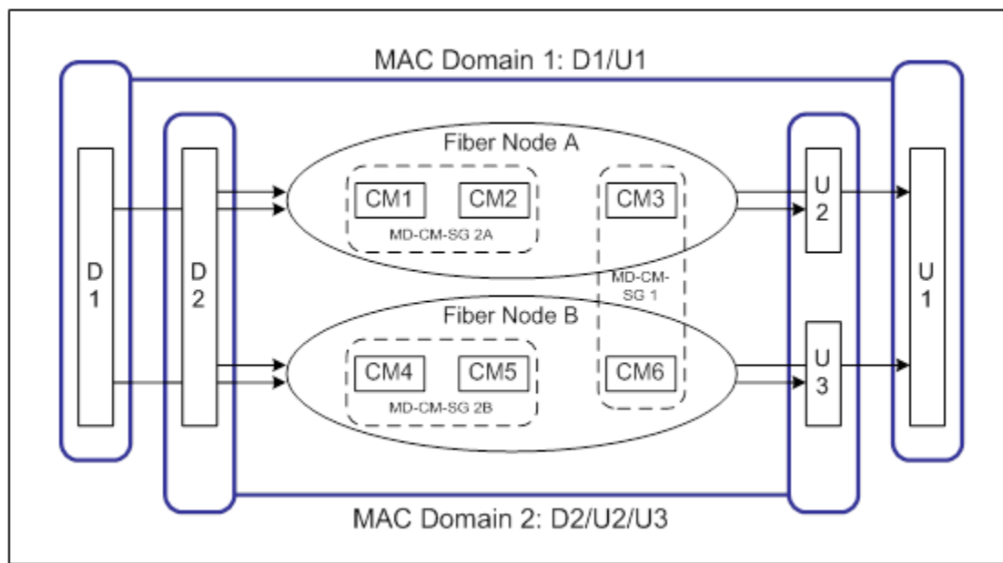
Figure 18 - Multiple MAC Domains per Fiber Node
