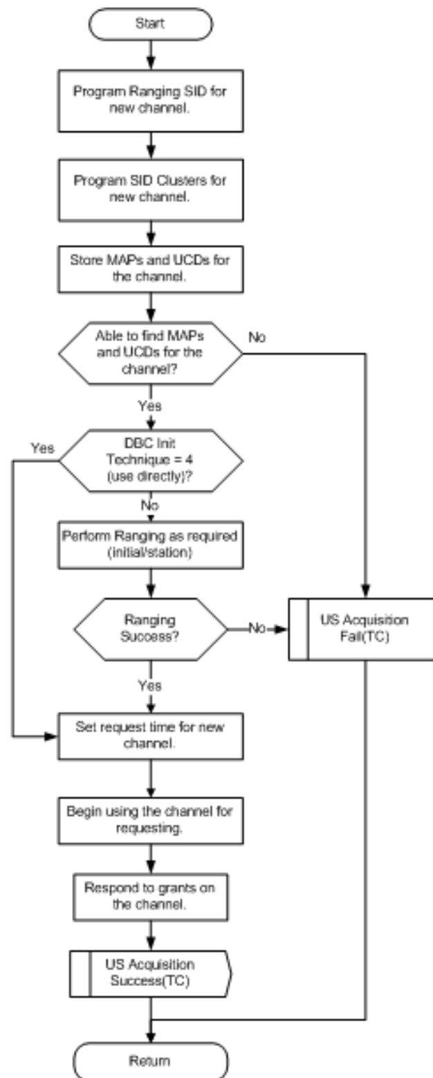
Figure 255 - CM AcquireUS Procedure
