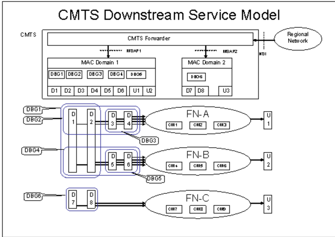
Figure 20 - CMTS Downstream Service Model
