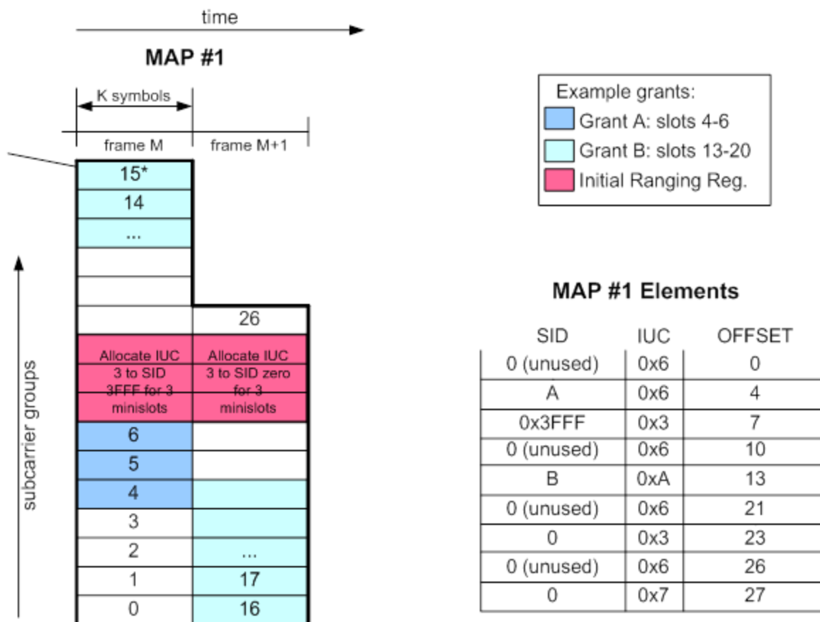
Figure 114 - Example MAP for Initial Ranging Region on an OFDMA Channel
