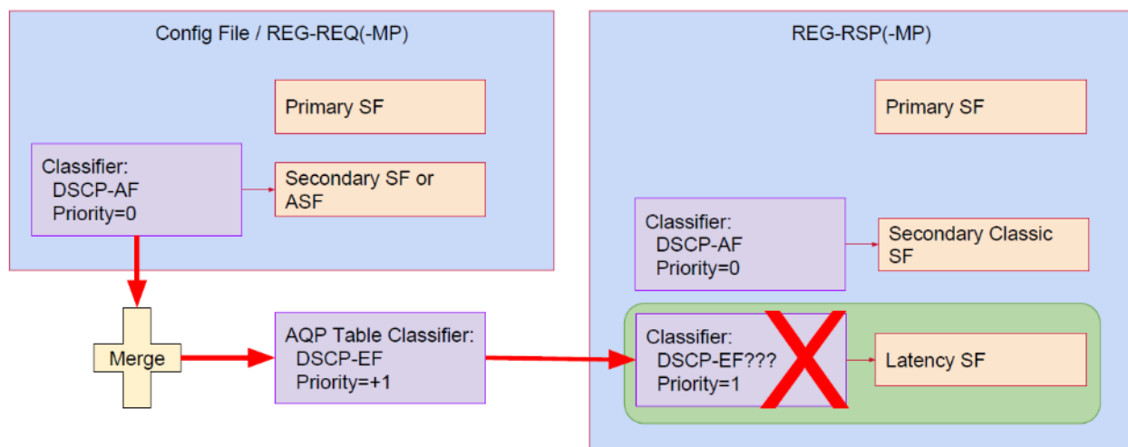
Figure 133 - Classifier Merge Example 3
