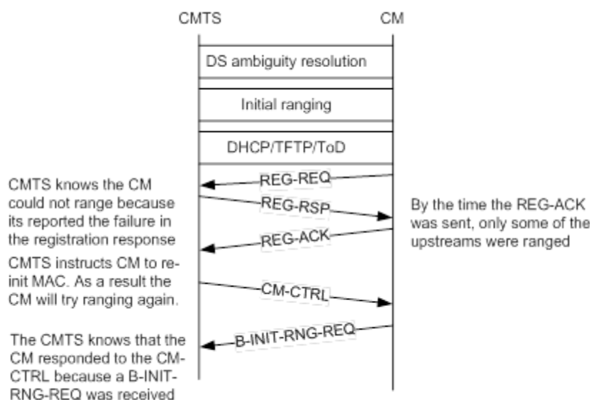
Figure 309 - Example 1 - Modem can't range on all upstreams
