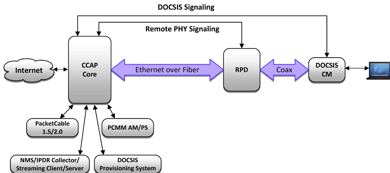
Figure 1 - The Modern DOCSIS Network
