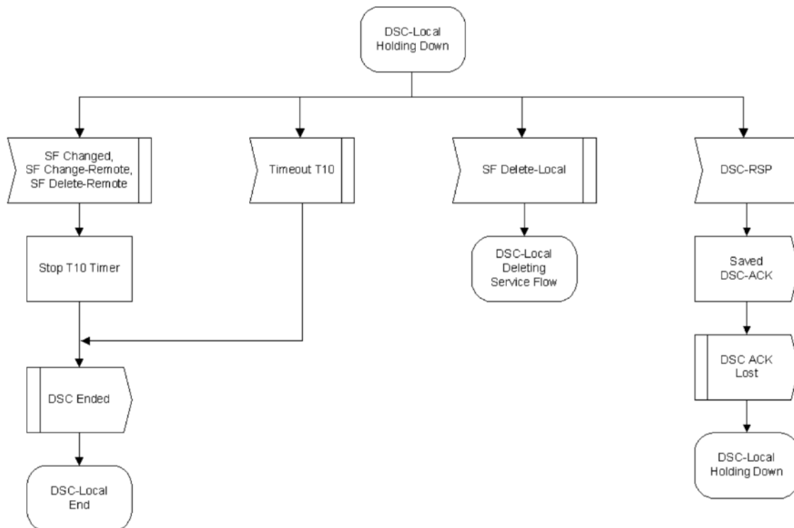
Figure 225 - DSC-Locally Initiated Transaction Holding Down State Flow Diagram
