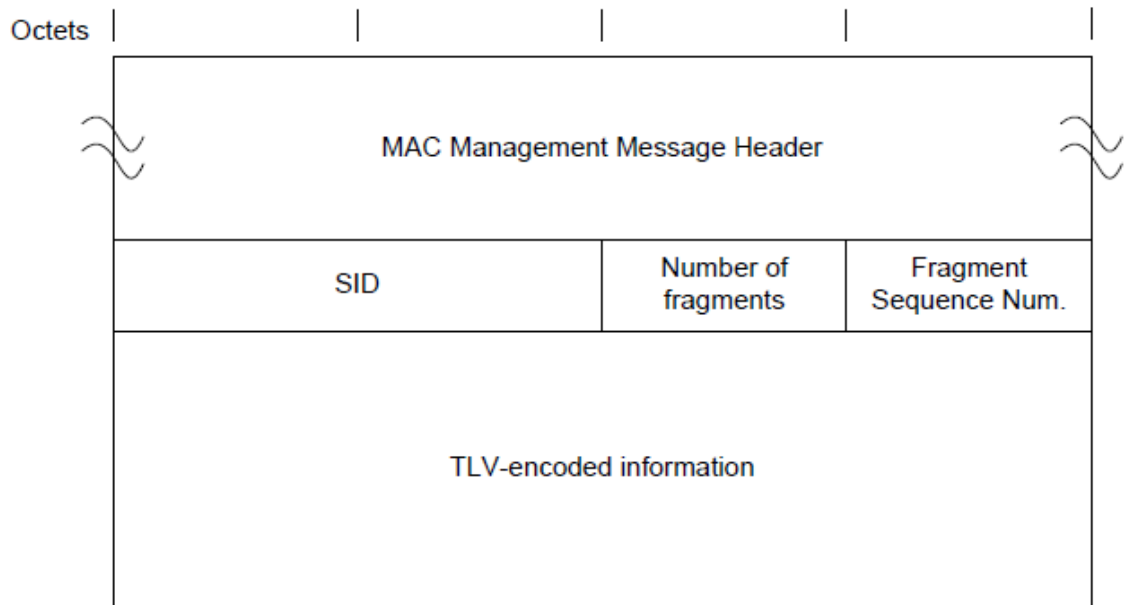
Figure 55 - Multipart Registration Request (REG-REQ-MP)
