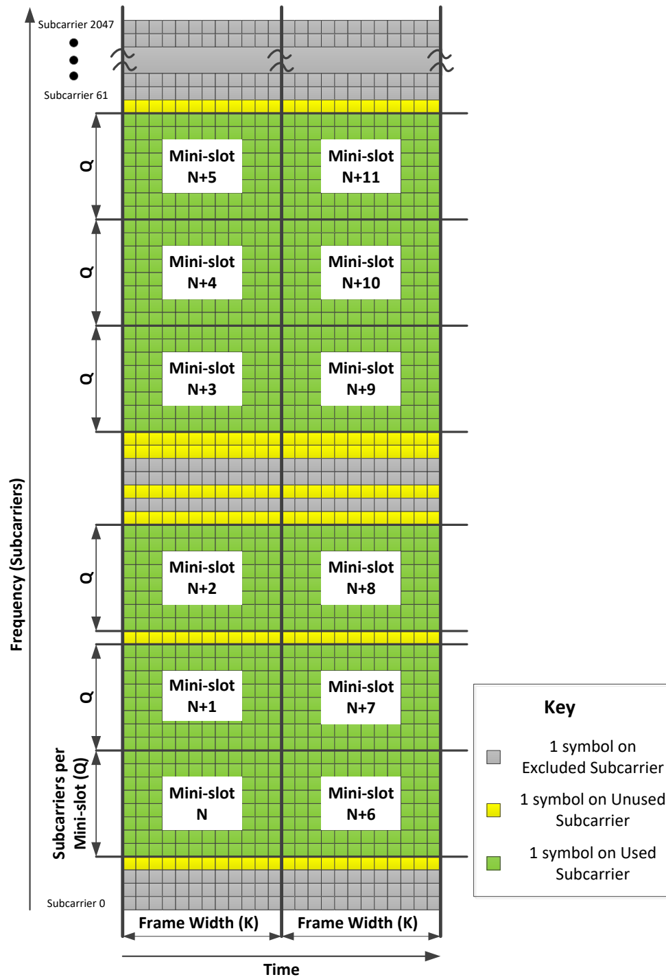
Figure 38 - Example Minislot Mapping for OFDMA
