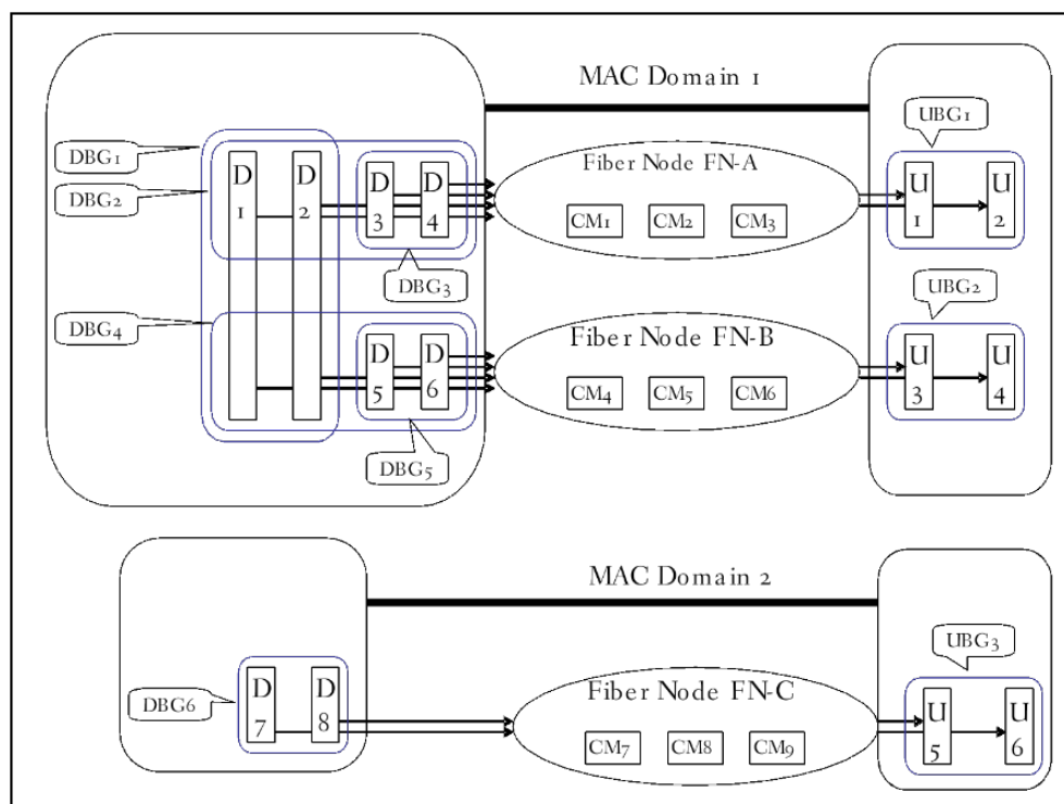
Figure 19 - Bonding Group Example
