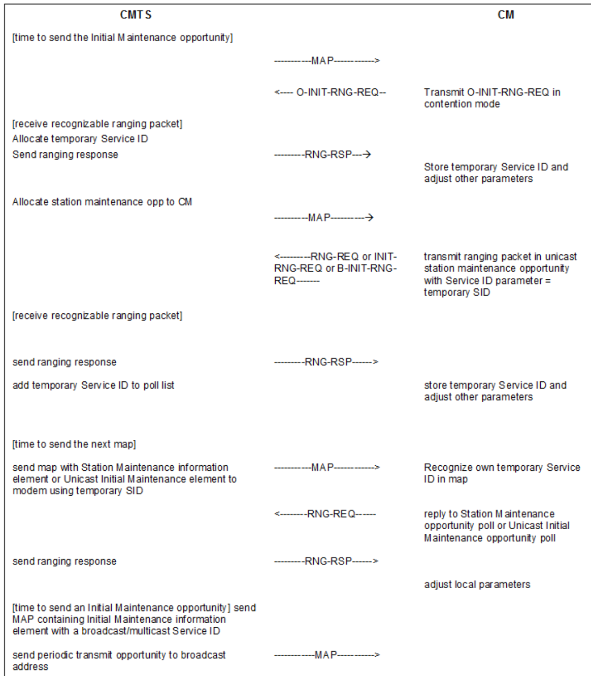
Figure 155 - Ranging and Automatic Adjustments Procedure for OFDMA Upstreams
