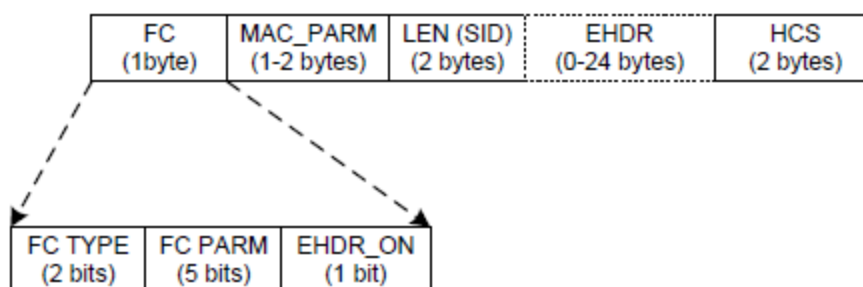
Figure 22 - MAC Header Format
