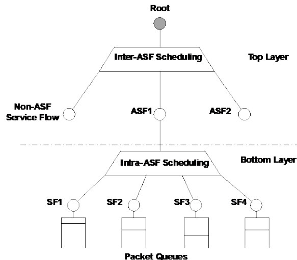
Figure 126 - Enhanced HQoS Scheduling Hierarchy
