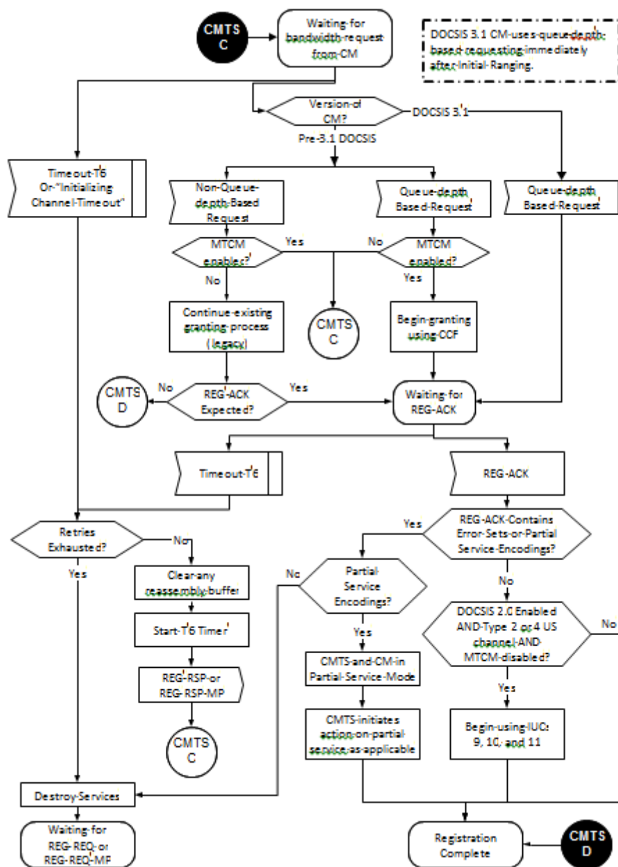
Figure 177 - CMTS Registration - End
