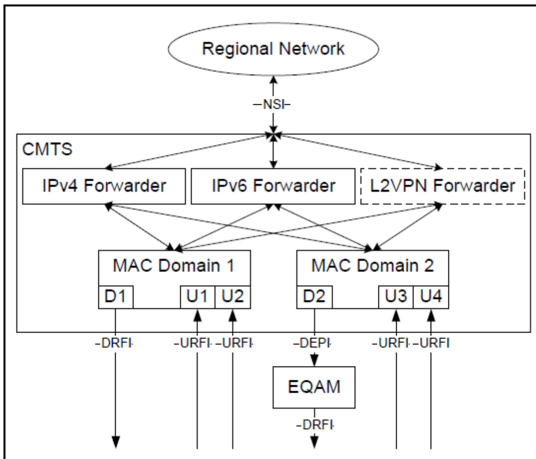
Figure 9 - CMTS Internal Forwarding Model
