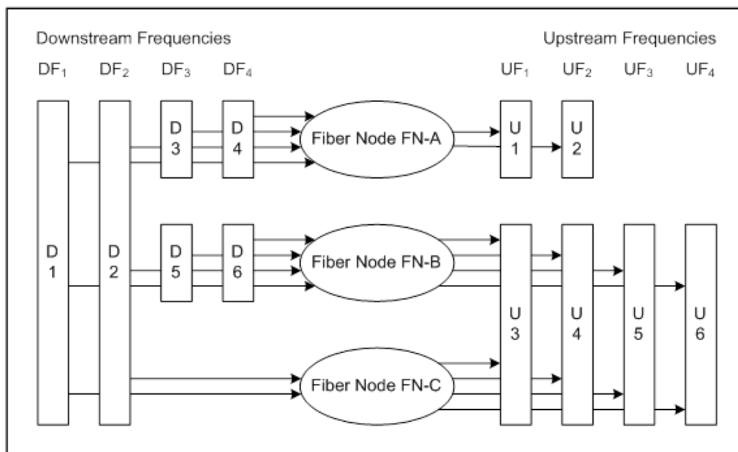
Figure 15 - Frequency Space Diagram
