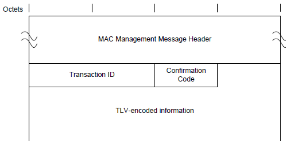
Figure 64 - Dynamic Service Change - Acknowledge
