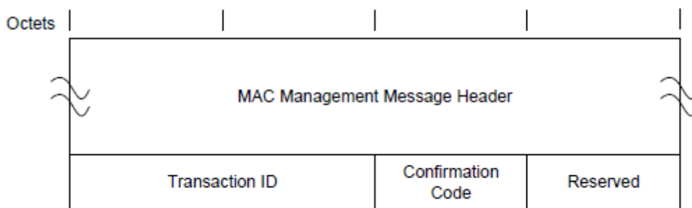
Figure 66 - Dynamic Service Deletion - Response
