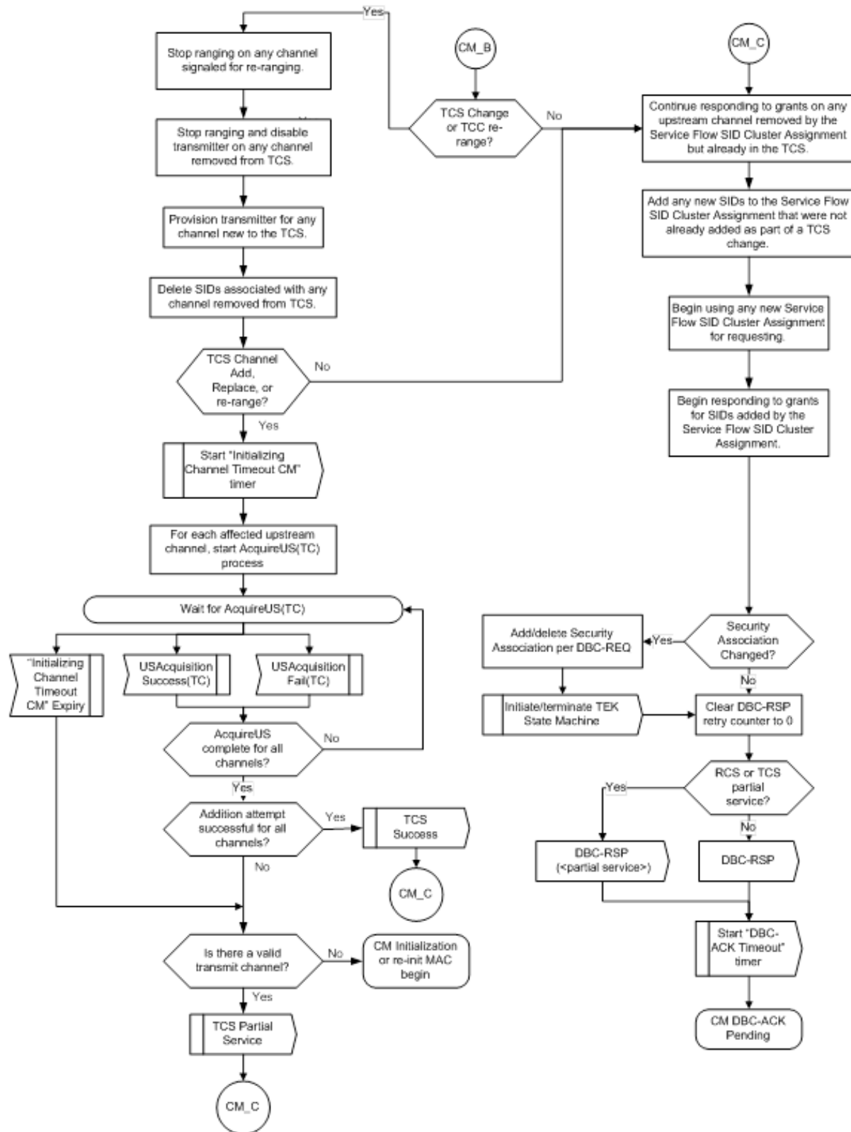
Figure 252 - CM DBC-RSP (part 3)
