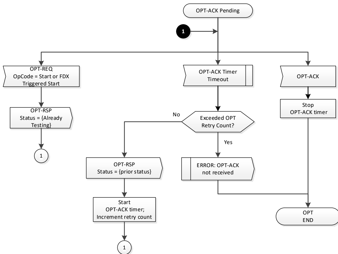
Figure 189 - CM OPT State Machine – OPT-ACK Pending
