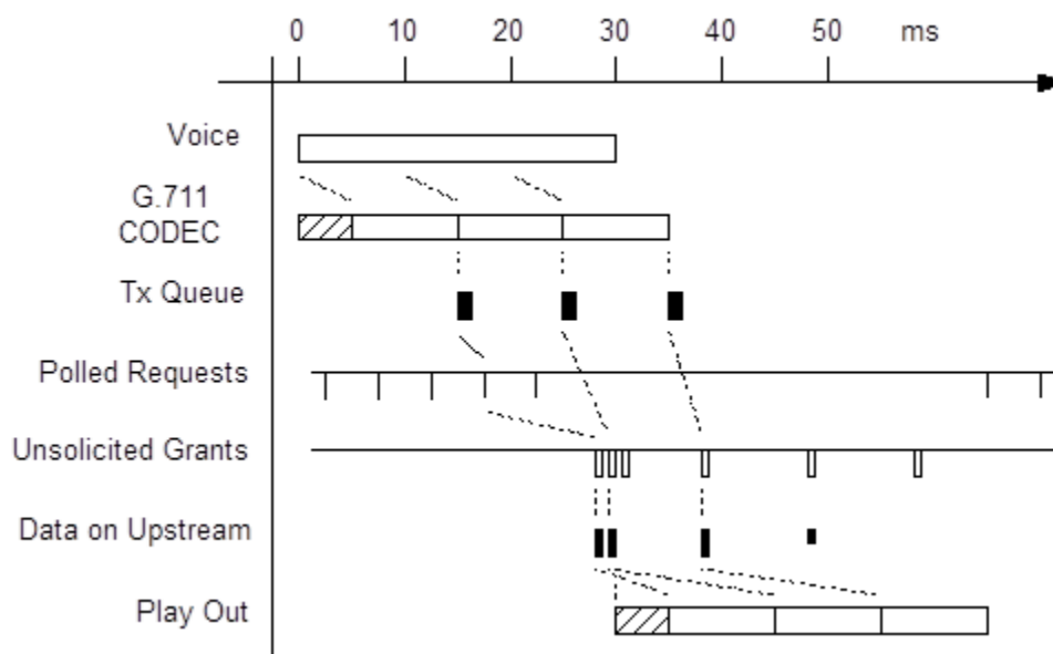
Figure 308 - VAD Start-Up and Stop
