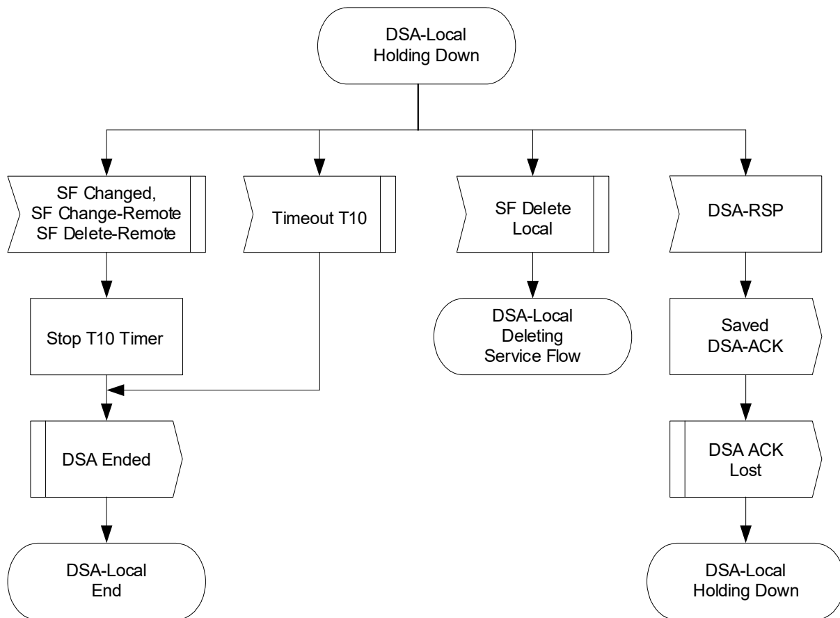
Figure 213 - DSA-Locally Initiated Transaction Holding State Flow Diagram
