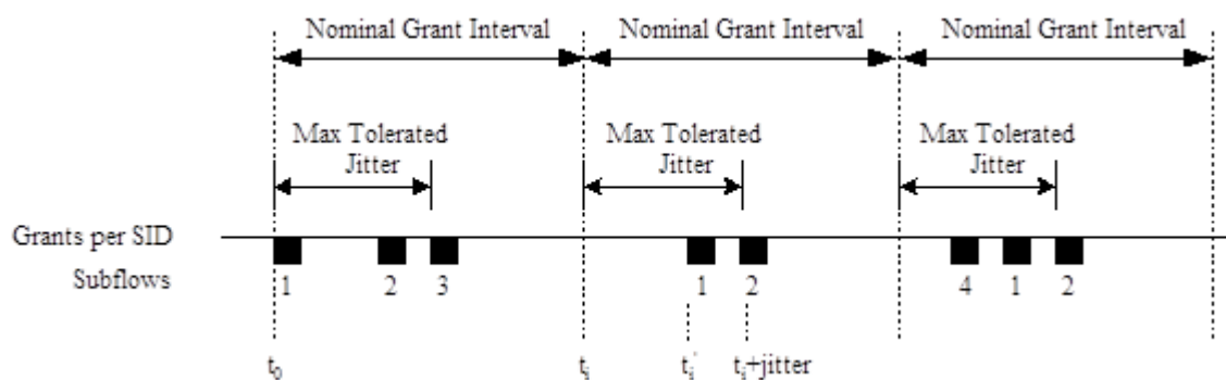
Figure 307 - Example Jitter with Multiple Grants per SID
