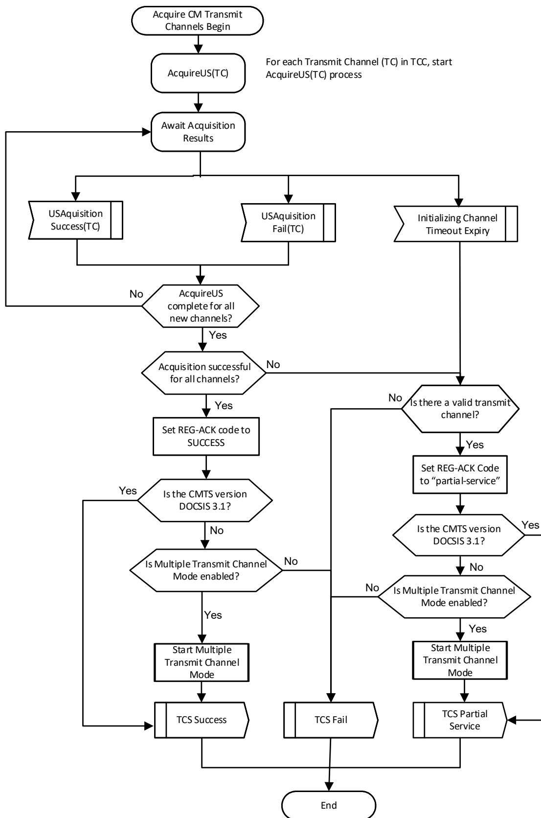
Figure 172 - CM Acquires Transmit Channels
