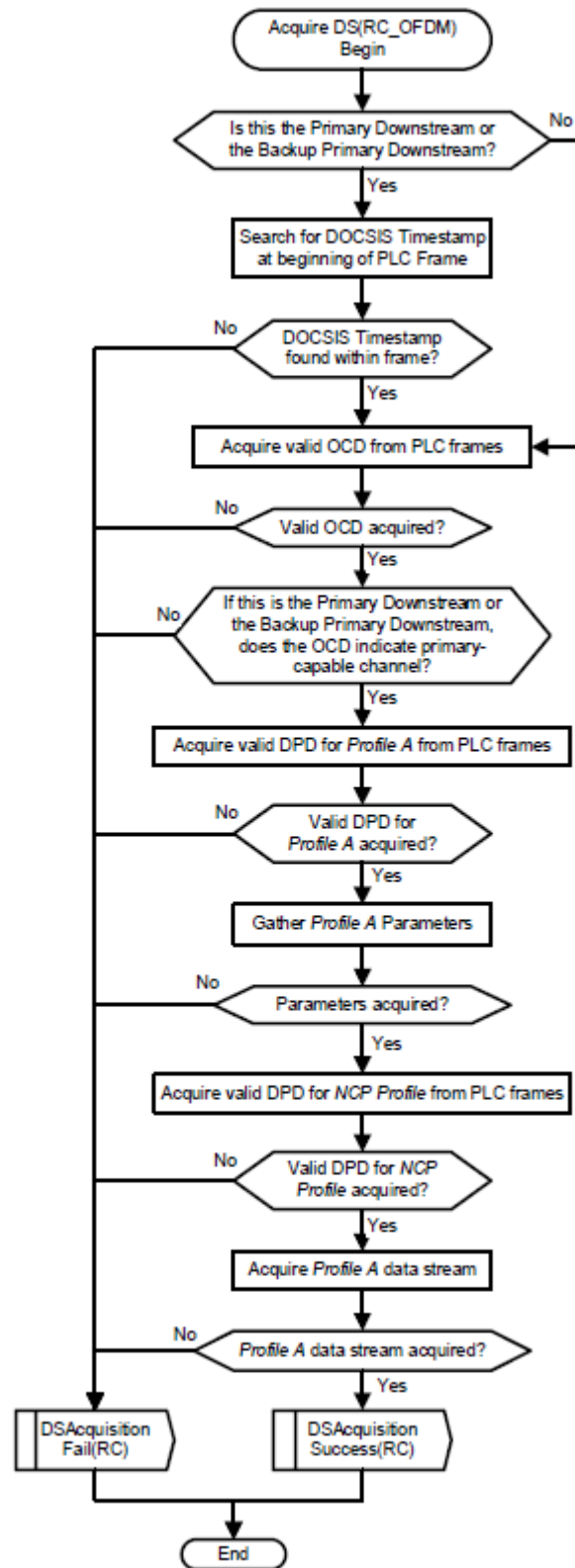
Figure 171 - CM Acquires OFDM Downstream Channel
