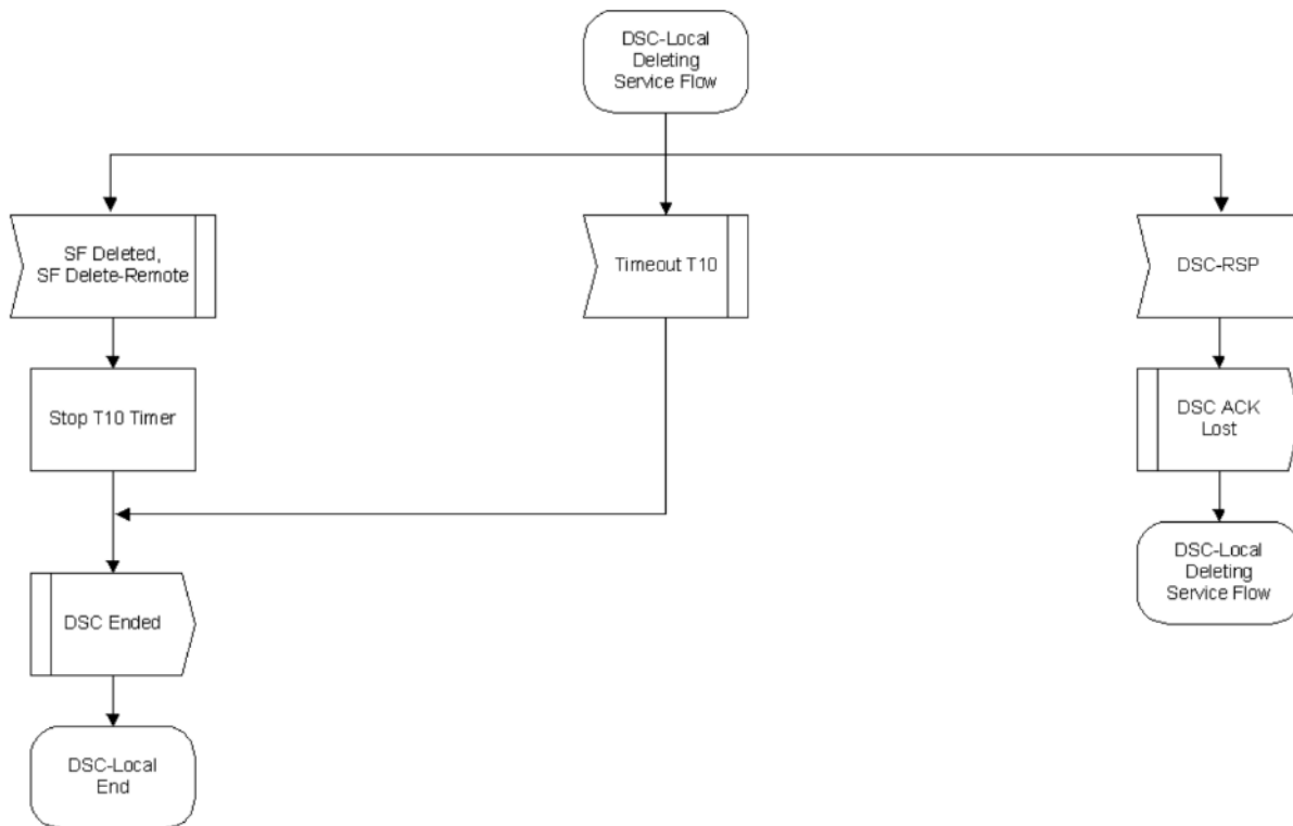
Figure 227 - DSC-Locally Initiated Transaction Deleting Service Flow State Flow Diagram
