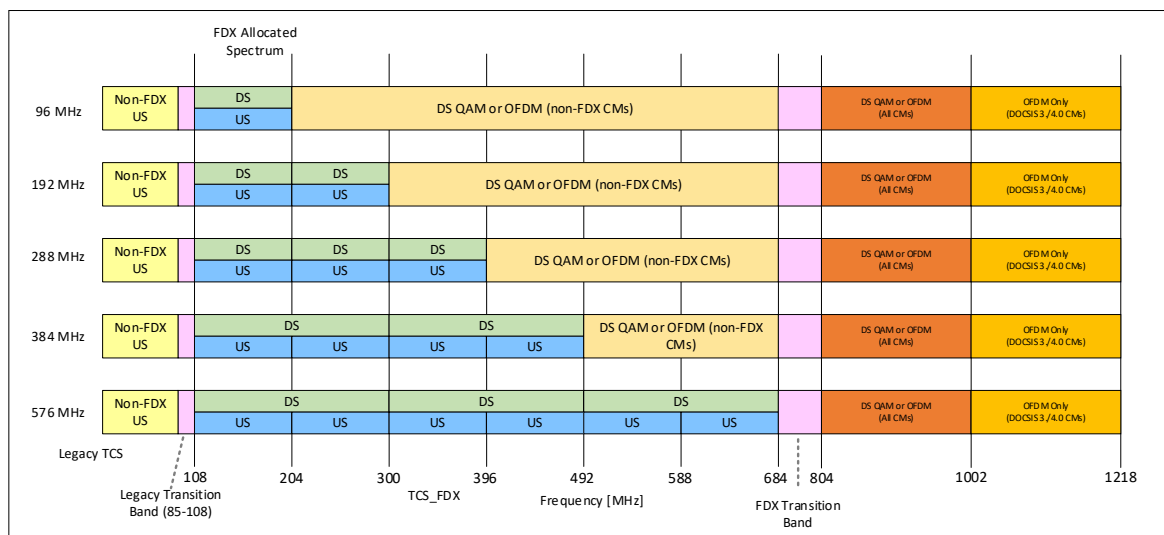
Figure 264 - Configurable FDX Allocated Spectrum Bandwidths for CFDX Band Plan with 1218 MHz Downstream Upper Band Edge
