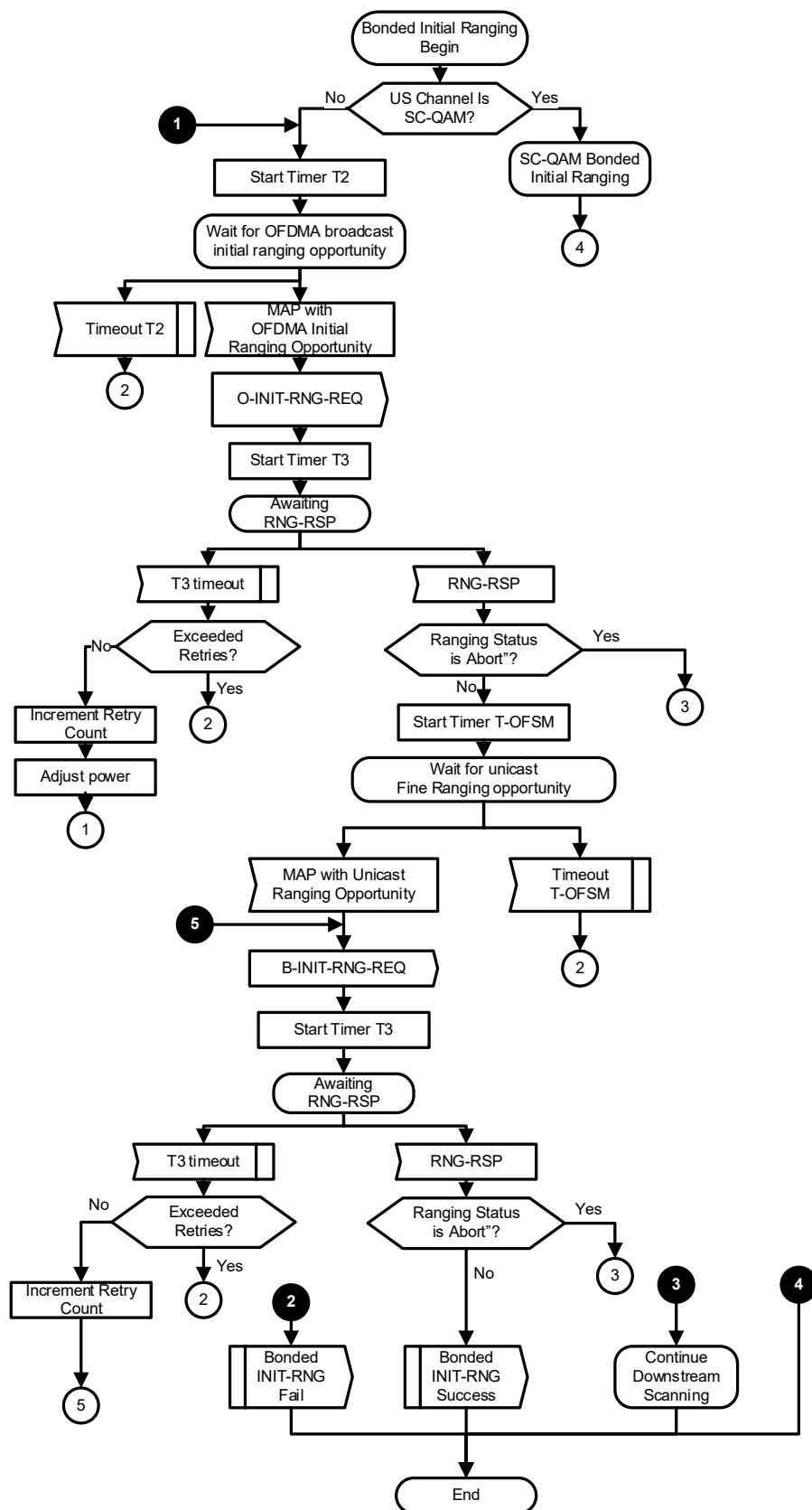
Figure 151 - Bonded Initial Ranging
