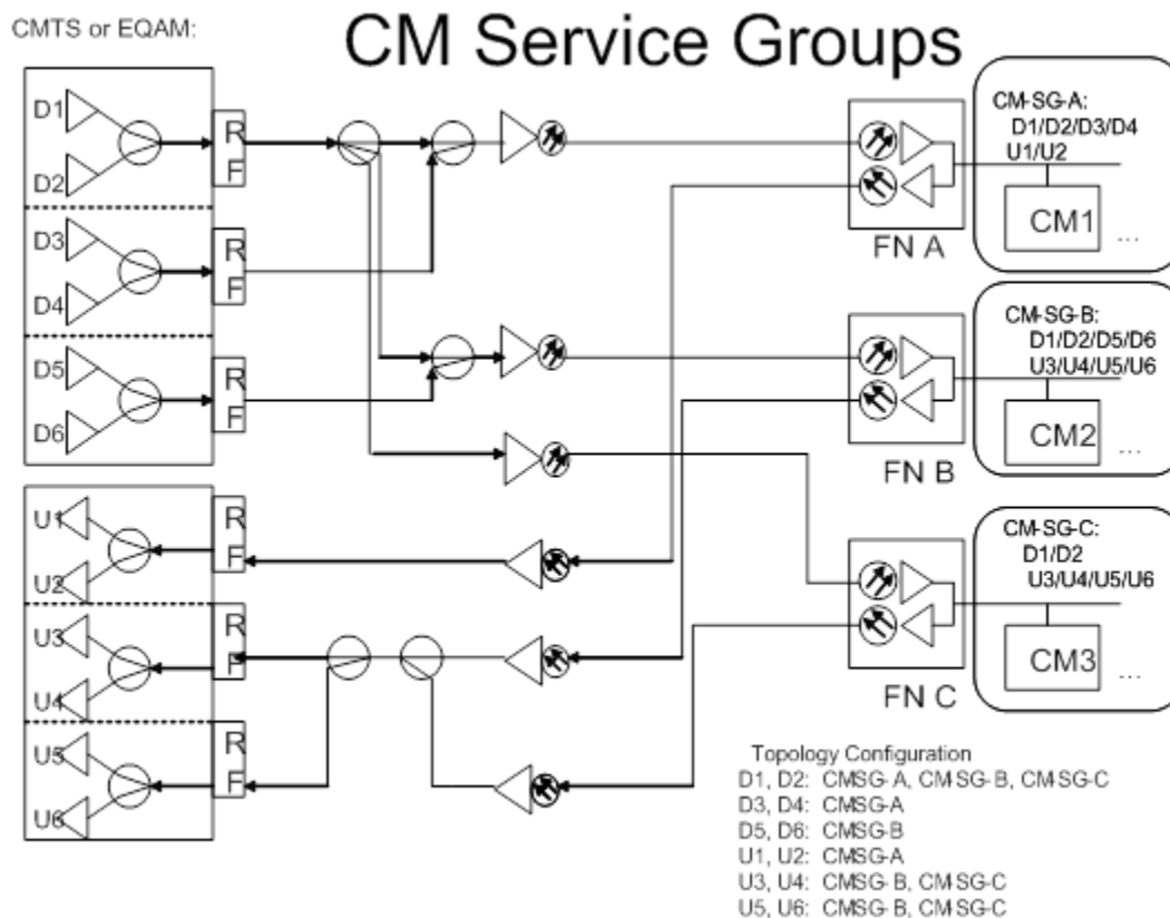
Figure 14 - CM Topology Configuration Example
