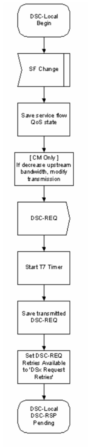
Figure 223 - DSC-Locally Initiated Transaction Begin State Flow Diagram
