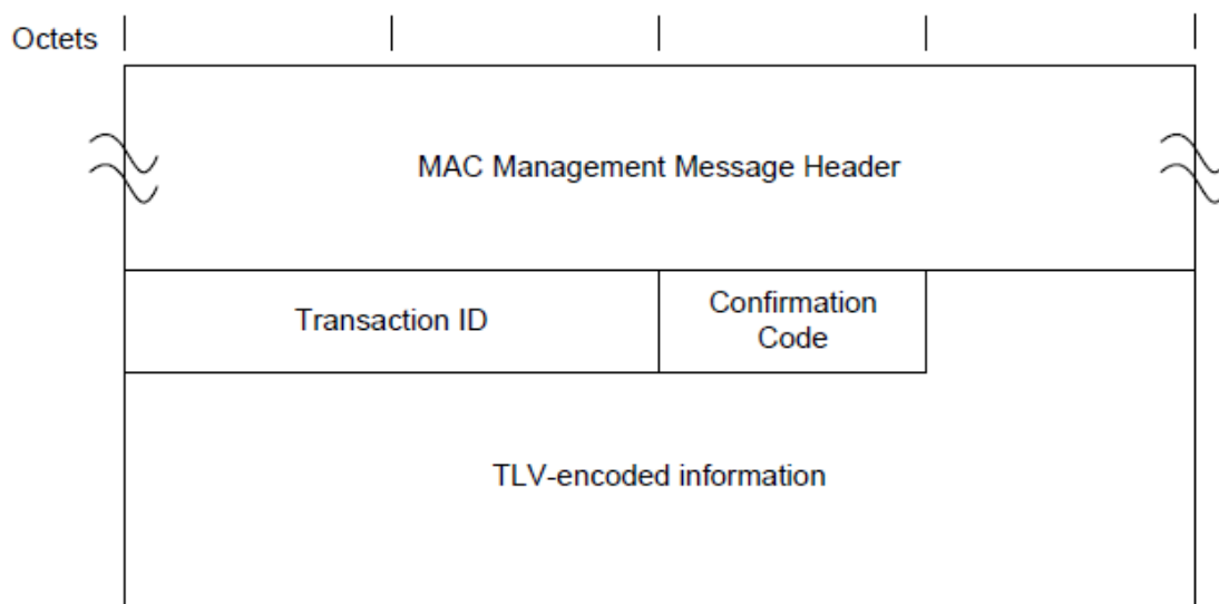
Figure 73 - Dynamic Bonding Change Response Message
