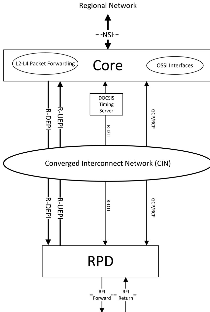
Figure 8 - MHA v2 Network Diagram
