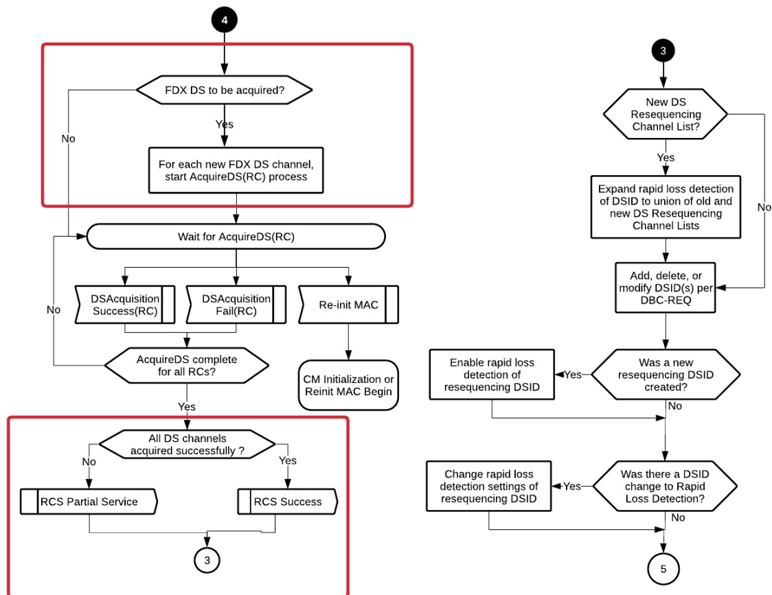
Figure 249 - CM DBC-RSP (part 1b)
