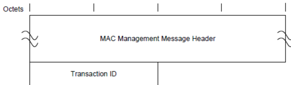
Figure 92 - DTP Acknowledge Message
