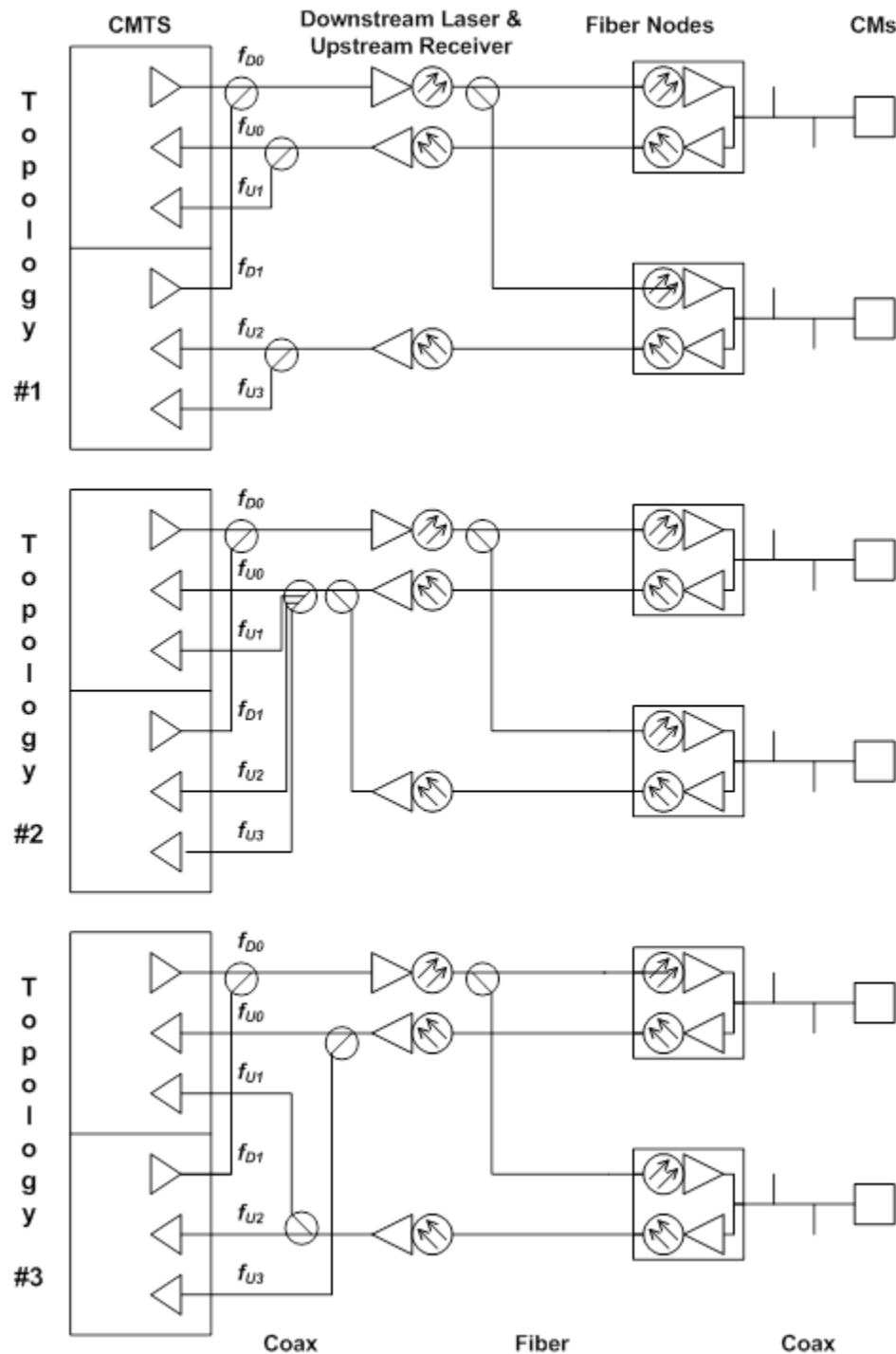
Figure 304 - Bonding Group Example
