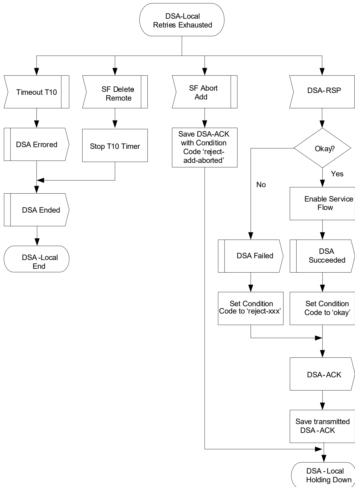
Figure 214 - DSA-Locally Initiated Transaction Retries Exhausted State Flow Diagram
