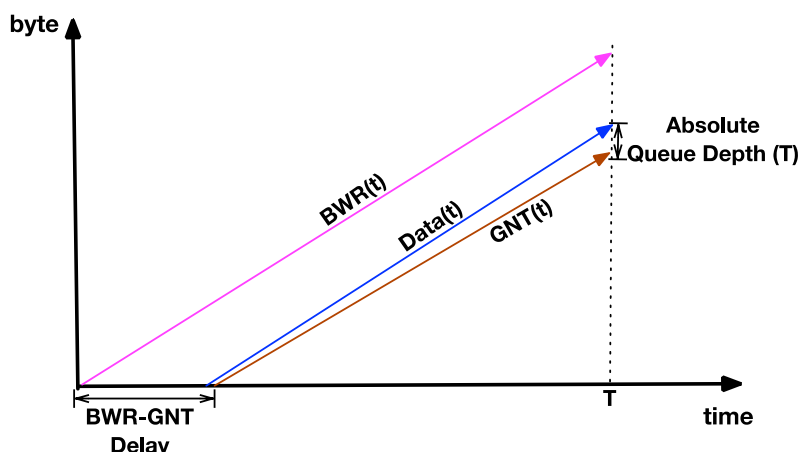
Figure 109 - Relationship between AQD, Data Traffic and BWR Triggered Grants in LLX
