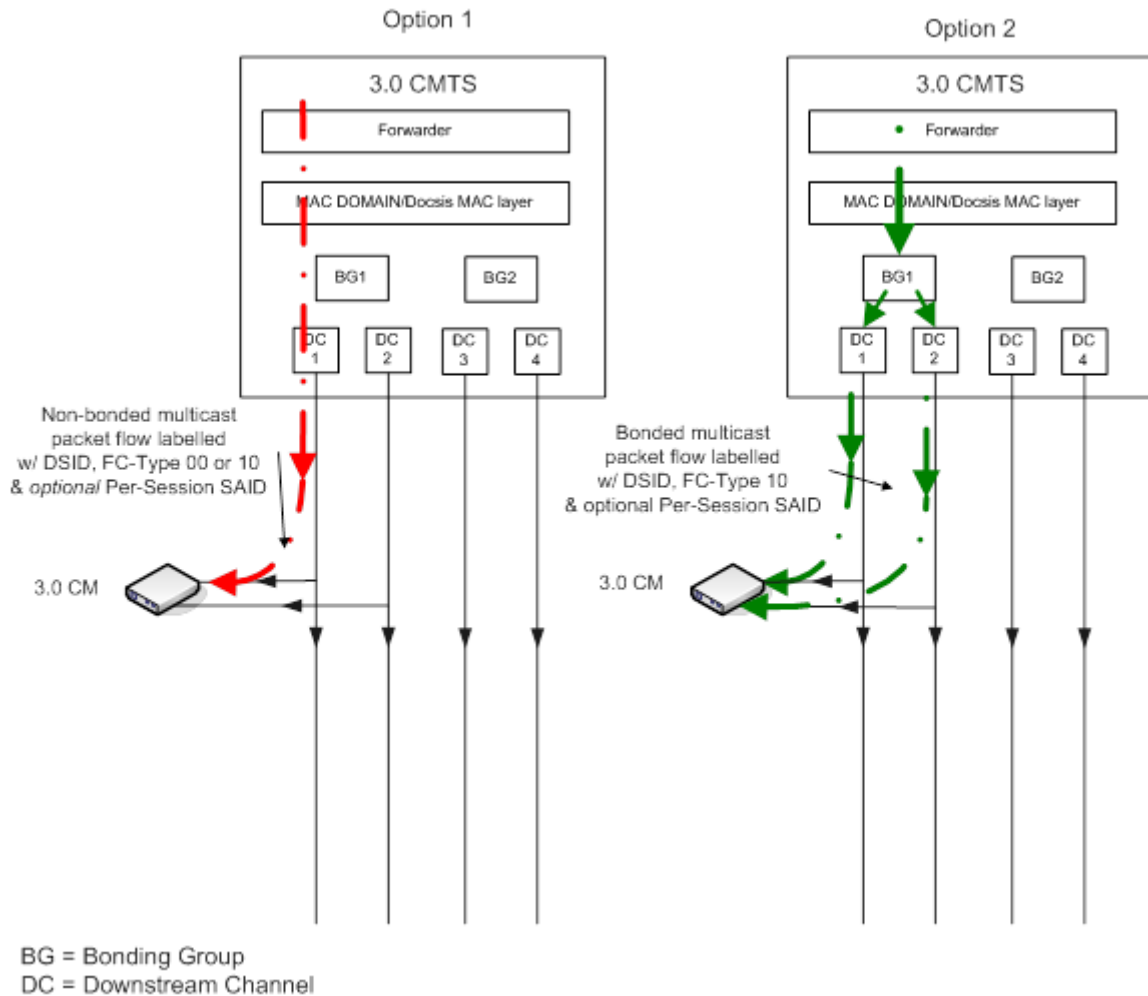
Figure 314 - Multicast Session Replication for a client behind a 3.0 CM
