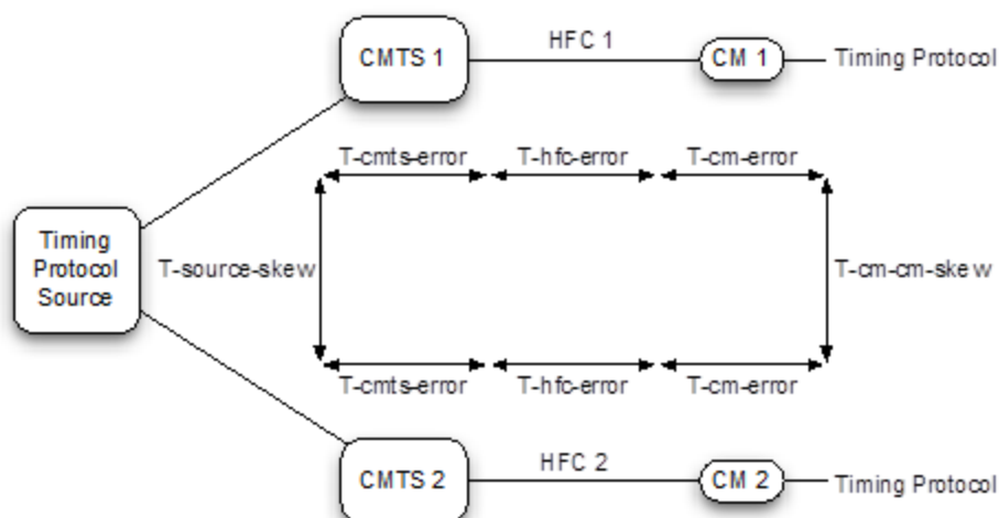
Figure 200 - DTP System Performance
