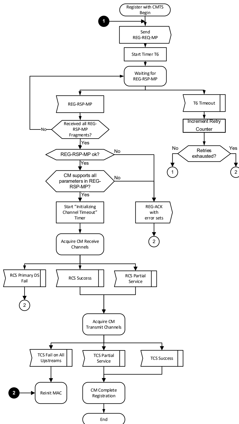
Figure 168 - CM Register with CMTS - Begin
