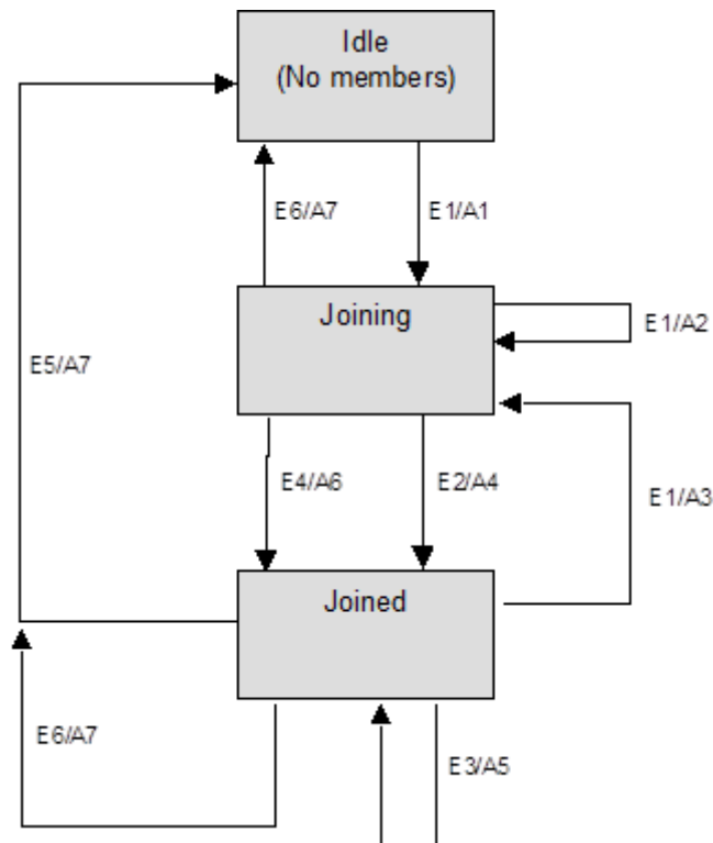
Figure 320 - IGMP Support - CM Passive Mode
