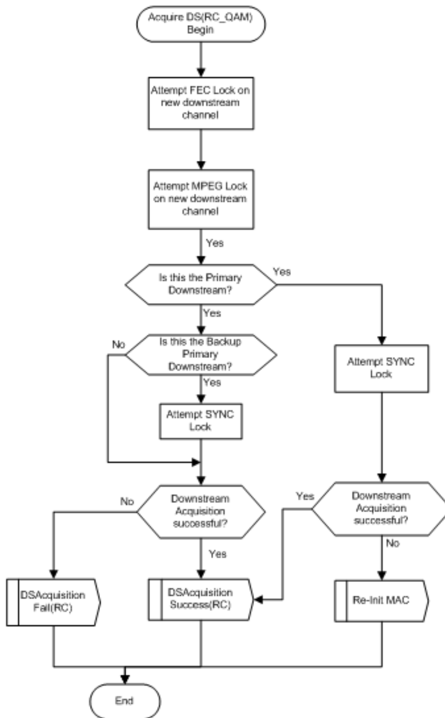
Figure 253 - CM AcquireDS Procedure for SC-QAM
