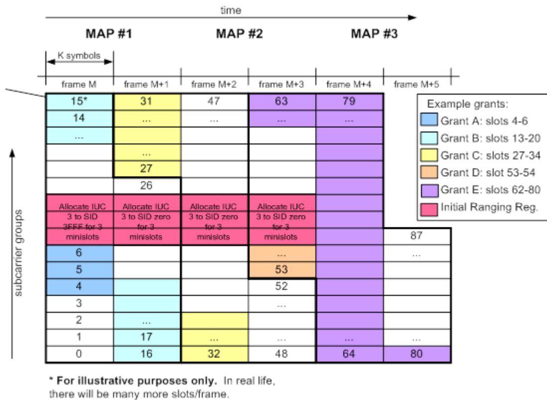
Figure 113 - Example Initial Ranging Region on an OFDMA Channel
