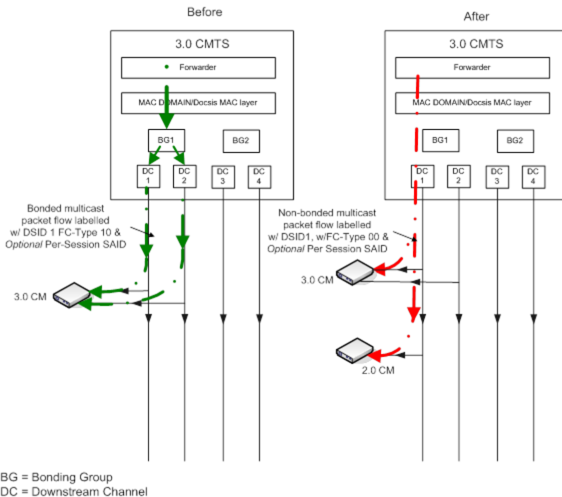
Figure 315 - Multicast Session Replication to Clients Behind Both a 3.0 CM and a 2.0 CM on the Same Downstream Channel (Subcase 1)
