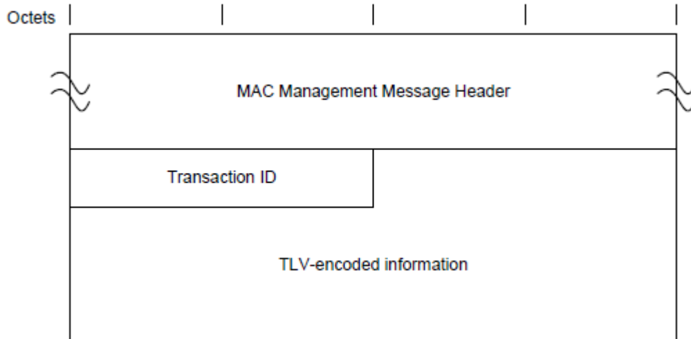
Figure 89 - DTP Request Message
