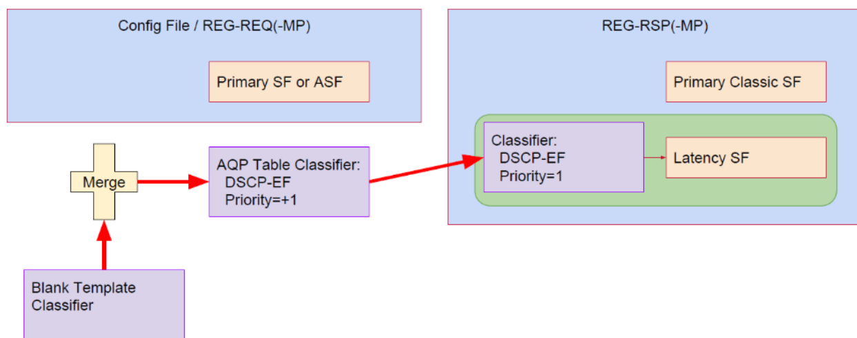
Figure 131 - Classifier Merge Example 1
