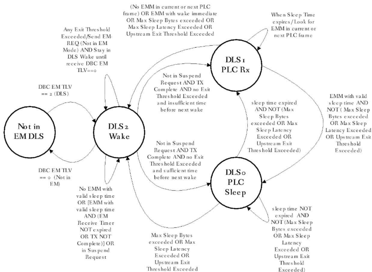
Figure 260 - CM DLS Substate Diagram
