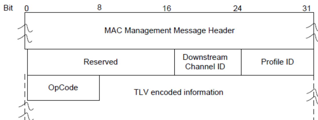
Figure 86 - The OFDM Downstream Profile Test Request (OPT-REQ) message
