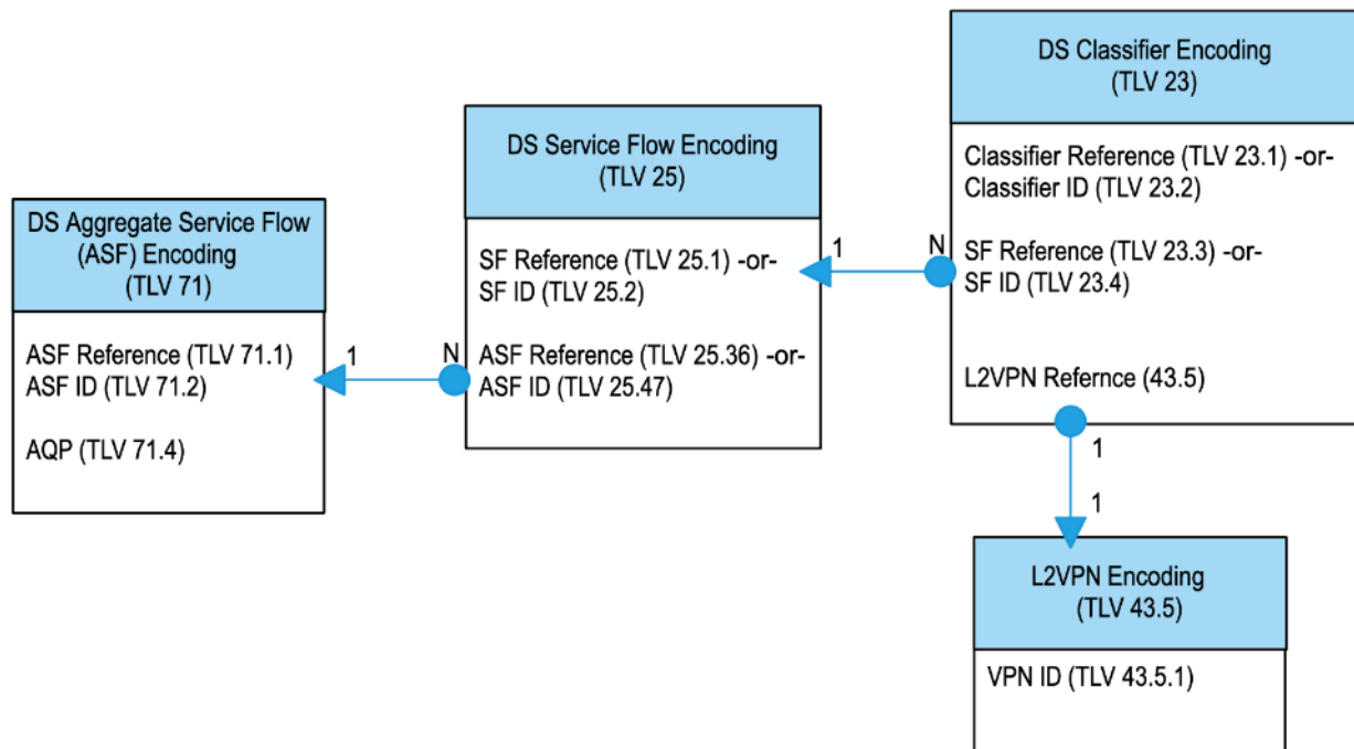
Figure 124 - Relationship of Downstream Classifiers, Service Flows, ASFs and L2VPN
