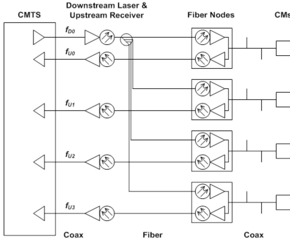
Figure 303 - Single Downstream and Single Upstream Channels per CM
