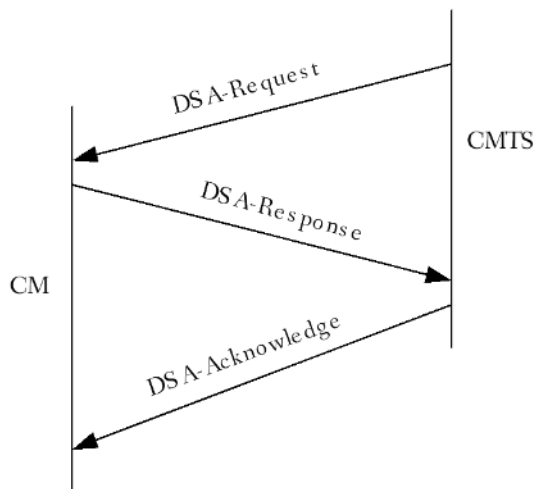
Figure 122 - Dynamic Service Addition Message Flow – CMTS Initiated
