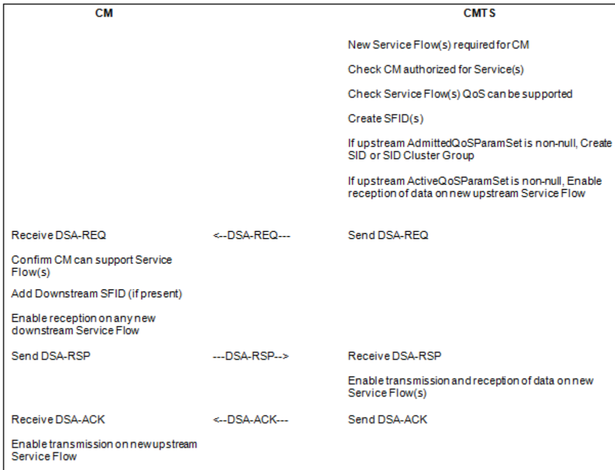
Figure 210 - Dynamic Service Addition Initiated from CMTS
