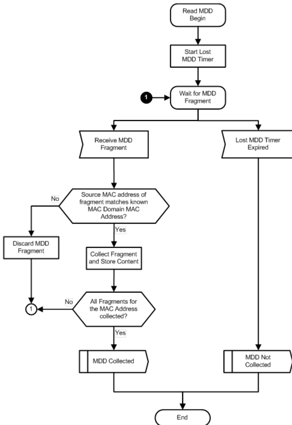
Figure 147 - Read MAC Domain Descriptor (MDD)
