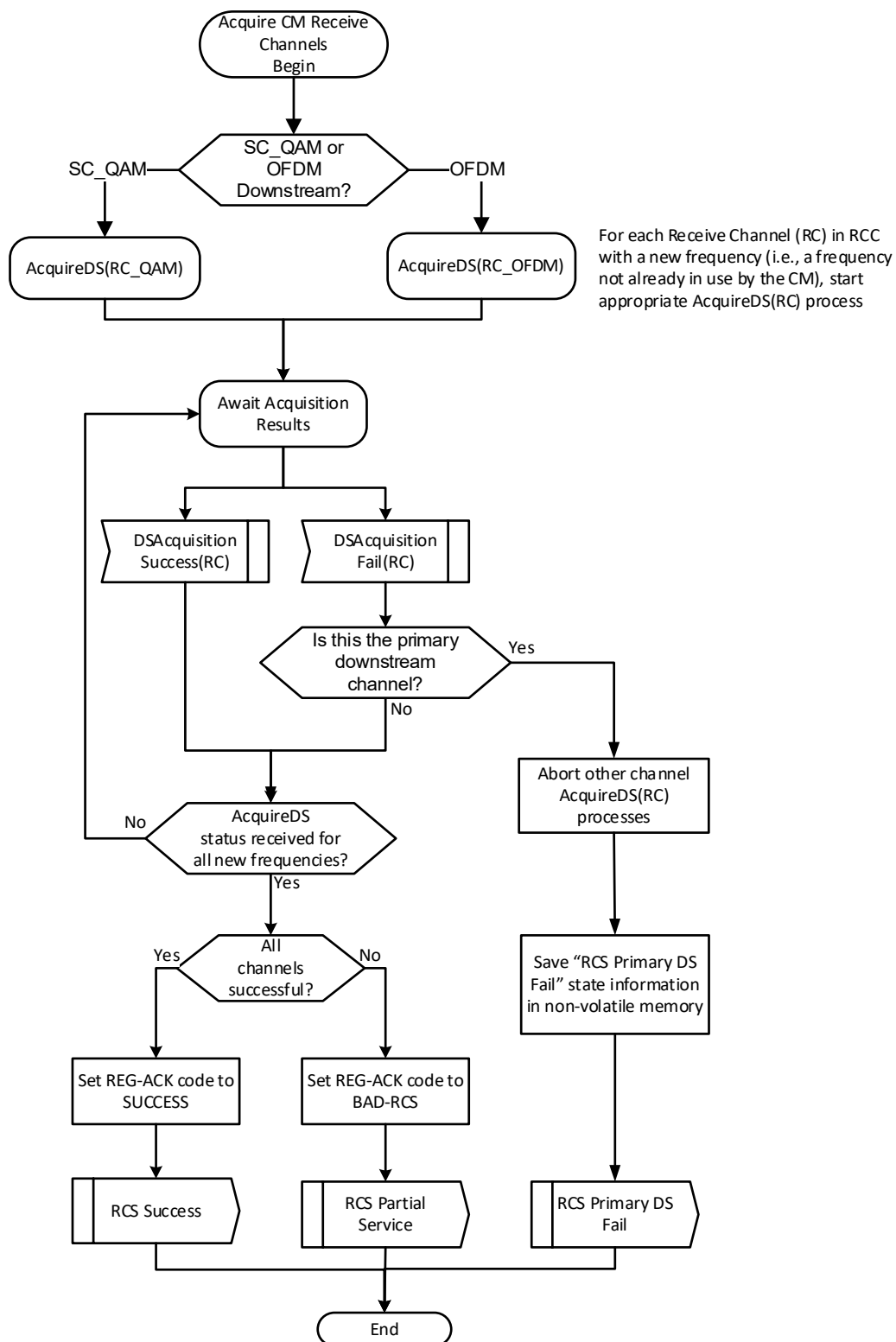
Figure 169 - CM Acquires Receive Channels
