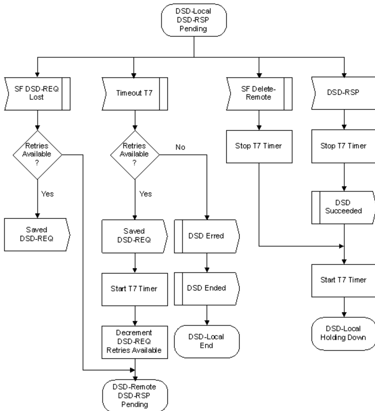
Figure 235 - DSD-Locally Initiated Transaction DSD-RSP Pending State Flow Diagram
