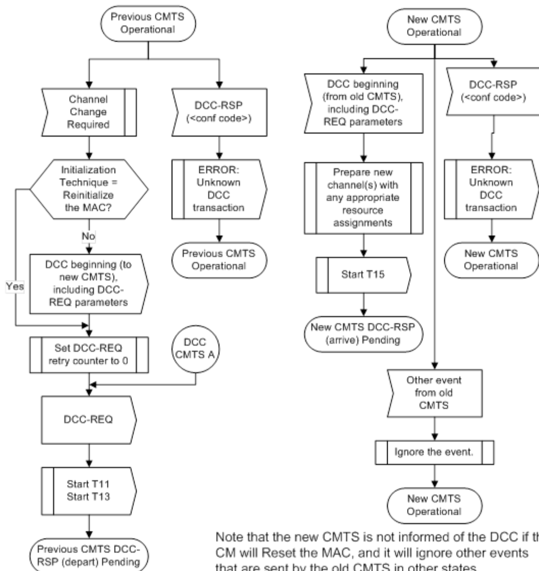
Figure 239 - Dynamically Changing Channels: CMTS View Part 1
