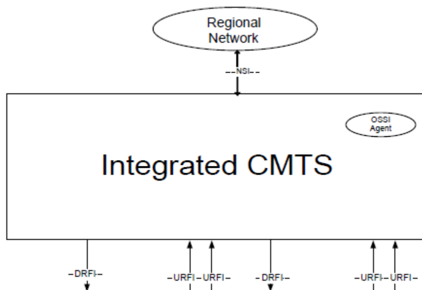
Figure 6 - Integrated CMTS Network Diagram (Legacy)
