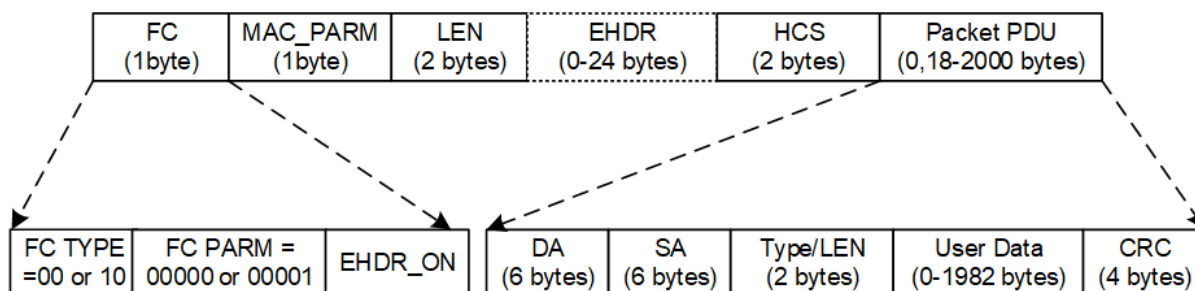
Figure 23 - Packet PDU or Isolation Packet PDU MAC Frame Format (IEEE 802.3)
