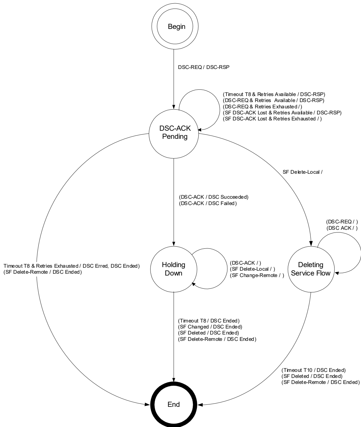
Figure 206 - DSC-Remotely Initiated Transaction State Transition Diagram
