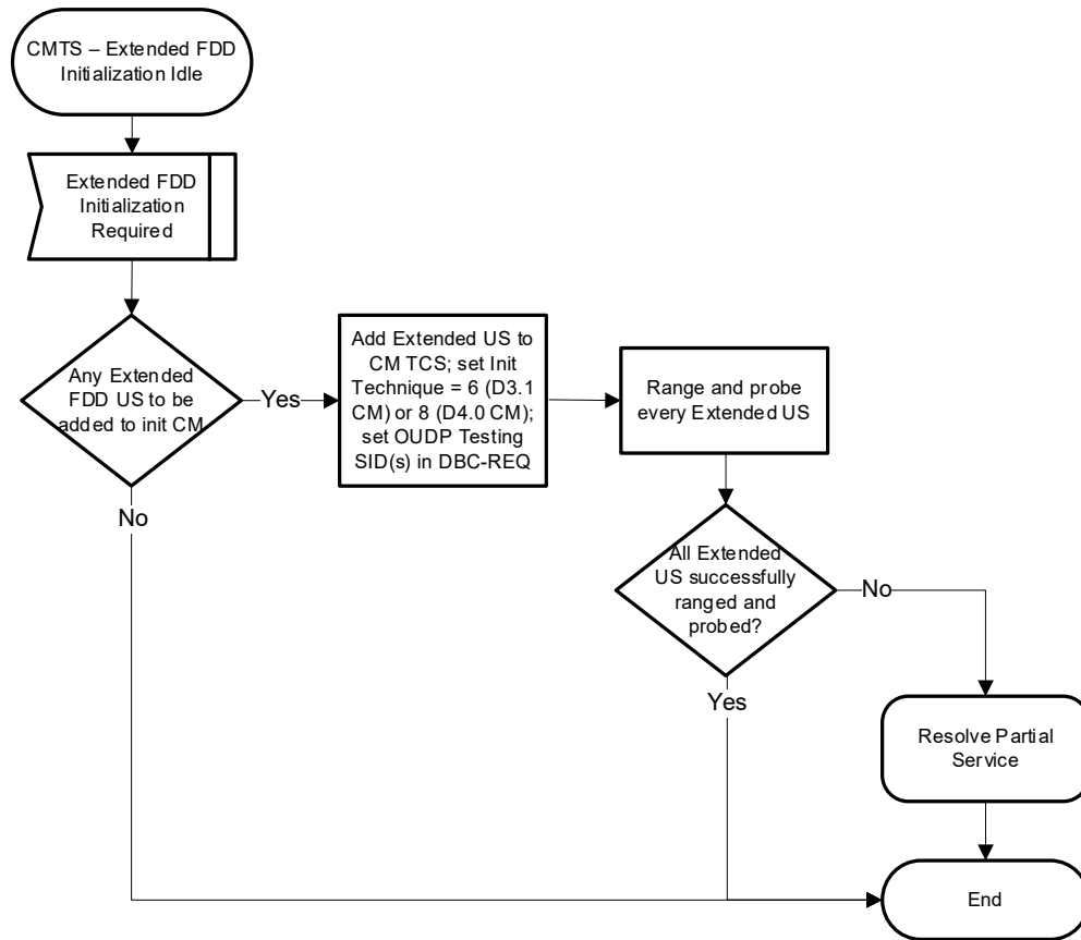
Figure 293 - CMTS Perspective on Adding FDD Extended Upstream Channels
