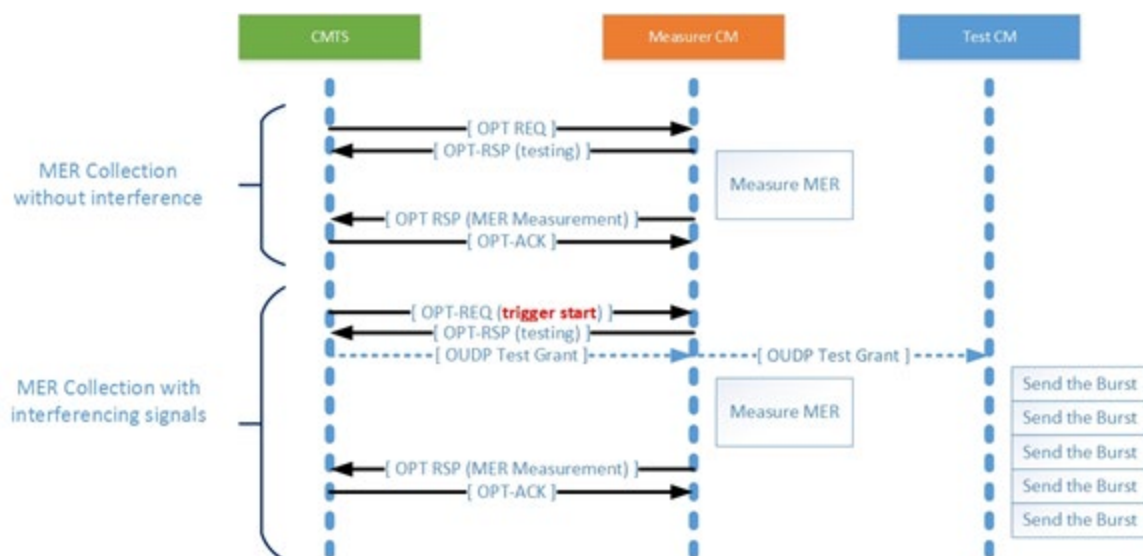
Figure 278 - IG Discovery Message Flow (OUDP)
