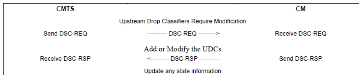
Figure 222 - CMTS-Initiated DSC Modifying an Upstream Drop Classifier
