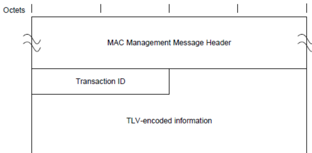
Figure 59 - Dynamic Service Addition - Request
