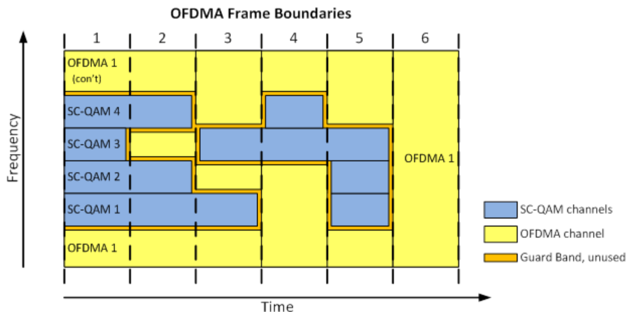
Figure 12 - Upstream Time and Frequency Multiplexing
