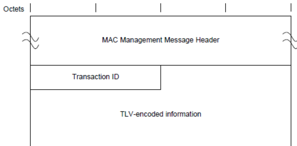
Figure 62 - Dynamic Service Change - Request
