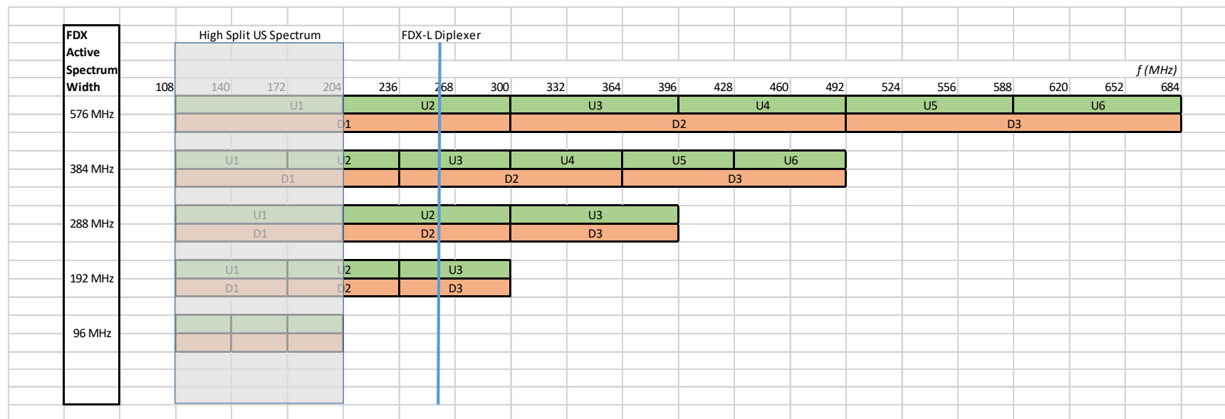
Figure 328 - FDX Grid Width Options
