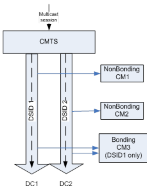
Figure 140 - DSIDs Prevent Duplication of Non-Bonded Replications
