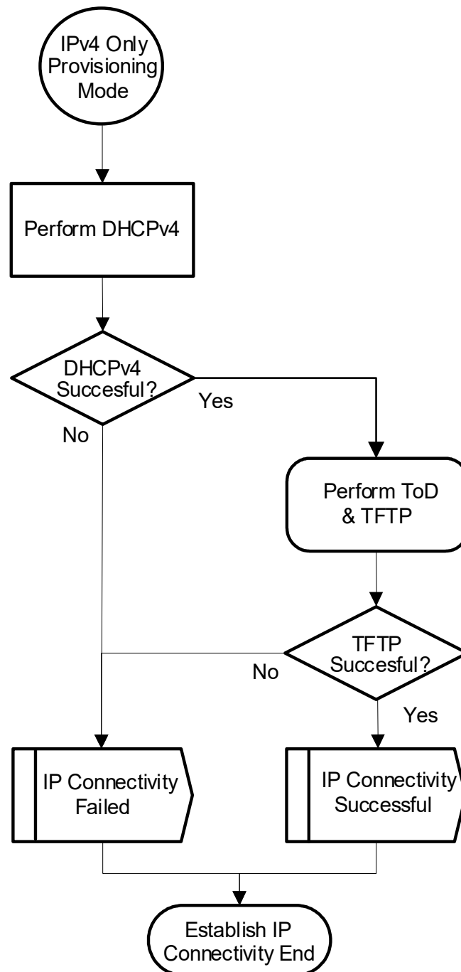
Figure 160 - IPv4 Only Provisioning Mode
