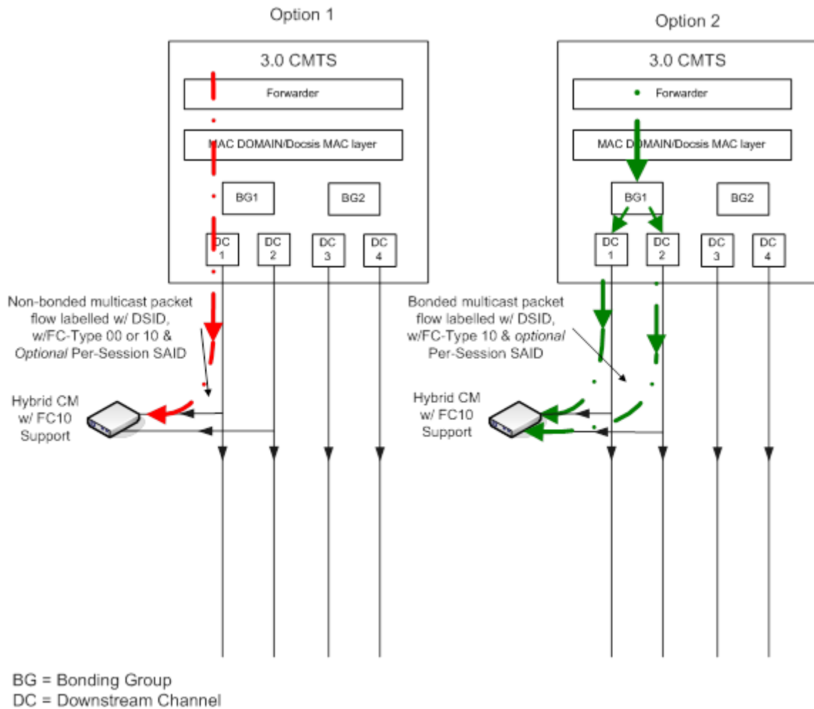
Figure 313 - Multicast Session Replication for a client behind a Hybrid CM capable of FC-Type 10
