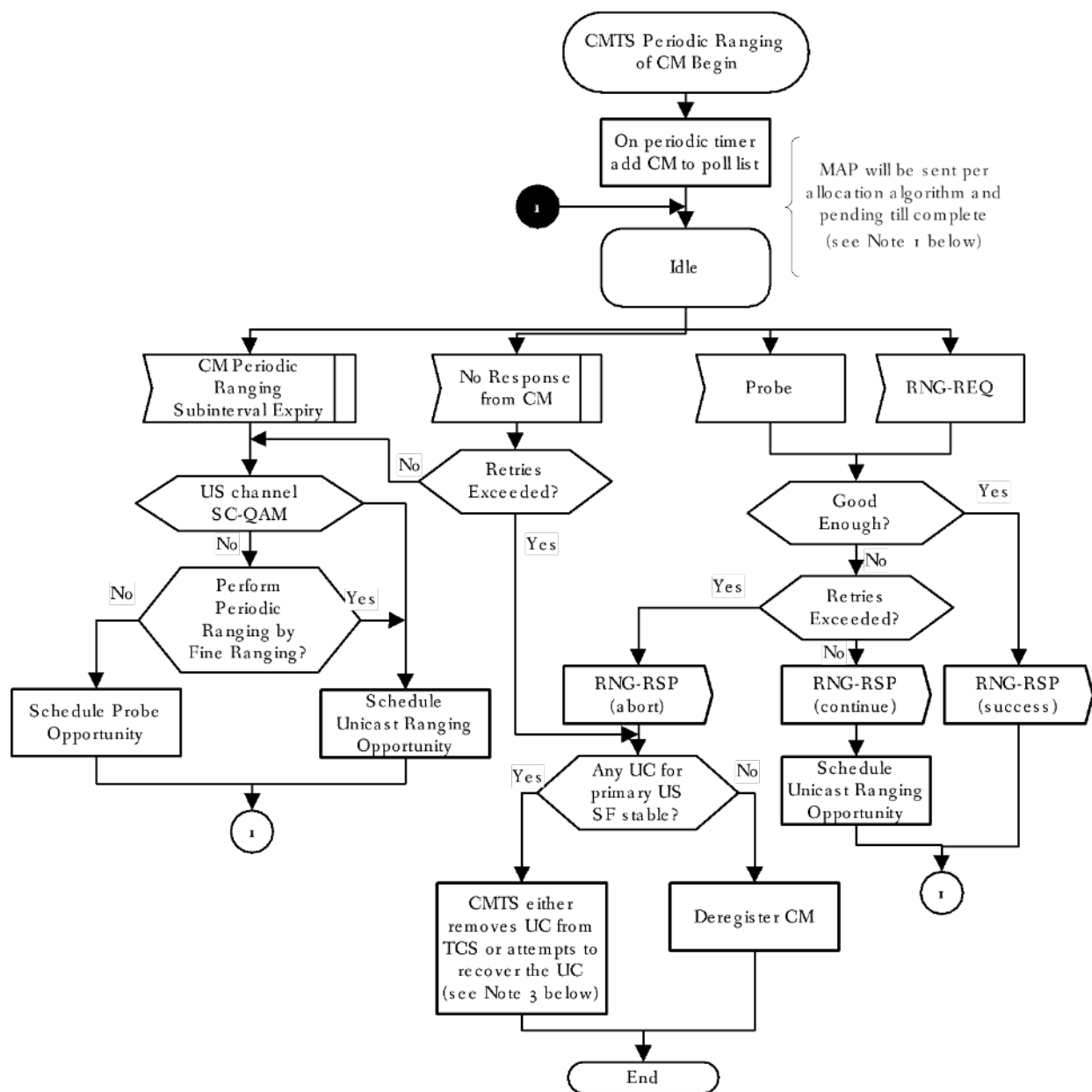
Figure 178 - Periodic Ranging – CMTS View
