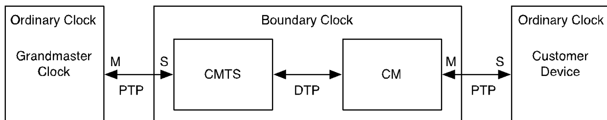
Figure 195 - DTP/PTP Reference Architecture
