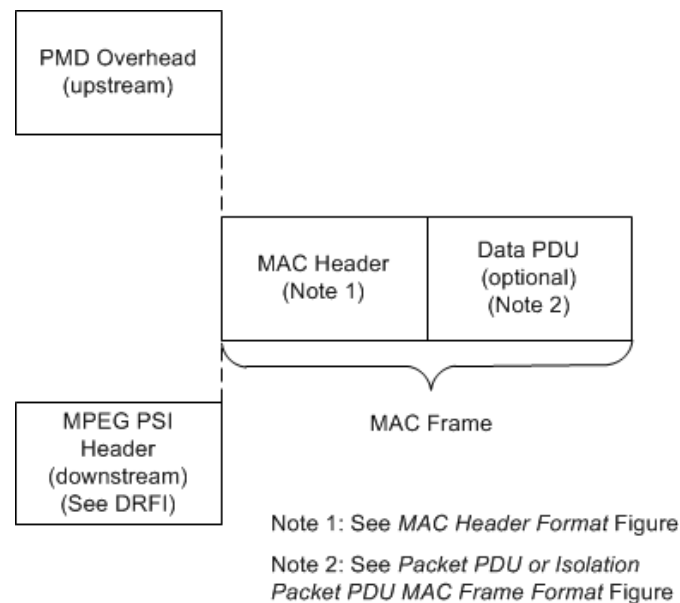
Figure 21 - Generic MAC Frame Format
