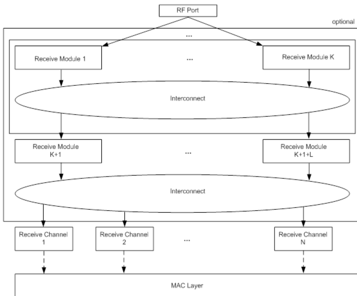
Figure 136 - Interconnection between Receive Channels and Receive Modules
