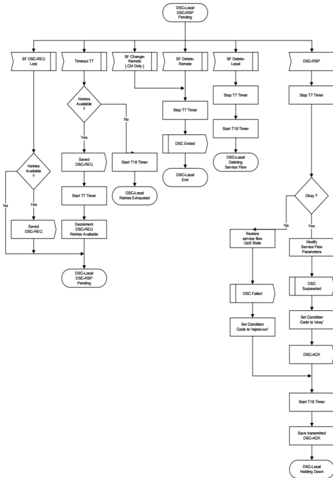
Figure 224 - DSC-Locally Initiated Transaction DSC-RSP Pending State Flow Diagram
