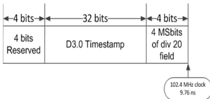
Figure 35 - OFDMA Timestamp Snapshot Sub-TLV Relationship to the Extended Timestamp
