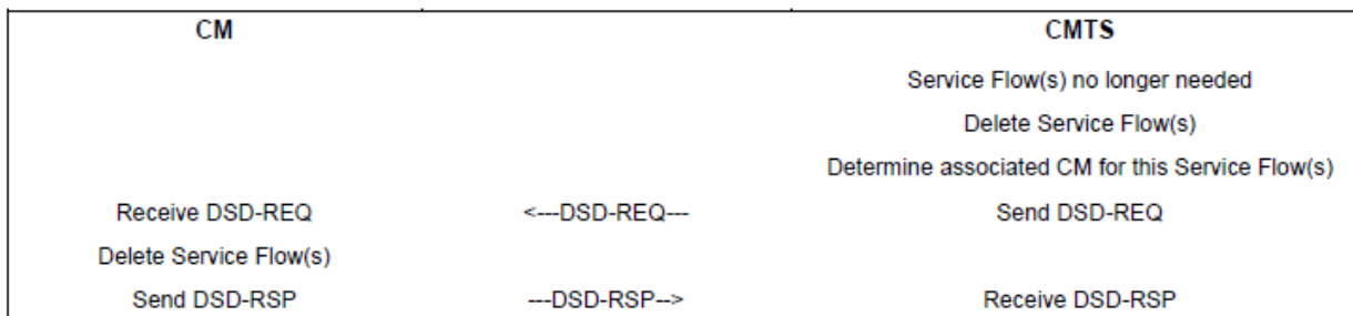
Figure 233 - Dynamic Service Deletion Initiated from CMTS
