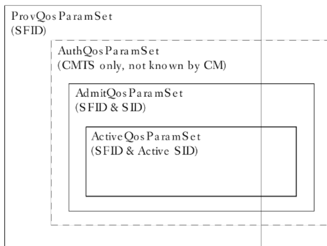
Figure 117 - Dynamic Authorization Model Envelopes
