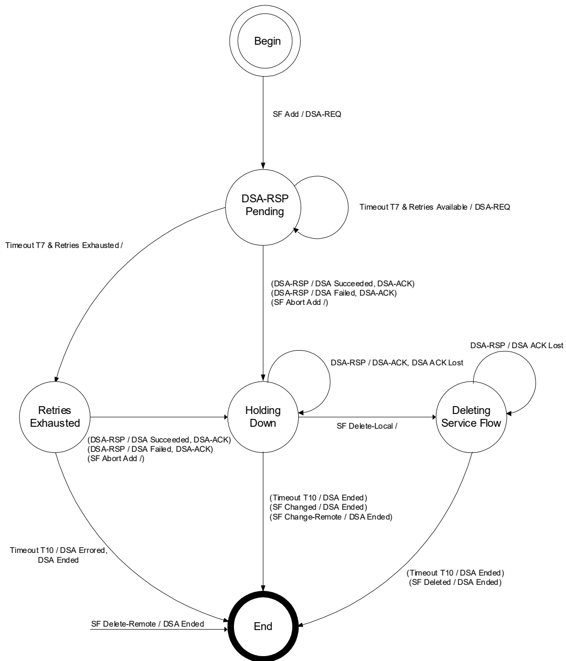
Figure 203 - DSA-Locally Initiated Transaction State Transition Diagram
