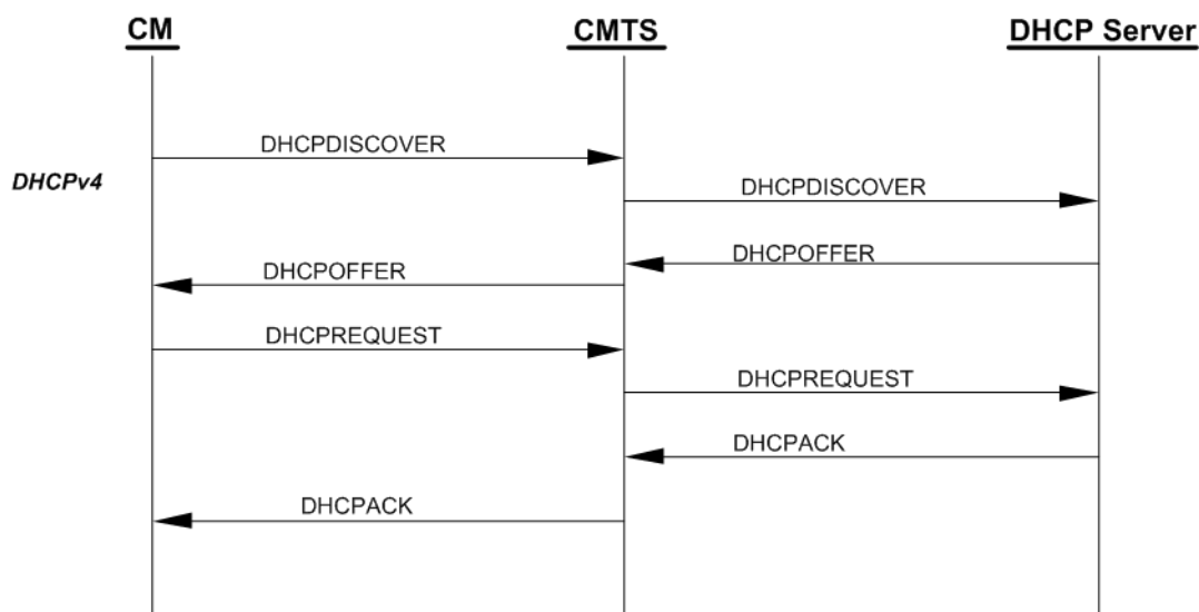
Figure 166 - IPv4 Provisioning Message Flow
