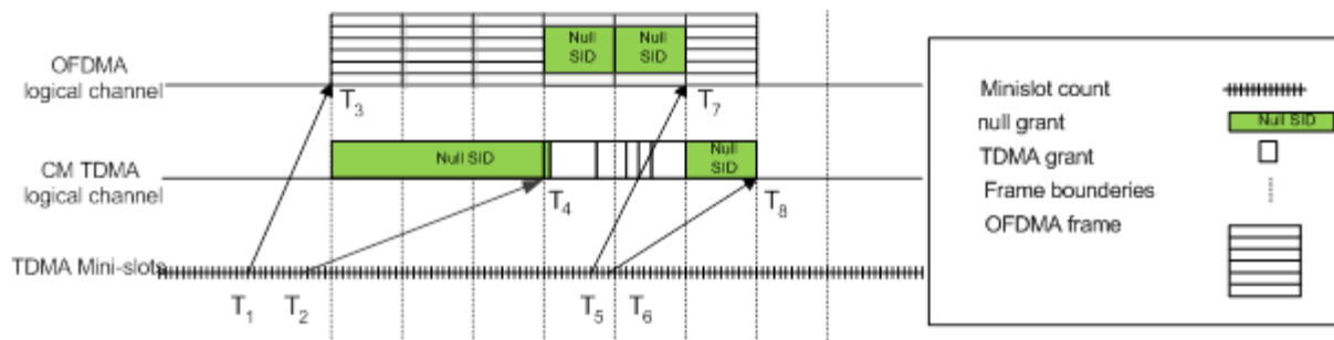
Figure 112 - Logical OFDMA and TDMA Channels
