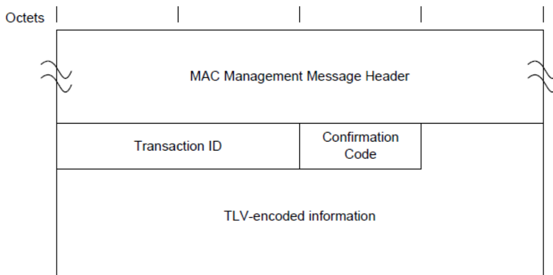
Figure 68 - Dynamic Channel Change Response
