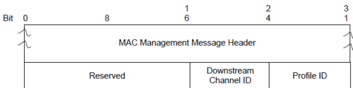
Figure 88 - The OFDM Profile Test Acknowledge (OPT-ACK) message
