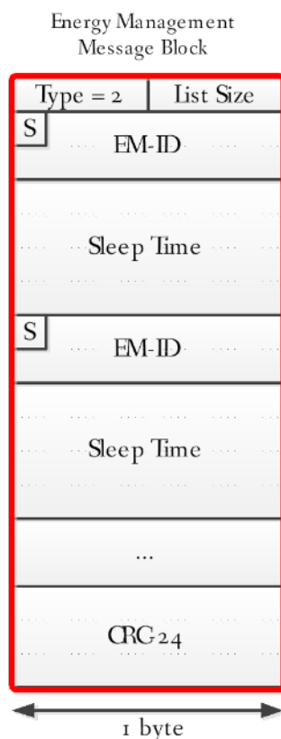
Figure 102 - Energy Management Message Block
