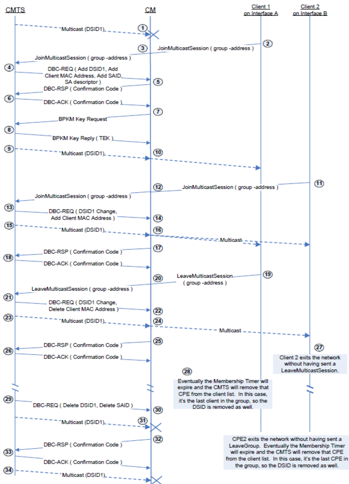
Figure 142 - Example – Encrypted Downstream Multicast Forwarding
