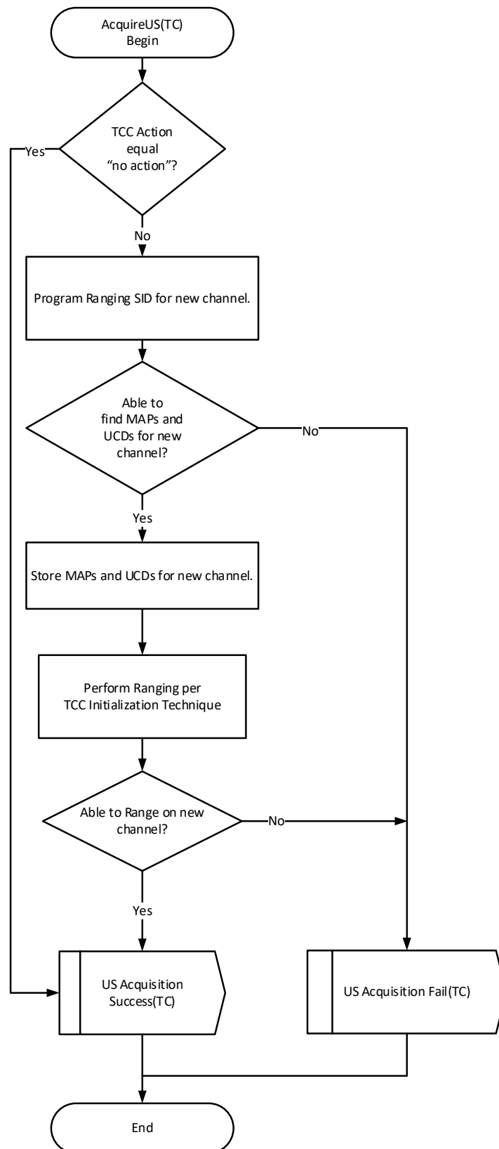
Figure 173 - CM Acquires Upstream Channel
