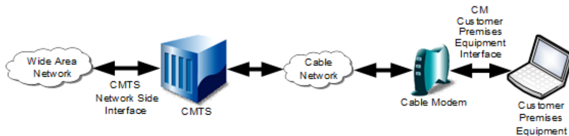
Figure 3 - Transparent IP Traffic Through the Data-Over-Cable System
