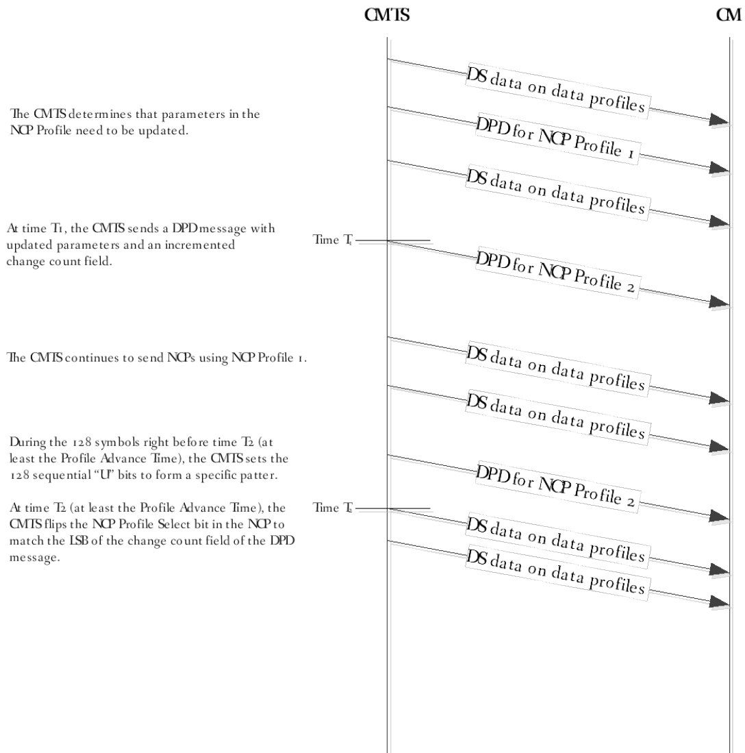
Figure 327 - DPD Change to the NCP Profile
