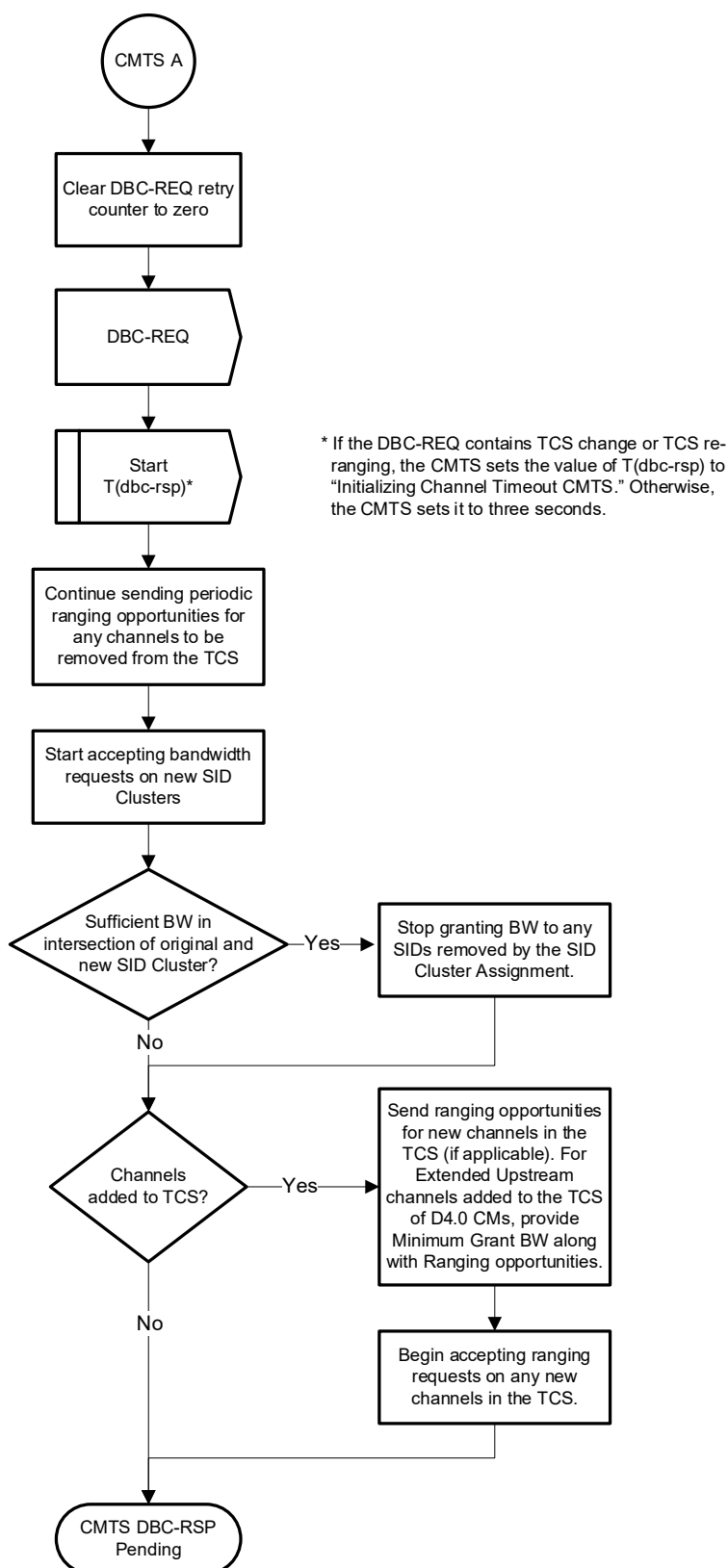
Figure 245 - CMTS DBC Request (part 2)
