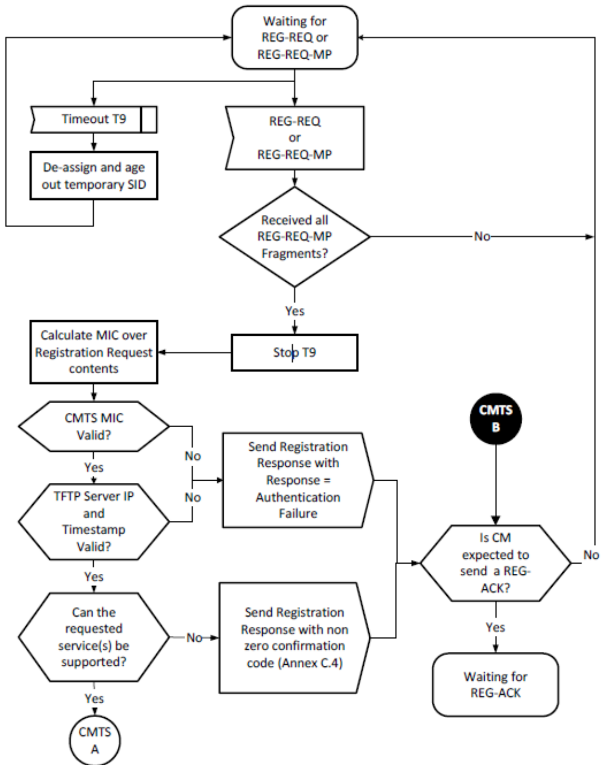
Figure 175 - CMTS Registration - Begin
