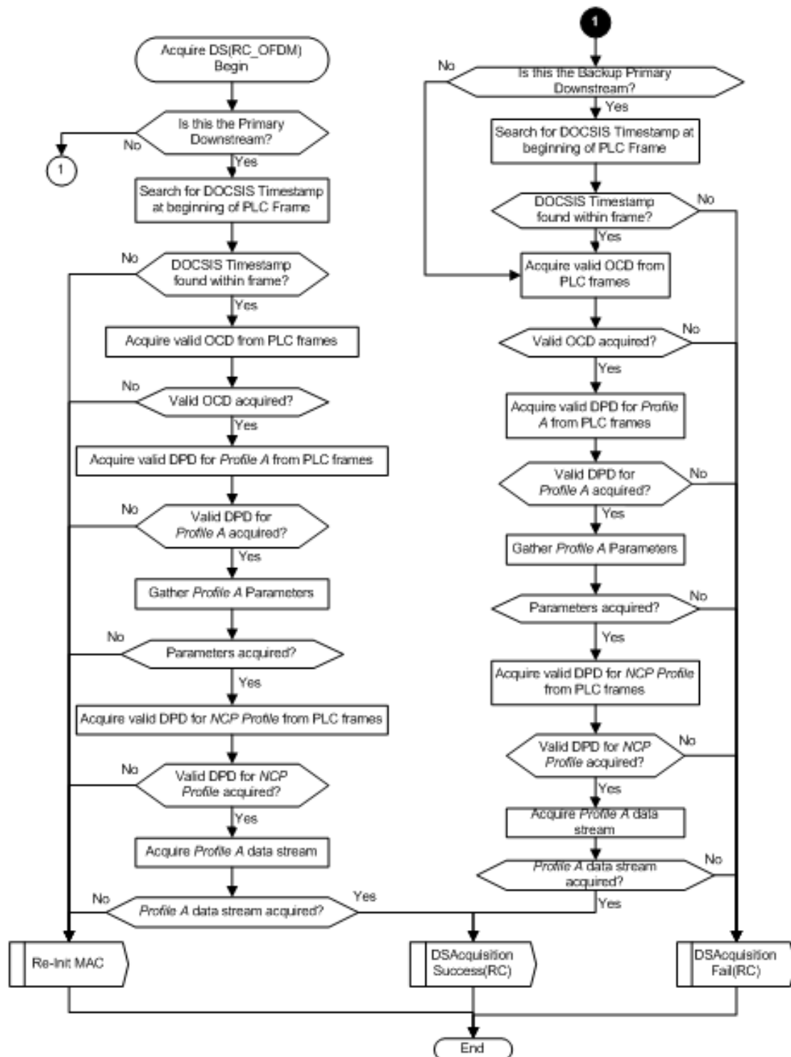
Figure 254 - CM AcquiredS Procedure for OFDM
