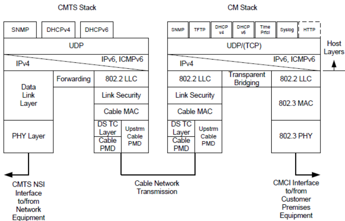
Figure 138 - DOCSIS Protocol Stacks
