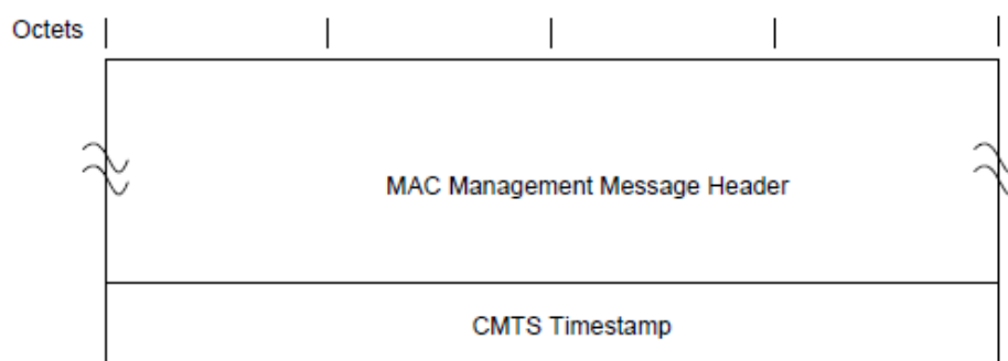
Figure 33 - Format of Packet PDU Following the Timing Header
