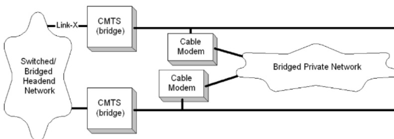
Figure 302 - Spanning Tree Across CMTSs
