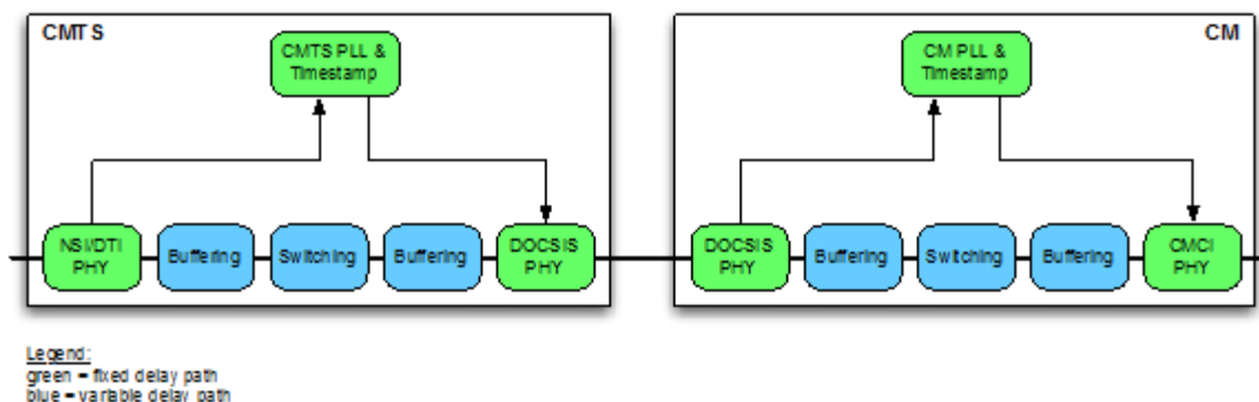
Figure 194 - DOCSIS Time Protocol Fixed Latency Path Example
