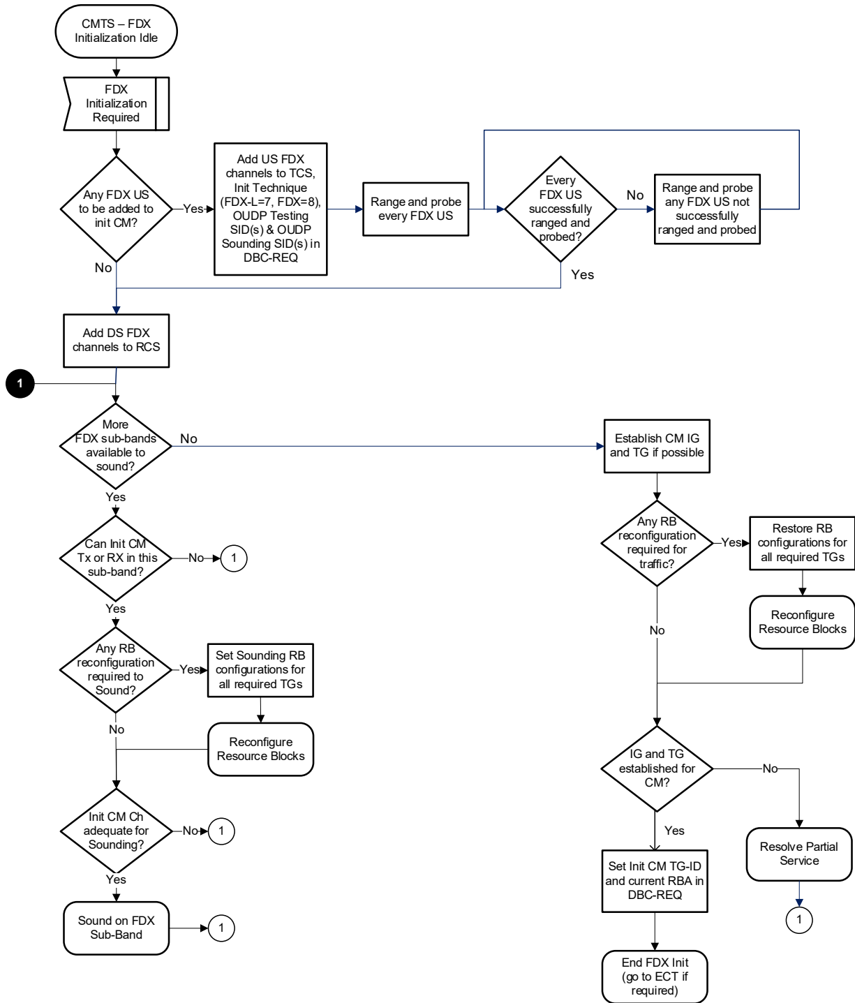
Figure 268 - CM FDX Initialization (CMTS Perspective)
