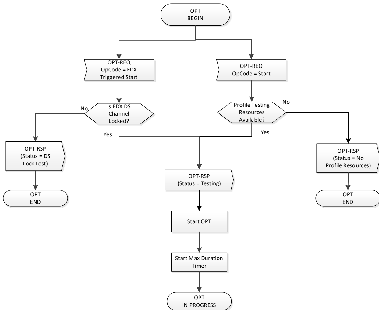
Figure 182 - CM OPT State Machine – OPT Idle
