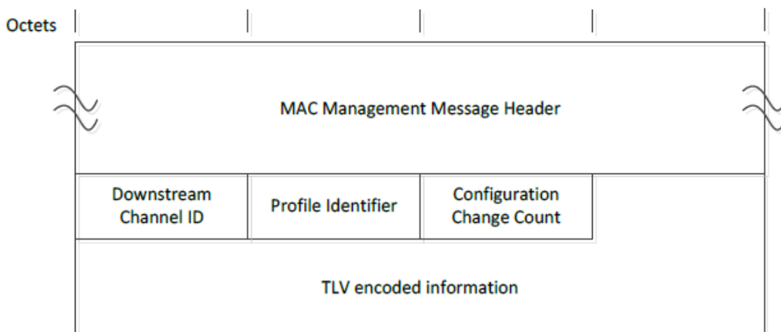
Figure 84 - Downstream Profile Descriptor
