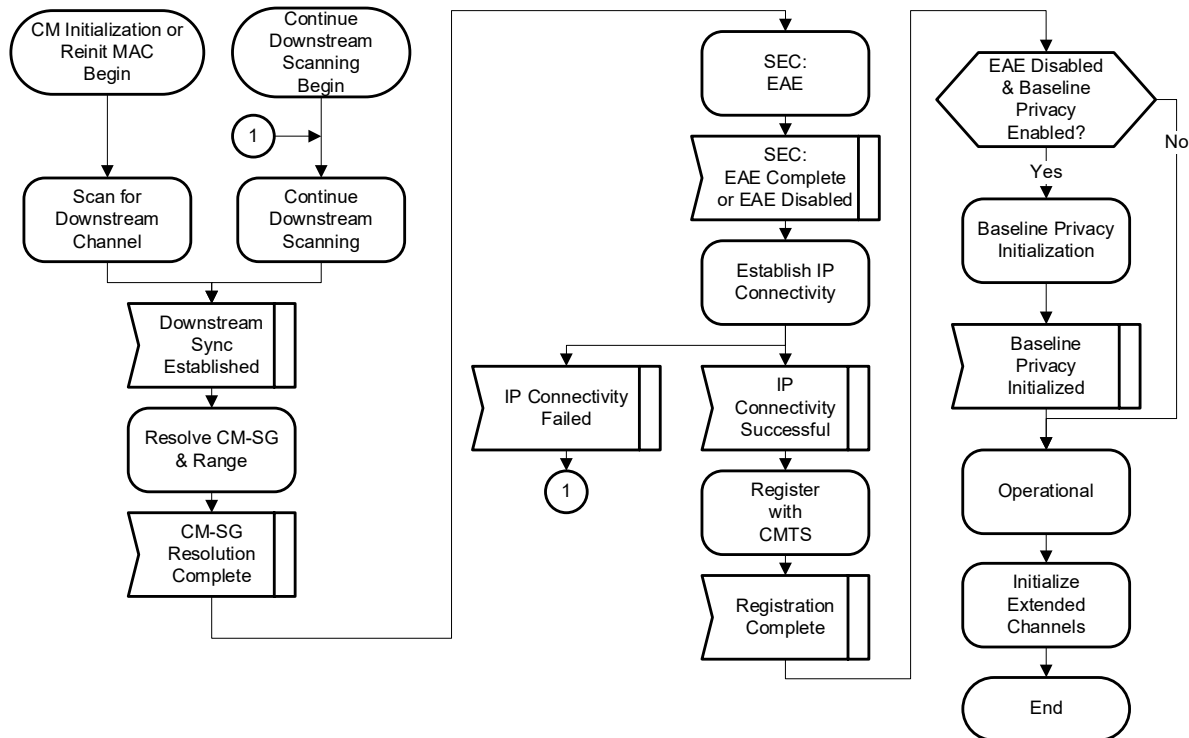
Figure 143 - Cable Modem Initialization Overview
