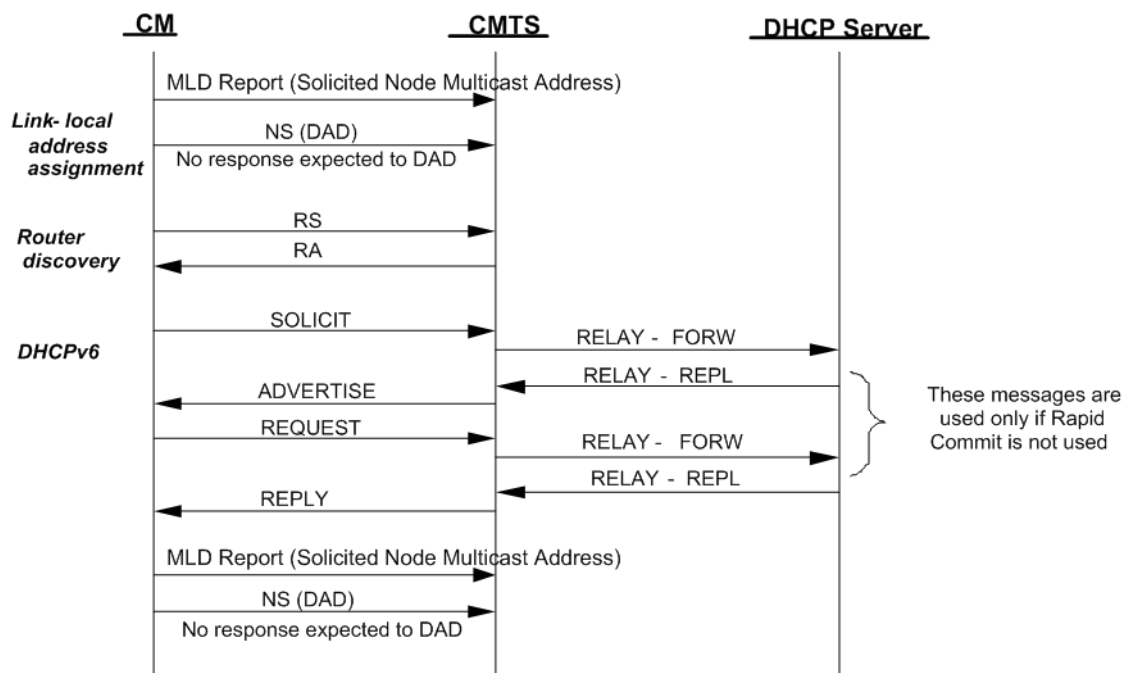
Figure 167 - IPv6 Provisioning Message Flow
