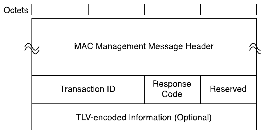
Figure 81 - Energy Management Response Message
