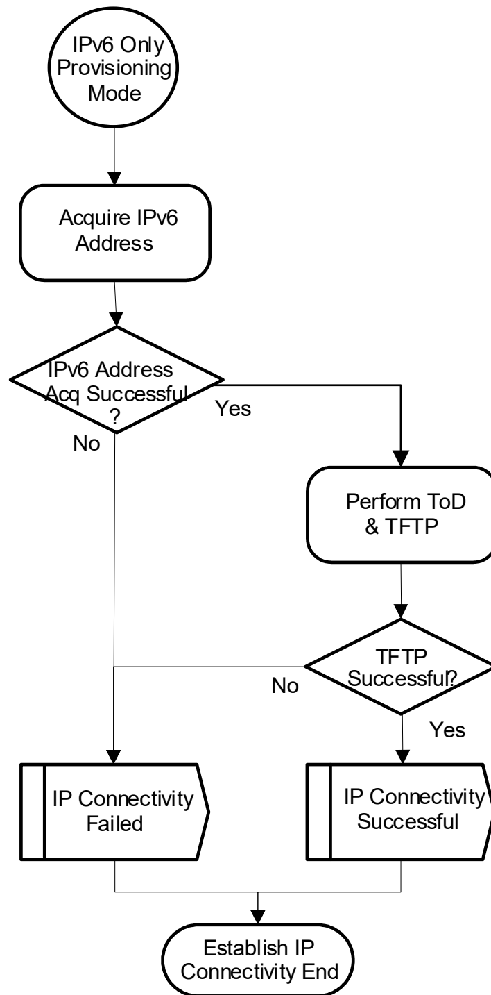
Figure 161 - IPv6 Only Provisioning Mode
