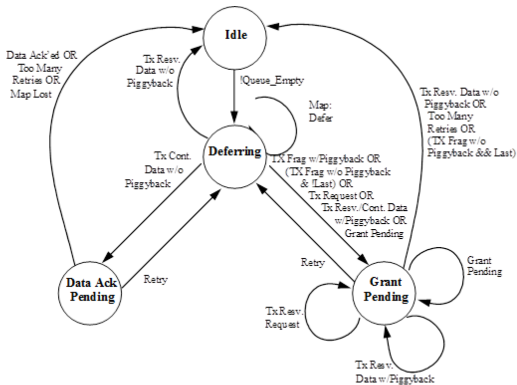
Figure 306 - Transmission and Deference State Transition Diagram
