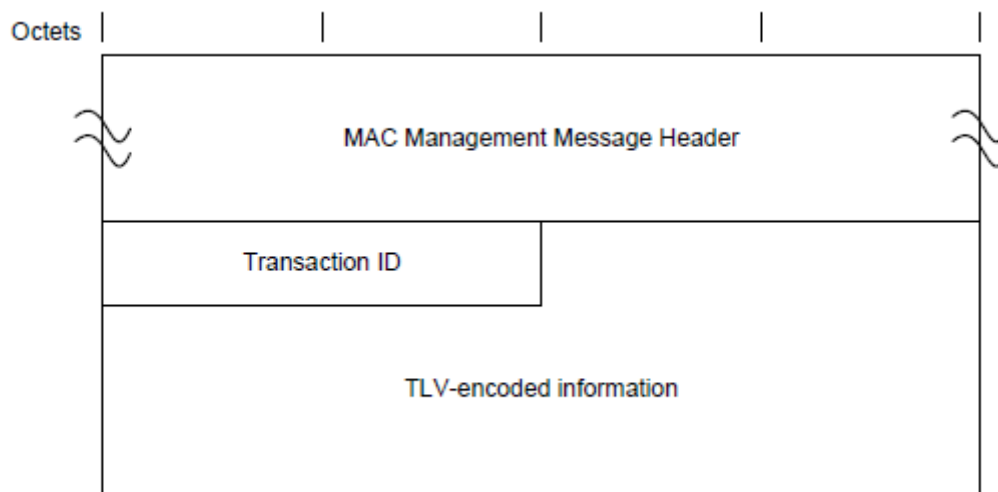
Figure 90 - DTP Response Message
