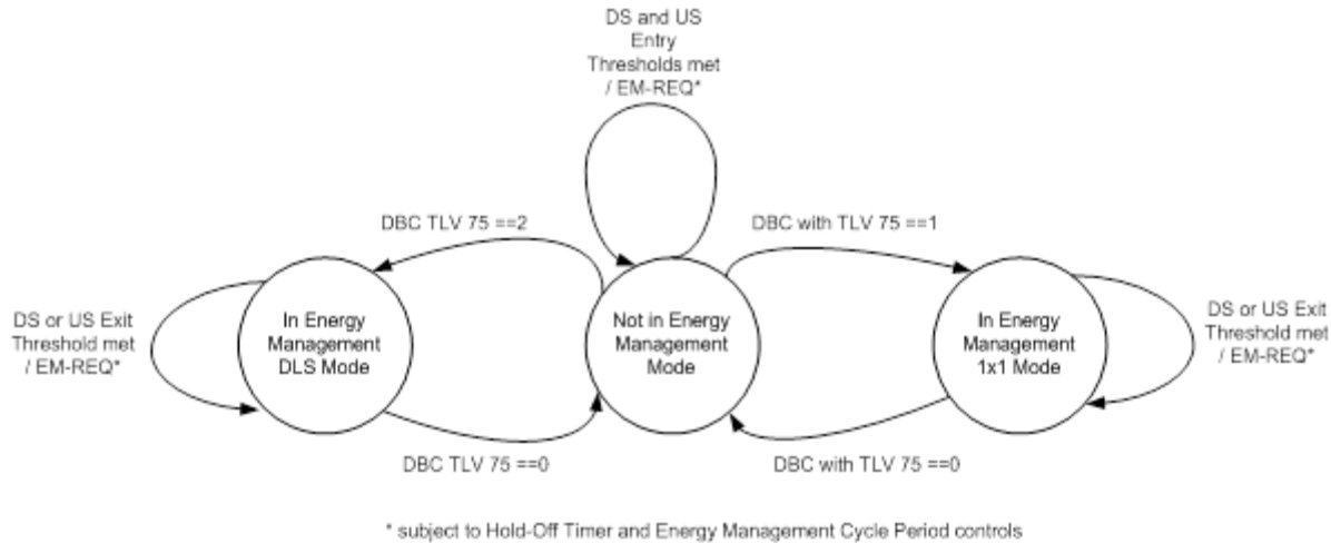
Figure 257 - Energy Management Modes State Diagram
