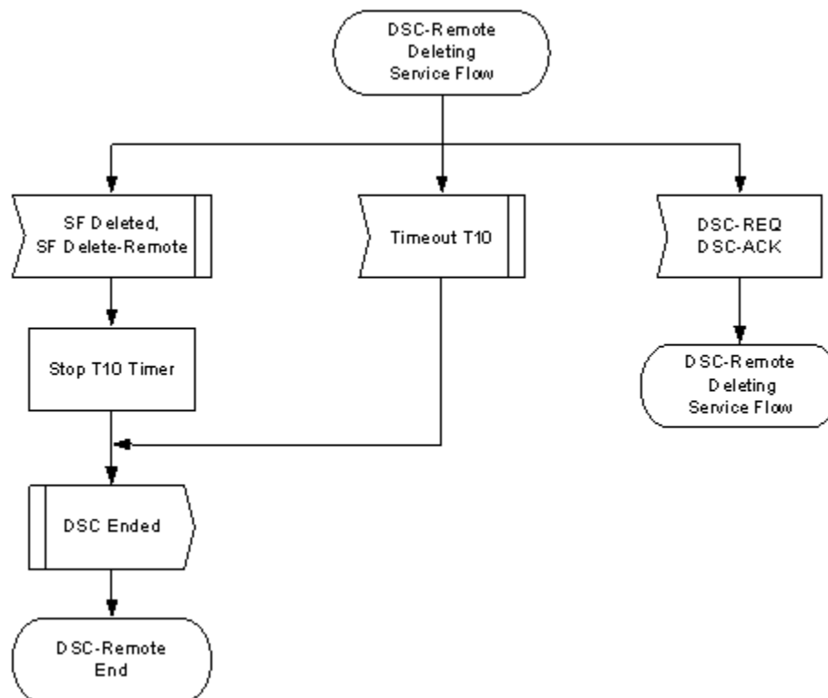
Figure 231 - DSC-Remotely Initiated Transaction Deleting Service Flow State Flow Diagram
