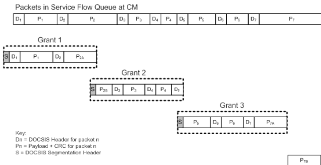
Figure 115 - CCF Using Segment Headers
