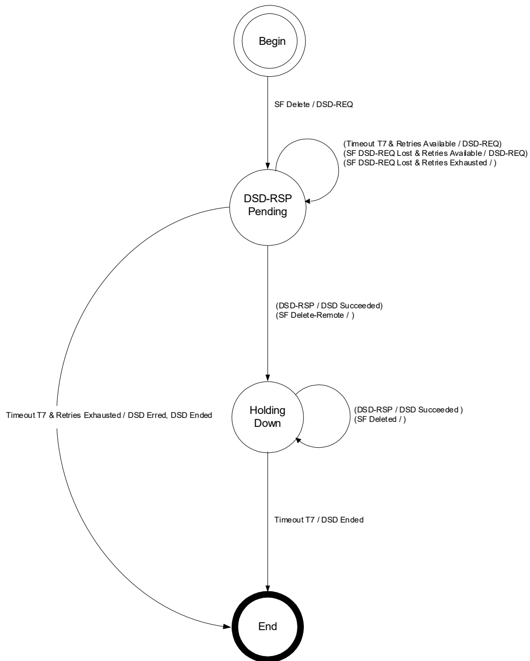
Figure 207 - DSD-Locally Initiated Transaction State Transition Diagram
