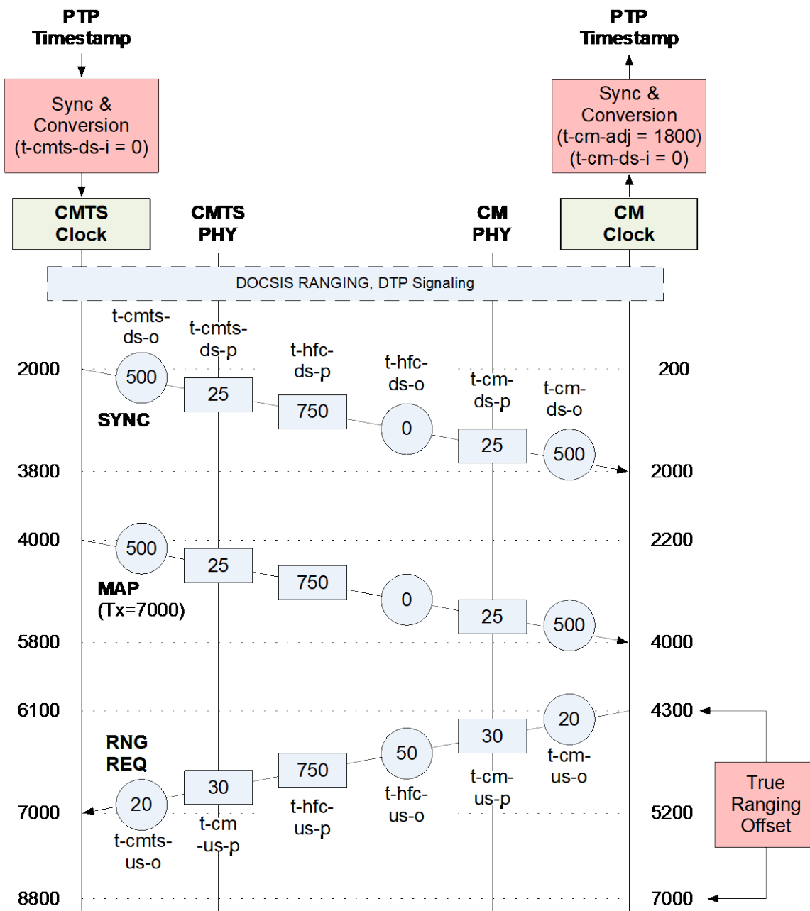
Figure 197 - True Ranging Offset Example
