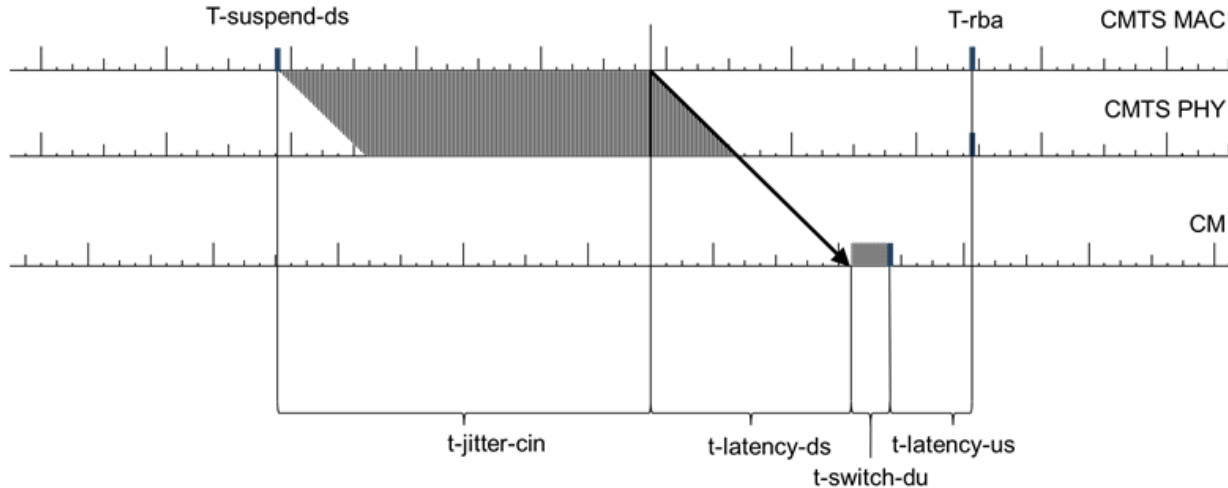
Figure 285 - T\text{-suspend-ds} R-PHY Timing
