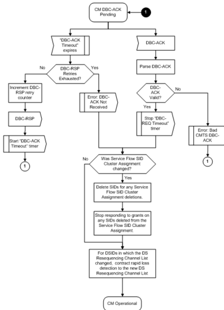
Figure 256 - CM DBC-ACK Pending
