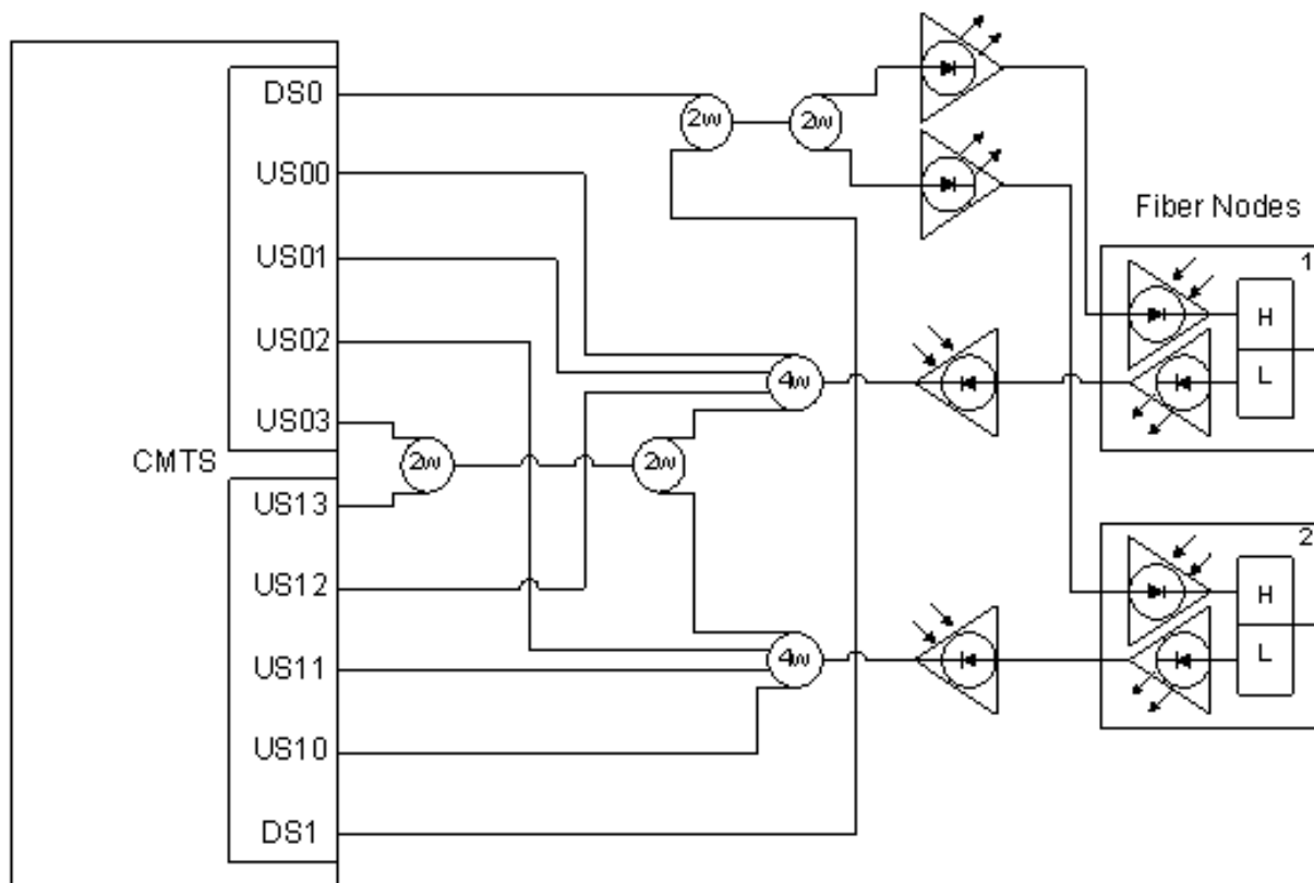
Figure 325 - Example Combining Network 2
