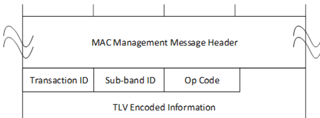
Figure 94 - CW Test Request (CWT-REQ) Message
