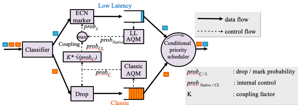
Figure 134 - Coupling between the Classic AQM and the Low Latency AQM
