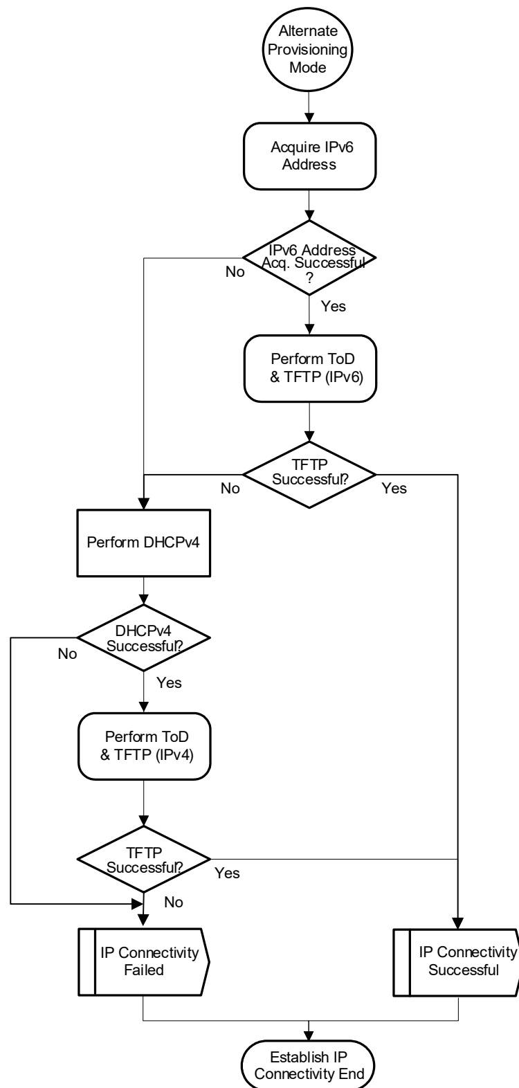
Figure 162 - Alternate Provisioning Mode
