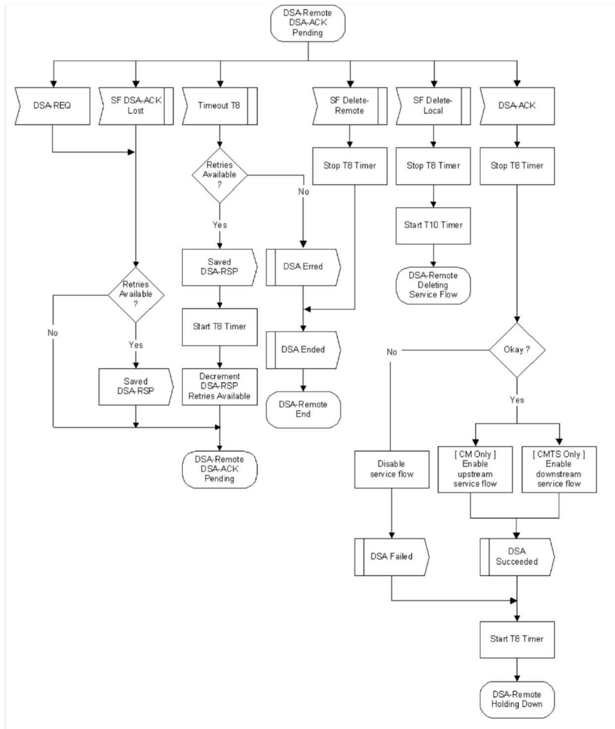
Figure 217 - DSA-Remotely Initiated Transaction DSA-ACK Pending State Flow Diagram
