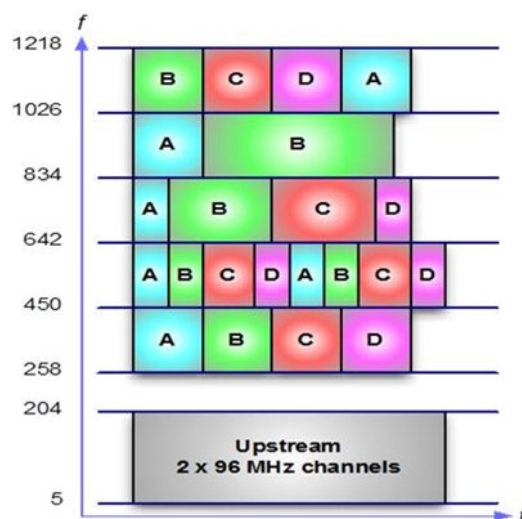
Figure 5 - Example View of DS and US Channels and DS Profiles
