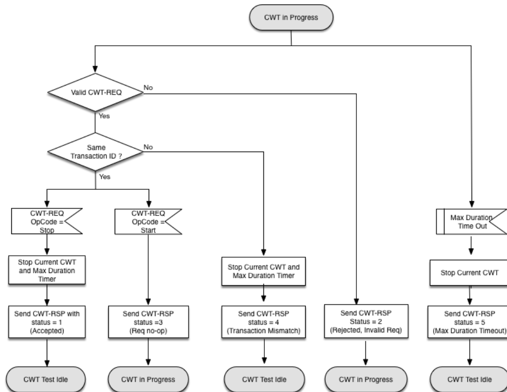
Figure 275 - CWT Sounding Transaction at Test CM - CWT in Progress
