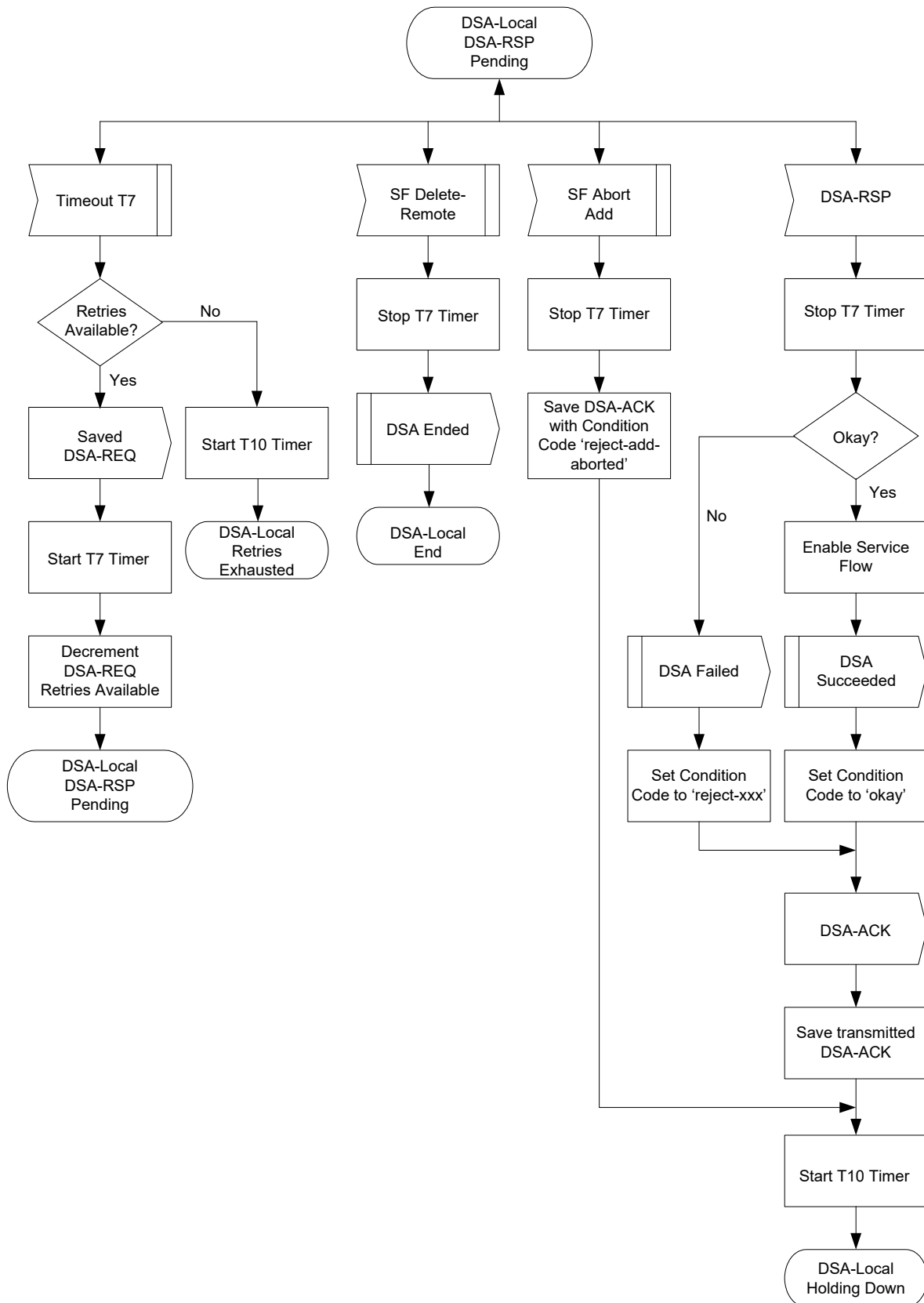
Figure 212 - DSA-Locally Initiated Transaction DSA-RSP Pending State Flow Diagram
