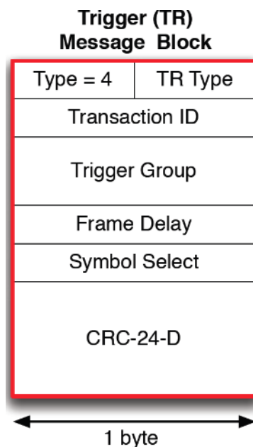
Figure 104 - Trigger Message Block
