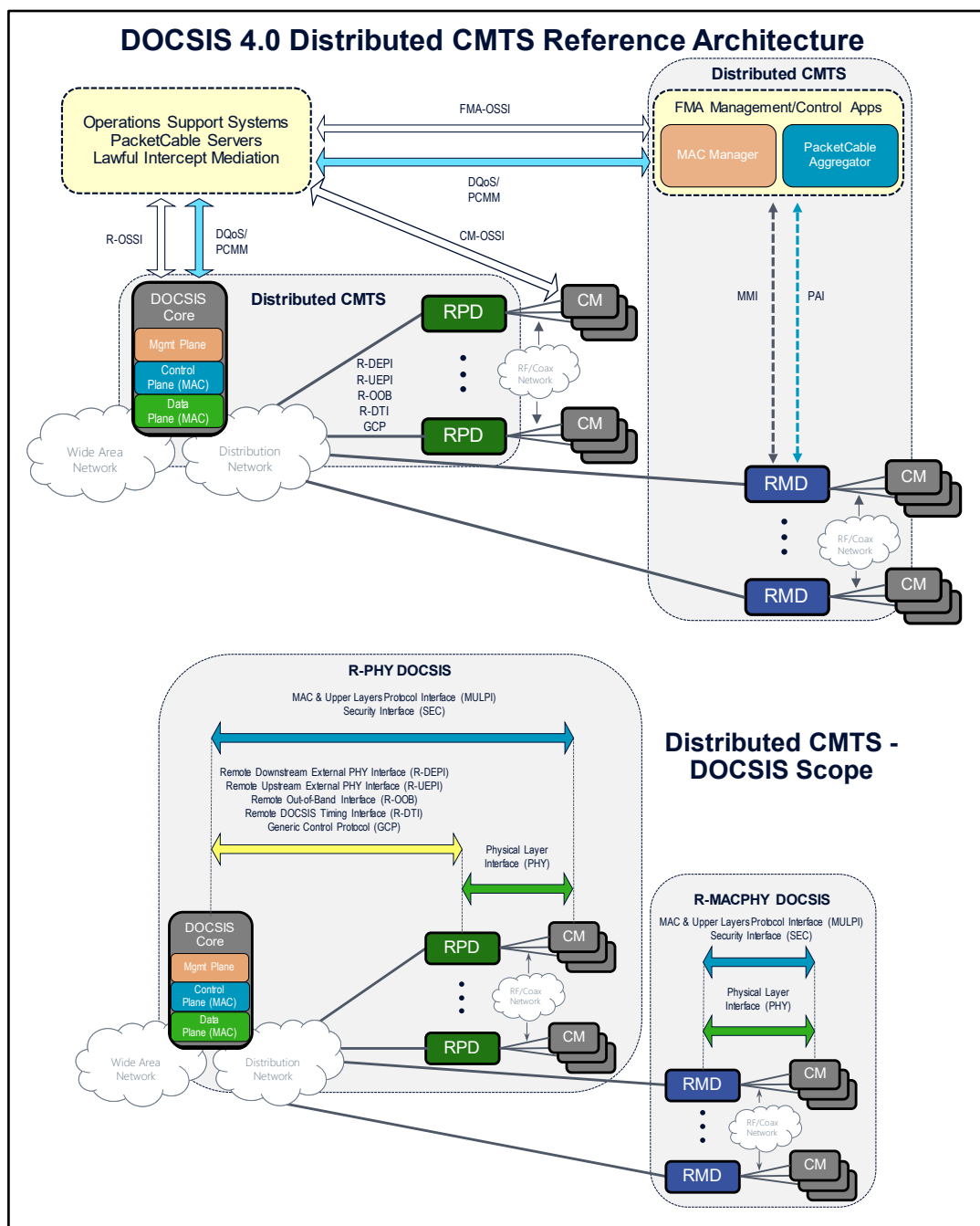
Figure 4 - Data-Over-Cable Reference Architecture
