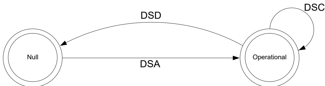
Figure 201 - Dynamic Service Flow Overview
