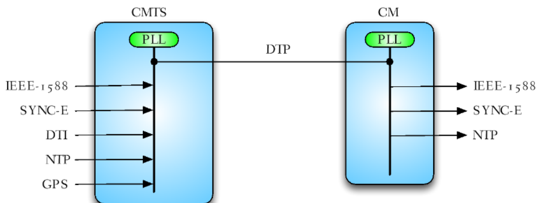
Figure 193 - DOCSIS Time Protocol System Overview
