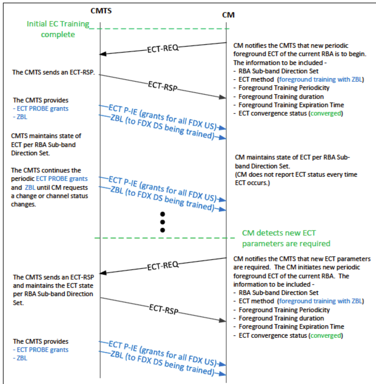
Figure 281 - Periodic Foreground Training with ZBL
