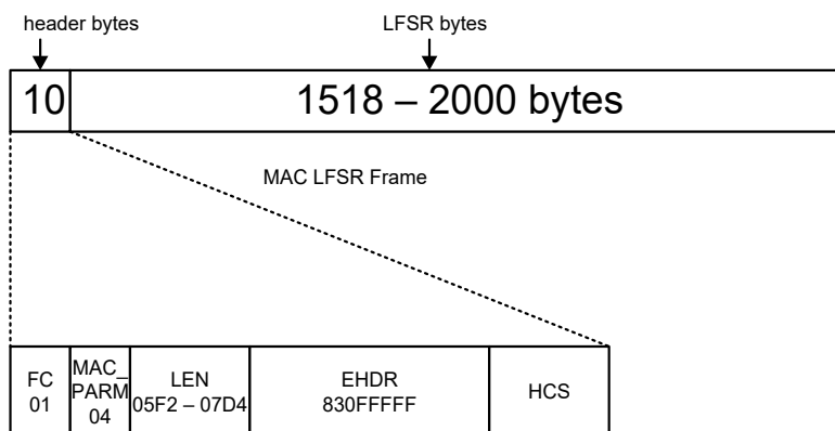
Figure 186 - MAC LFSR Frame
