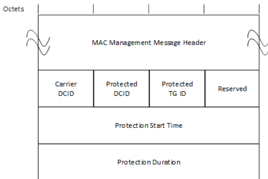
Figure 98 - Downstream Protection (DPR) Message
