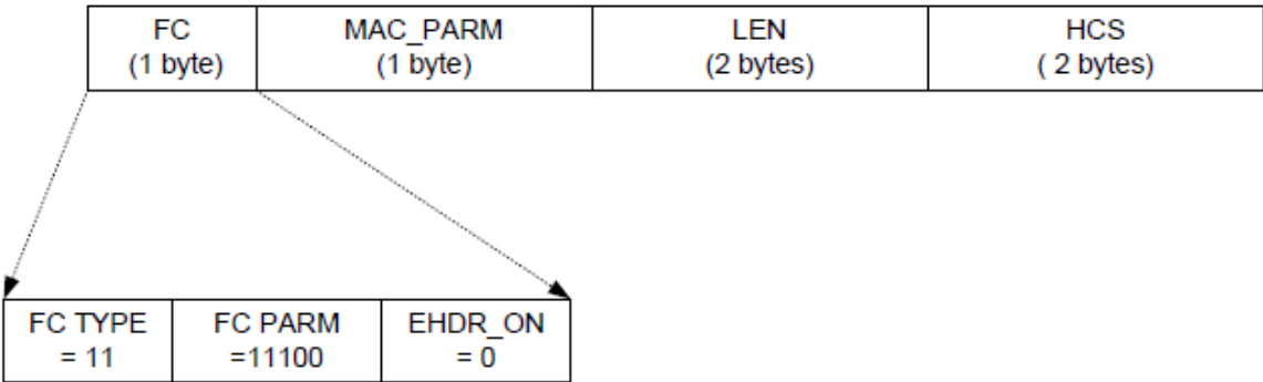
Figure 29 - Concatenation MAC Header Format
