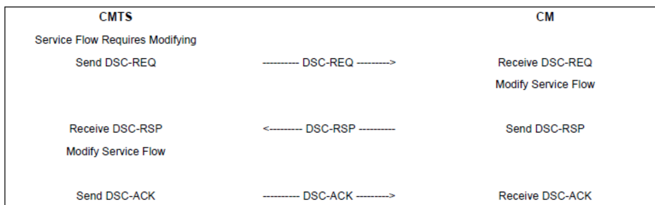
Figure 221 - CMTS-Initiated DSC Modifying a Service Flow
