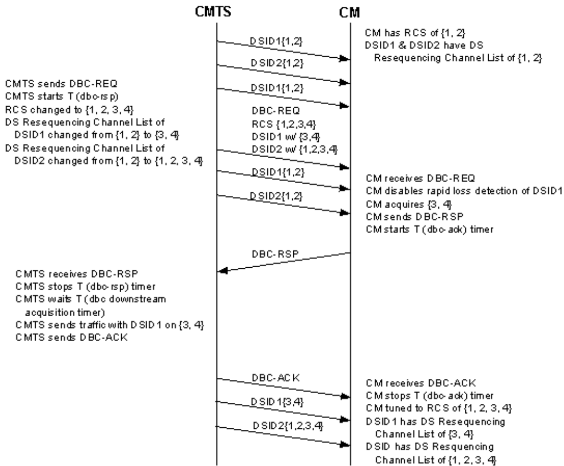
Figure 322 - Changing the RCS and Downstream Resequencing Channel List
