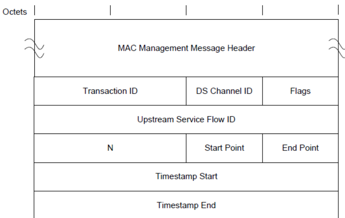
Figure 75 - DPV-REQ MAC Message
