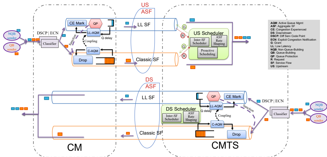
Figure 128 - Low Latency System Architecture Diagram
