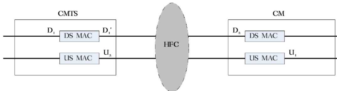
Figure 192 - DPV Reference Diagram
