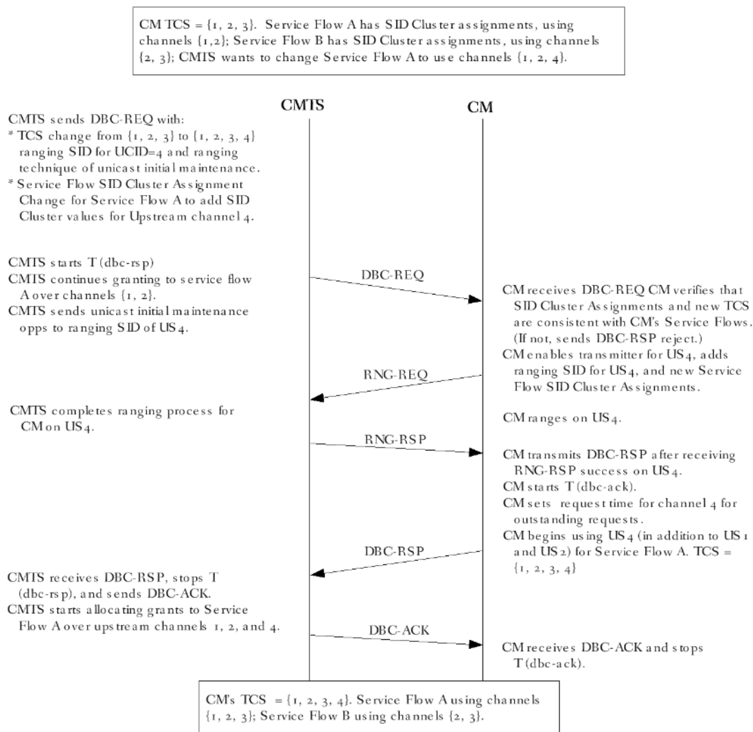
Figure 321 - Adding a Channel to the TCS and making a Service Flow SID Cluster Assignment
