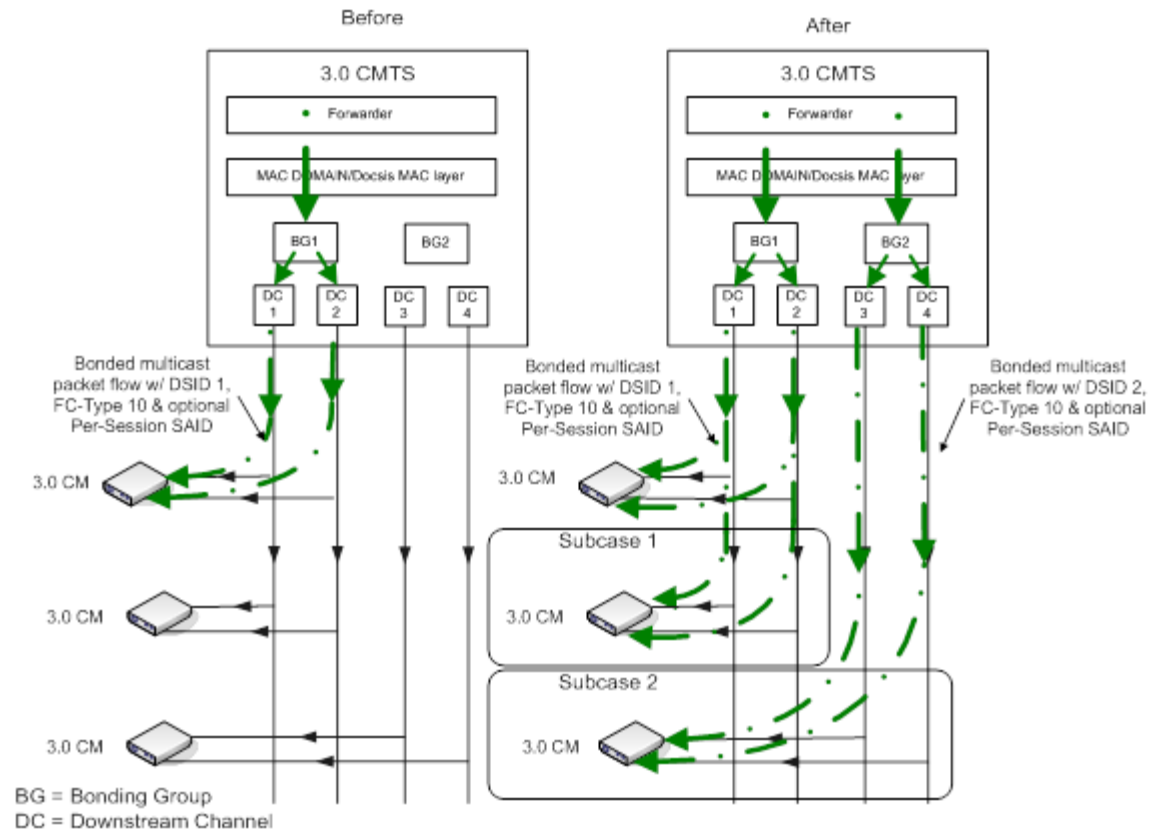
Figure 319 - Multicast Session Replication to Clients Behind Two 3.0 CMs
