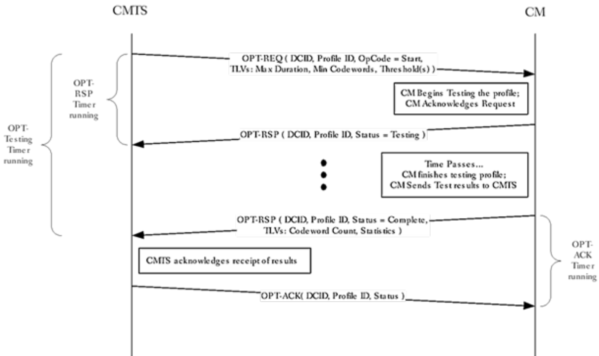
Figure 180 - Typical OFDM Profile Test Transaction
