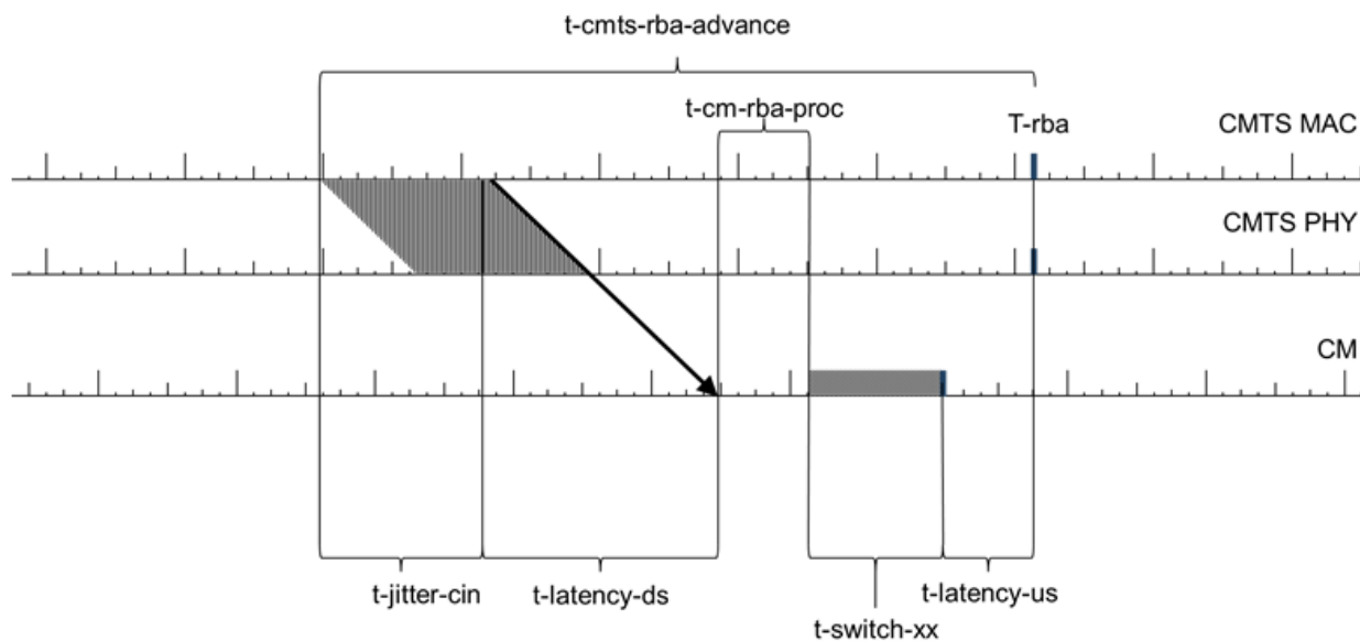
Figure 290 - t-cmts-rba-advance and t-cm-rba-proc Timing
