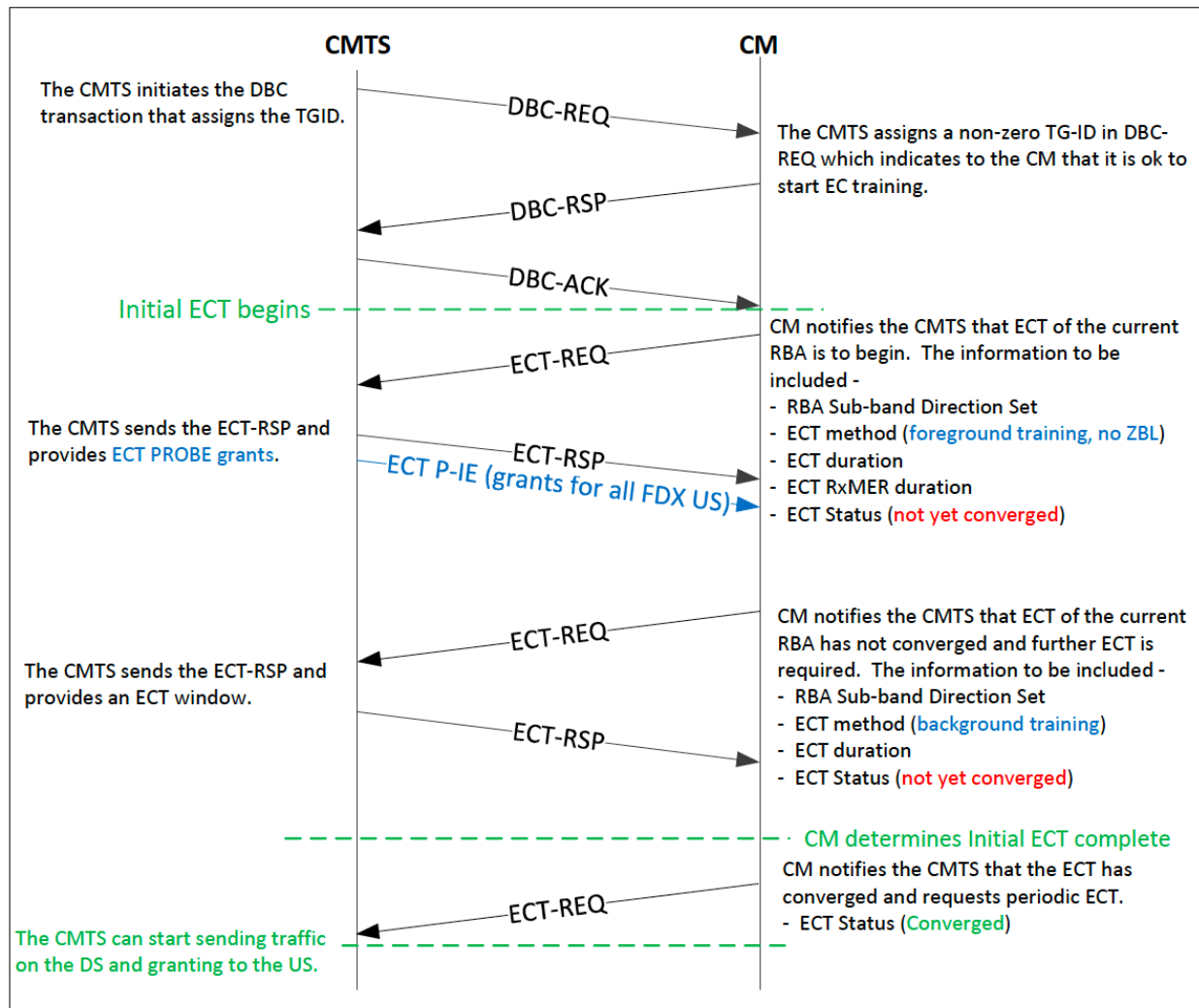
Figure 280 - Initial EC Training of Background Training and Foreground Training Without ZBL
