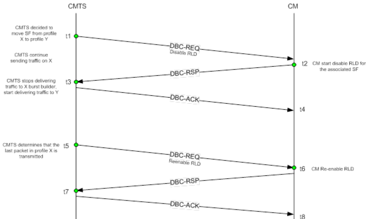
Figure 323 - DBC procedure for SF profile switch on OFDM channel
