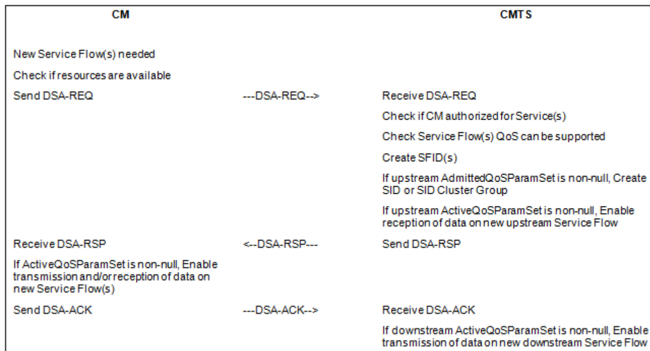
Figure 209 - Dynamic Service Addition Initiated from CM
