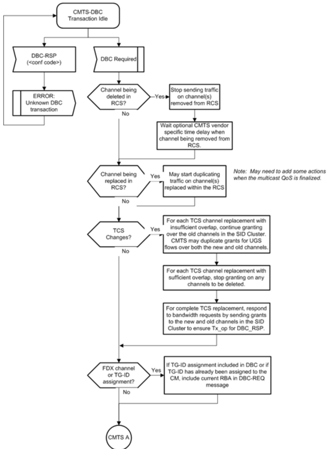
Figure 244 - CMTS DBC Request (part 1)
