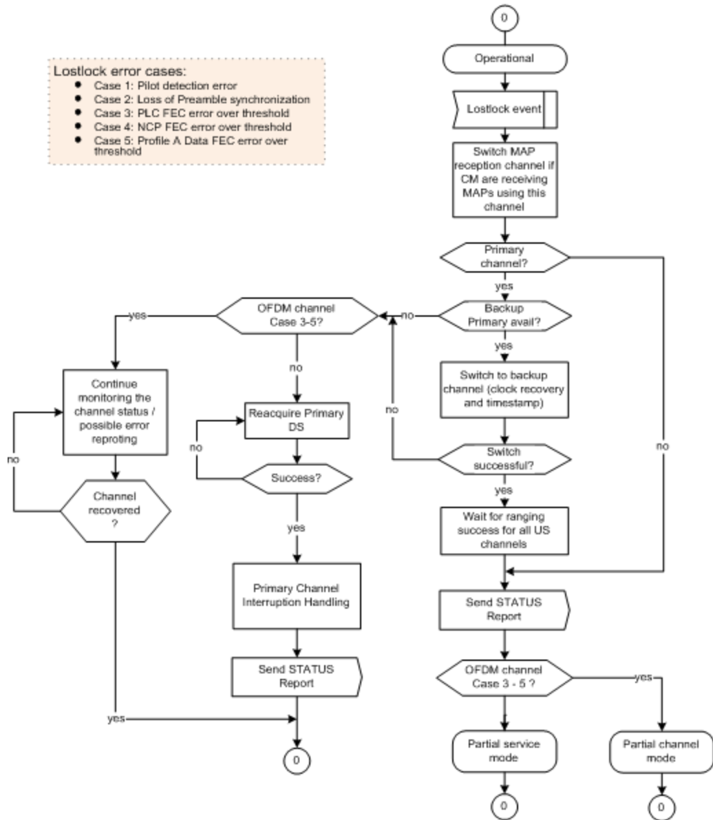
Figure 190 - Lost Lock on an OFDM Channel Procedure
