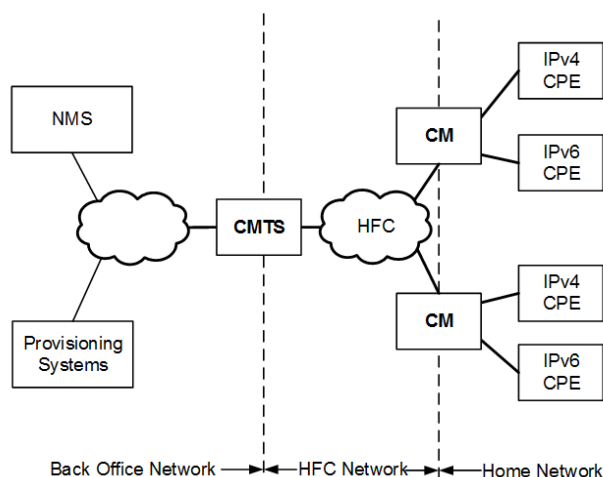
Figure 2 - The Legacy DOCSIS Network
