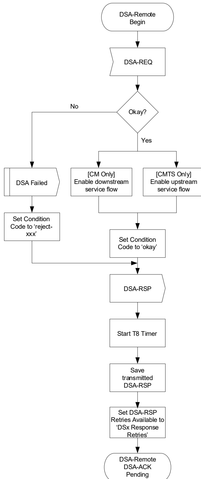
Figure 216 - DSA-Remotely Initiated Transaction Begin State Flow Diagram
