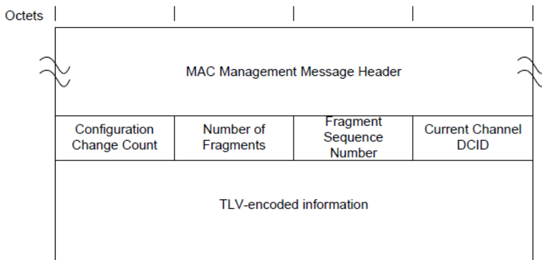
Figure 70 - MAC Domain Descriptor
