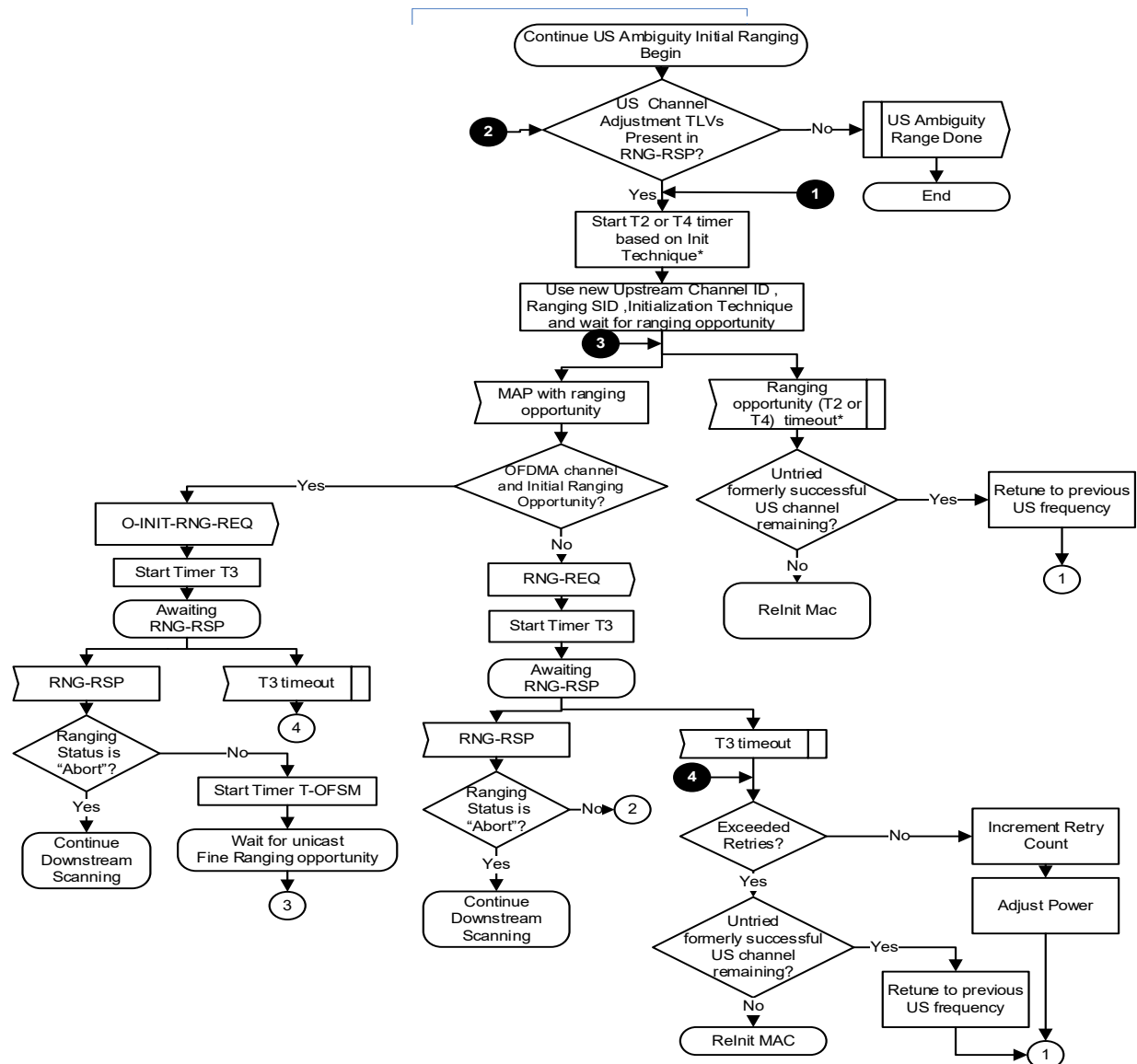
Figure 153 - Continue US Ambiguity Initial Ranging
