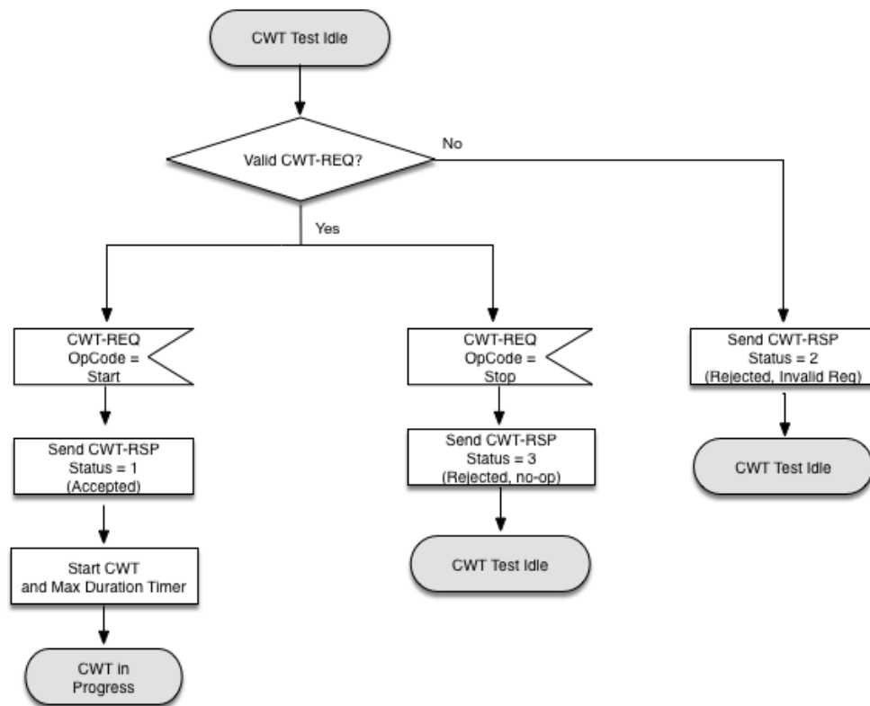
Figure 274 - Sounding Transactions at Test CM - CWT Test Idle
