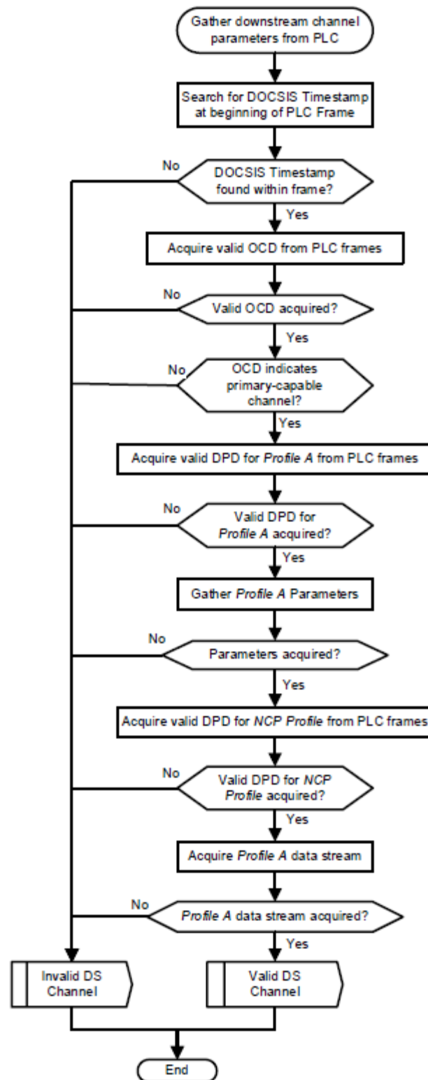
Figure 145 - Gather Downstream Channel Parameters from PLC
