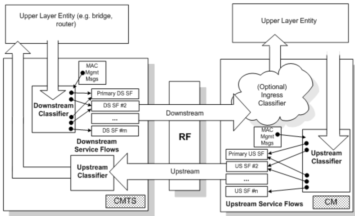
Figure 118 - Classification within the MAC Layer
