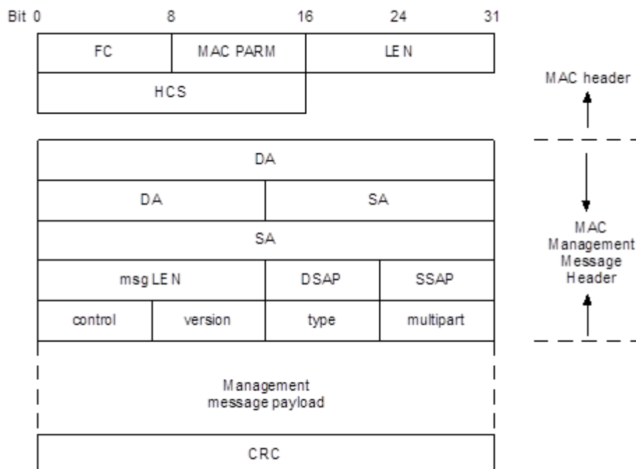
Figure 32 - MAC Header and MAC Management Message Header Fields
