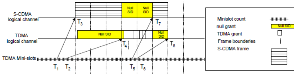
Figure 111 - Logical S-CDMA and TDMA Channels
