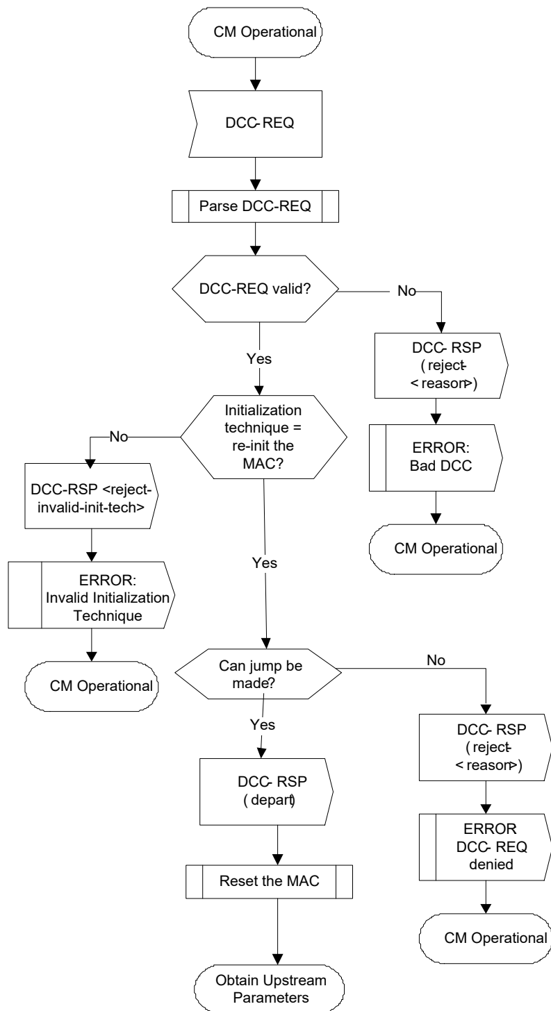
Figure 243 - Dynamically Changing Channels: CM View
