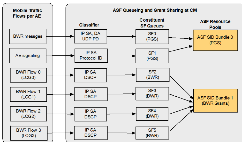
Figure 127 - DHQoS ASF SID Bundle Assignment Example - Two ASF SID Bundles
