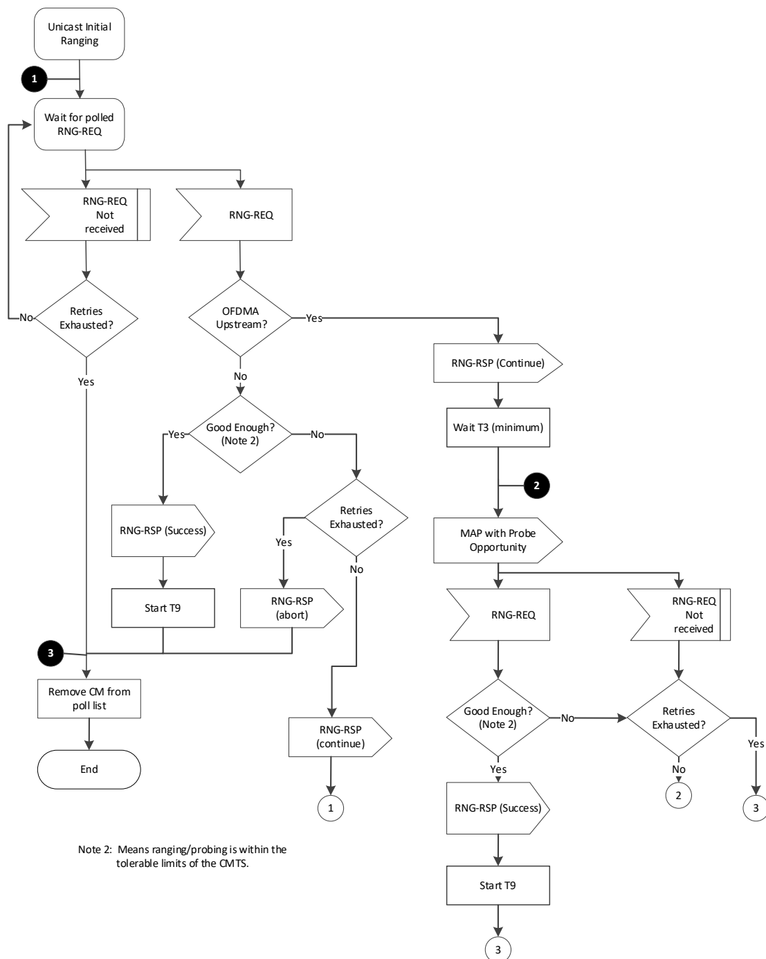
Figure 158 - Unicast Initial Ranging - CMTS
