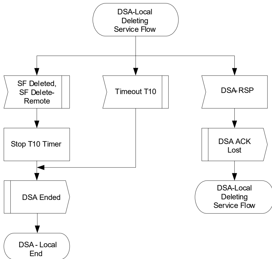
Figure 215 - DSA-Locally Initiated Transaction Deleting Service Flow State Flow Diagram
