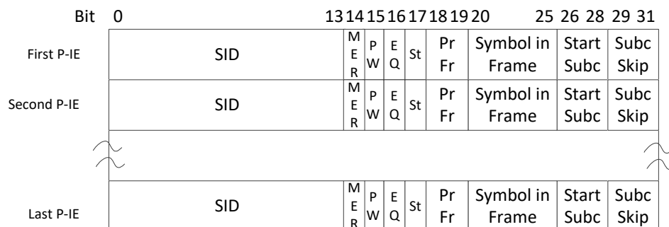
Figure 43 - Probe Information Element Structure
