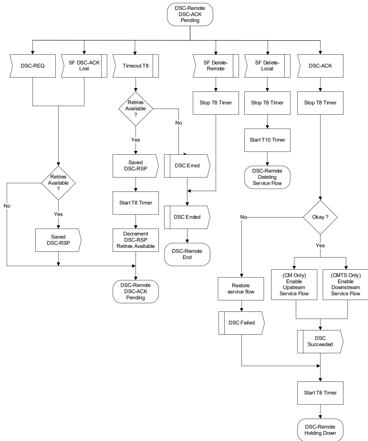
Figure 229 - DSC-Remotely Initiated Transaction DSC-ACK Pending State Flow Diagram
