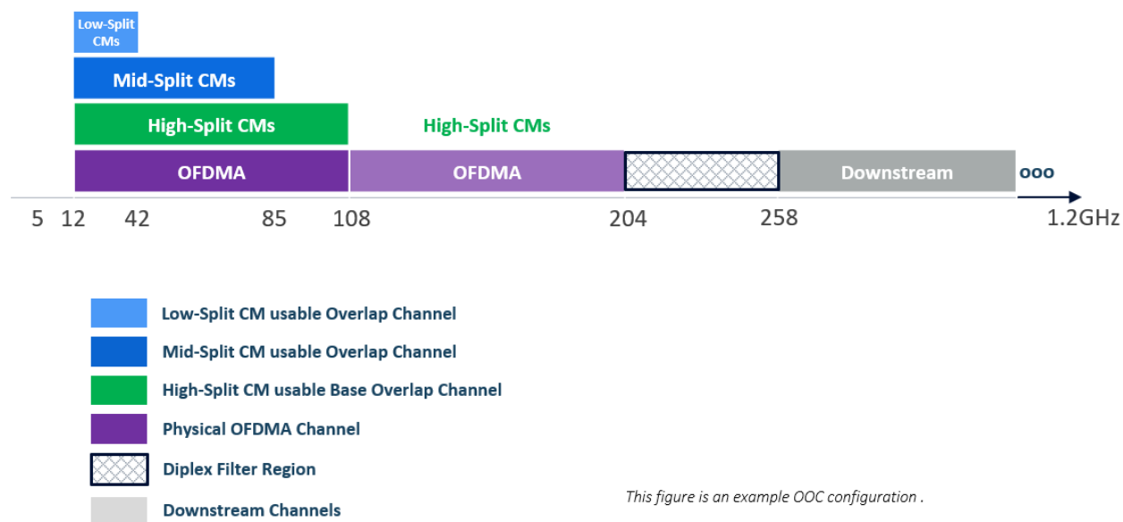
Figure 13 - Overlapping OFDMA Channels on High-Split Plant
