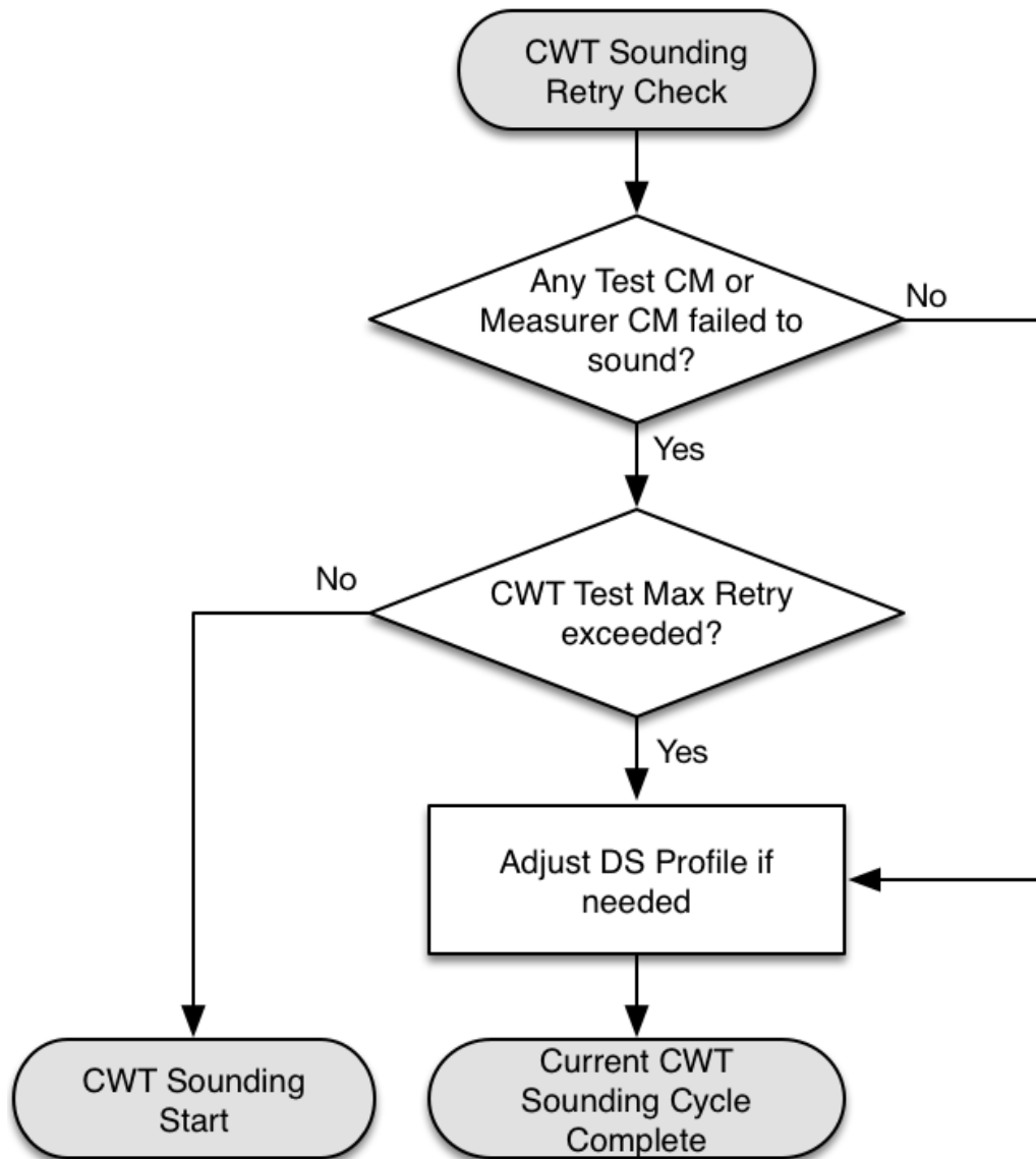
Figure 277 - CM Sounding Transactions – Retry Check
