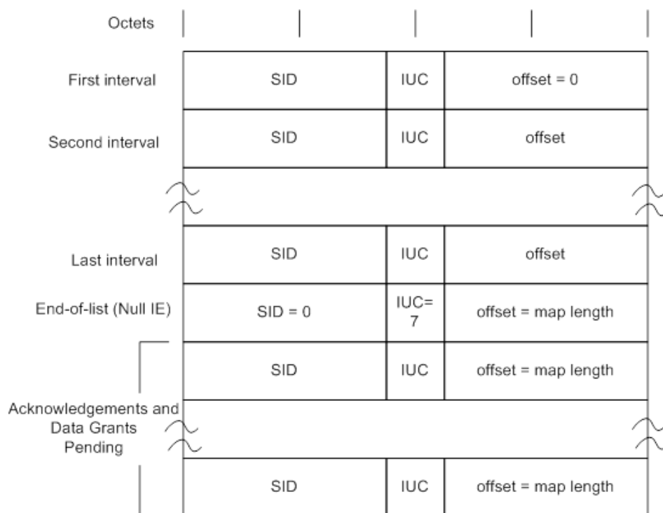
Figure 41 - MAP Information Element Structure
