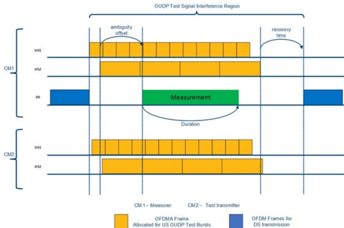
Figure 271 - OUDP Sounding Opportunities Timing Diagram
