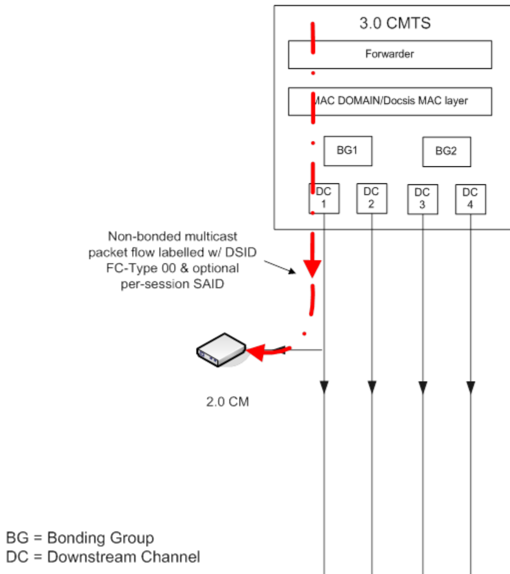
Figure 312 - Multicast Session Replication for a client behind a 2.0 CM
