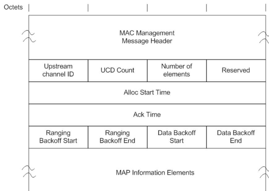
Figure 39 - Version 1 MAP Format
