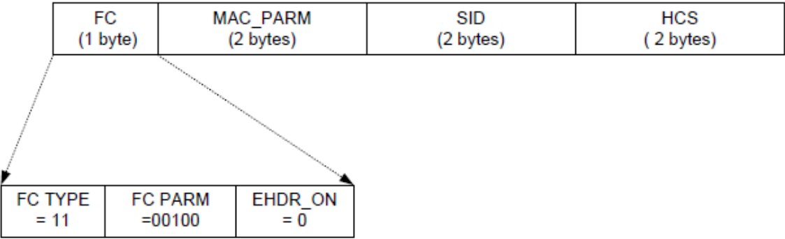
Figure 28 - Queue-depth Based Request Frame Format
