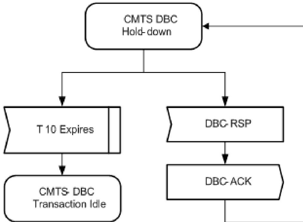
Figure 247 - CMTS DBC Hold-down
