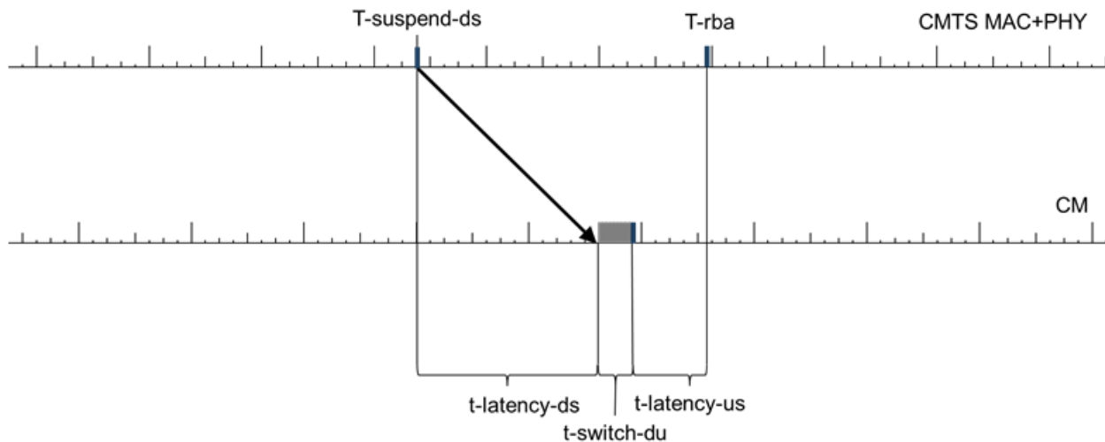
Figure 286 - T\text{-suspend-ds} CMTS Timing
