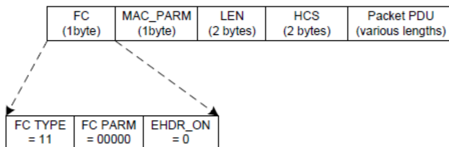
Figure 24 - Timing MAC Header
