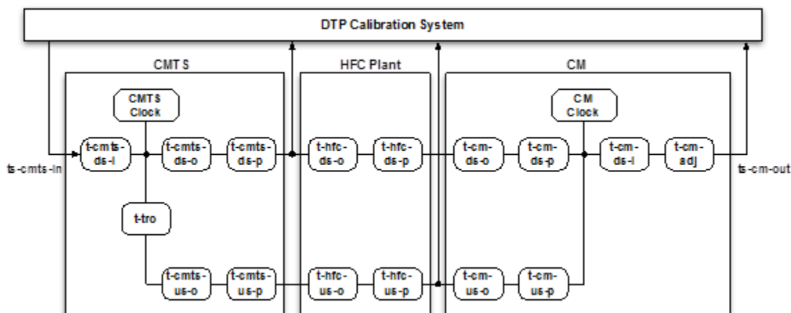
Figure 196 - DTP Math and Delays
