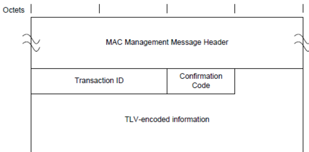
Figure 63 - Dynamic Service Change - Response
