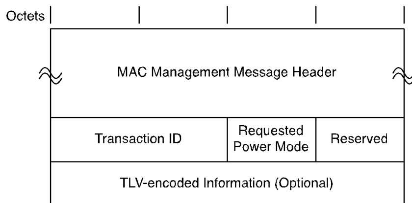
Figure 80 - Energy Management Request Message
