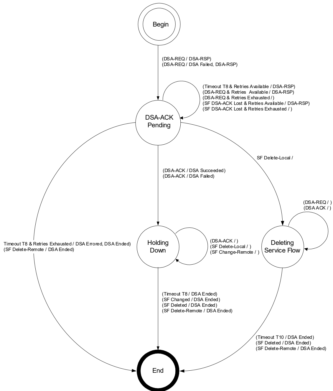
Figure 204 - DSA-Remotely Initiated Transaction State Transition Diagram
