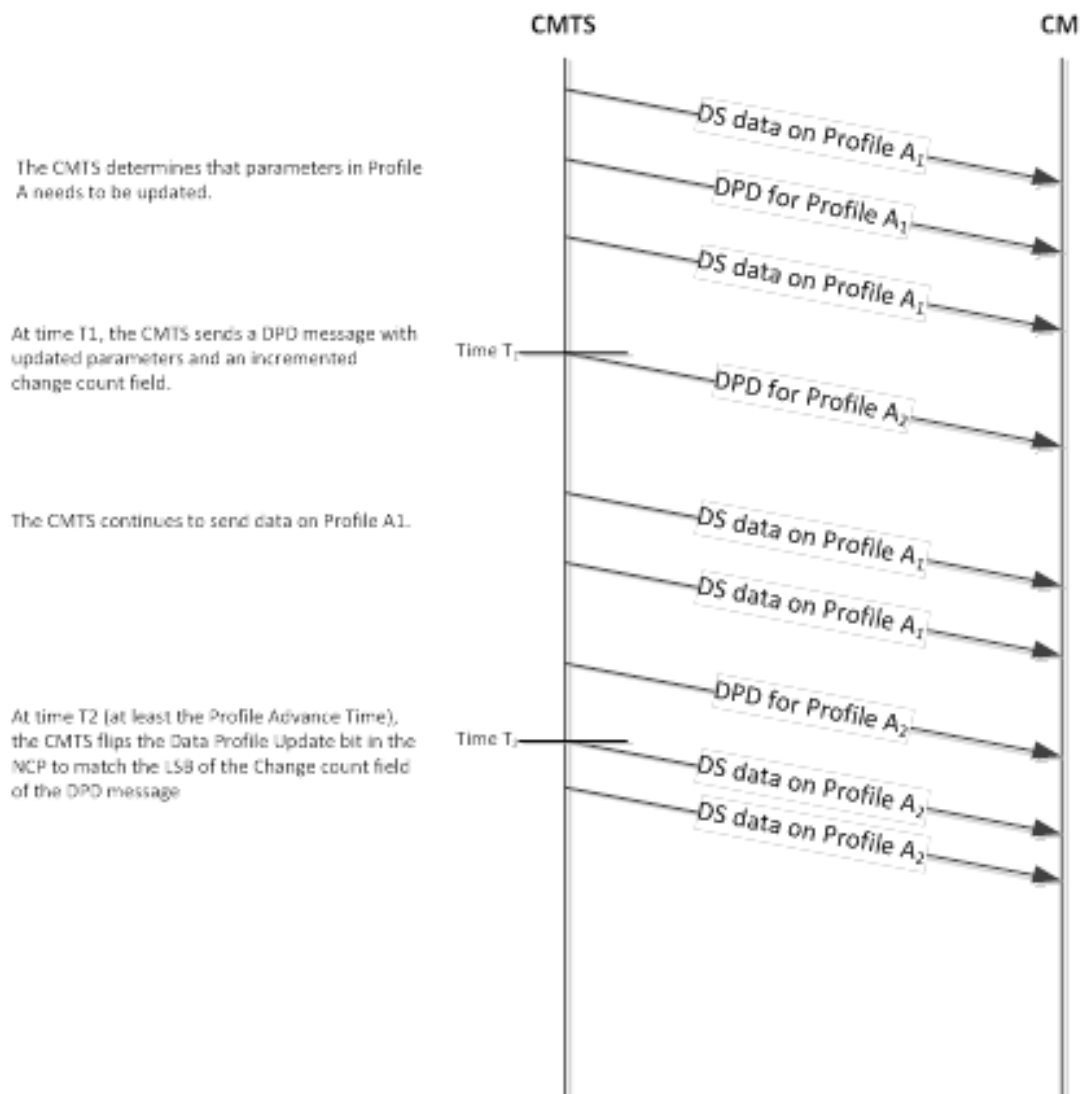
Figure 326 - DPD Change to Profile A
