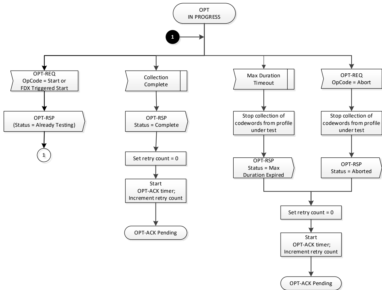
Figure 188 - CM OPT State Machine – OPT in Progress
