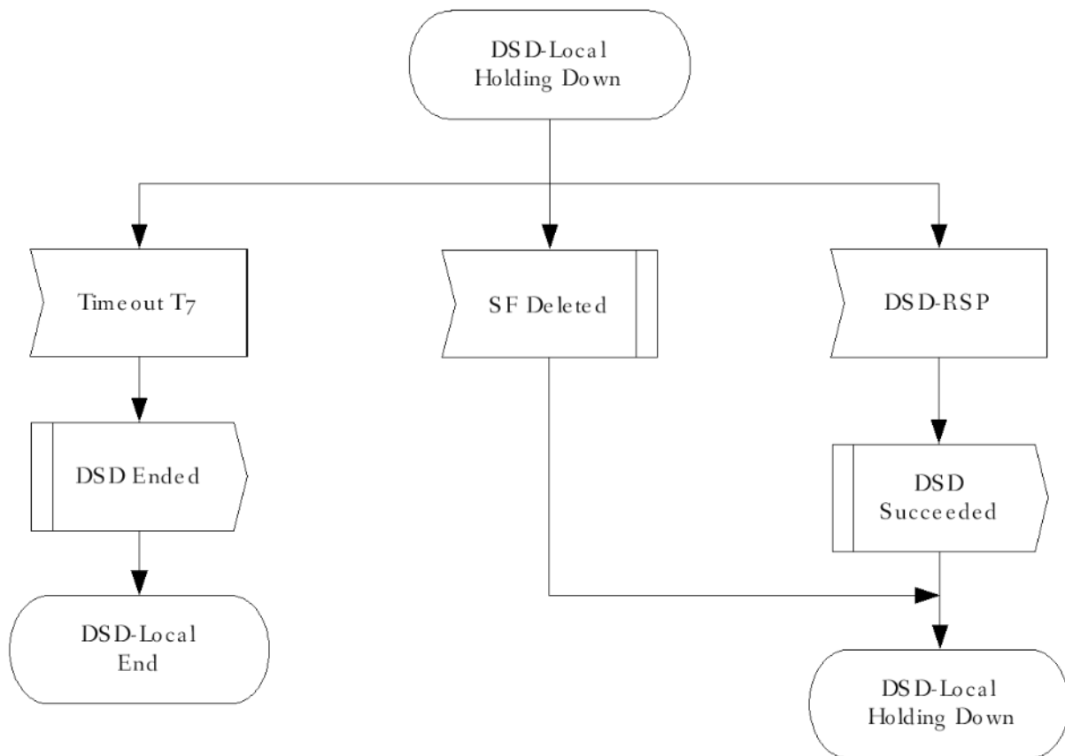
Figure 236 - DSD-Locally Initiated Transaction Holding Down State Flow Diagram
