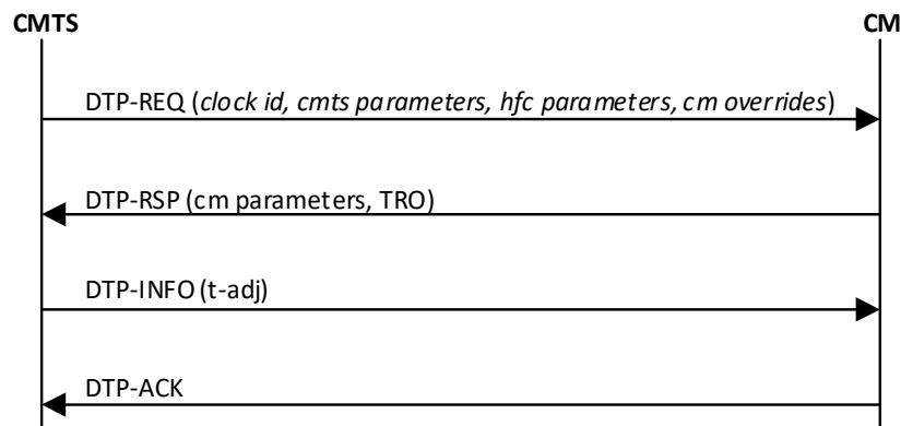
Figure 198 - CMTS is DTP Master
