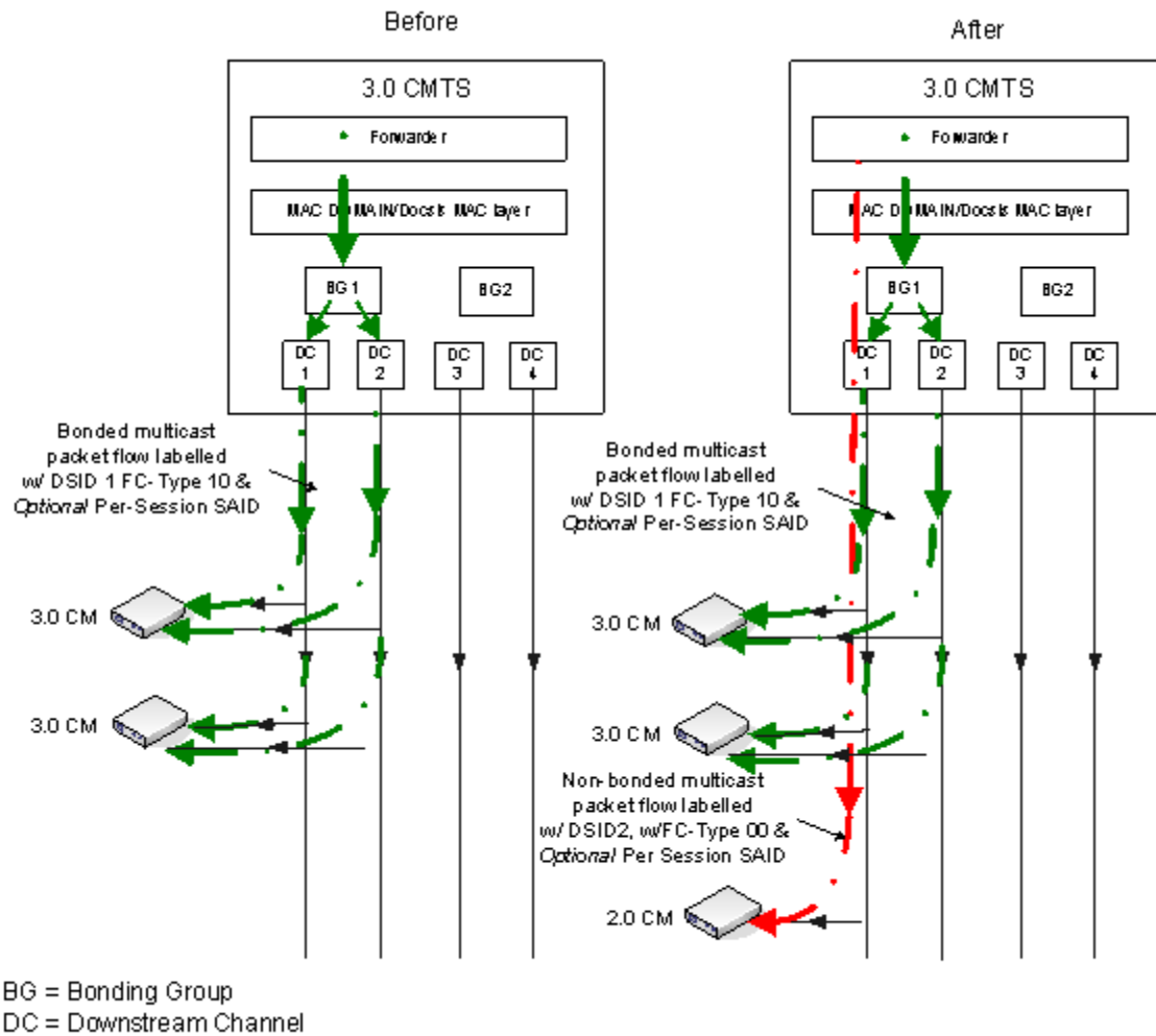
Figure 316 - Bonded and Non-bonded Replications of a Multicast Session on an Overlapping Downstream Channel Using FC 10 Isolation Technique (Subcase 2)
