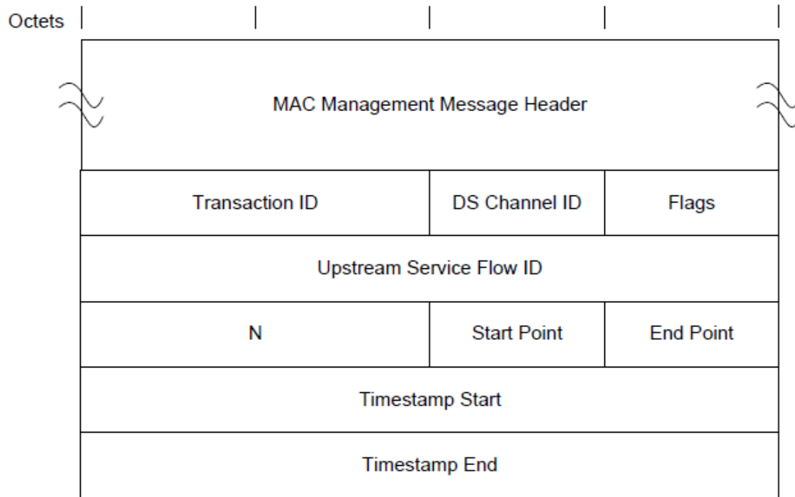
Figure 76 - DPV-RSP MAC Message
