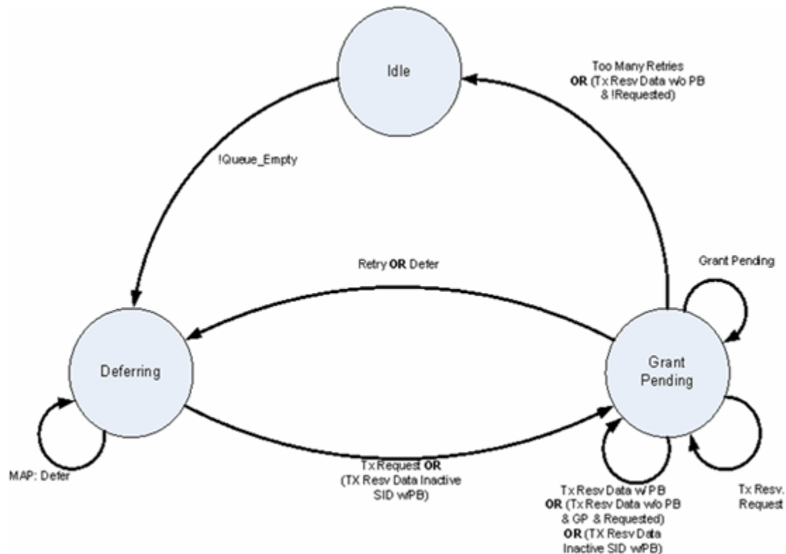
Figure 305 - Transmission and Deference State Transition Diagram (Multiple Transmit Channel Mode)
