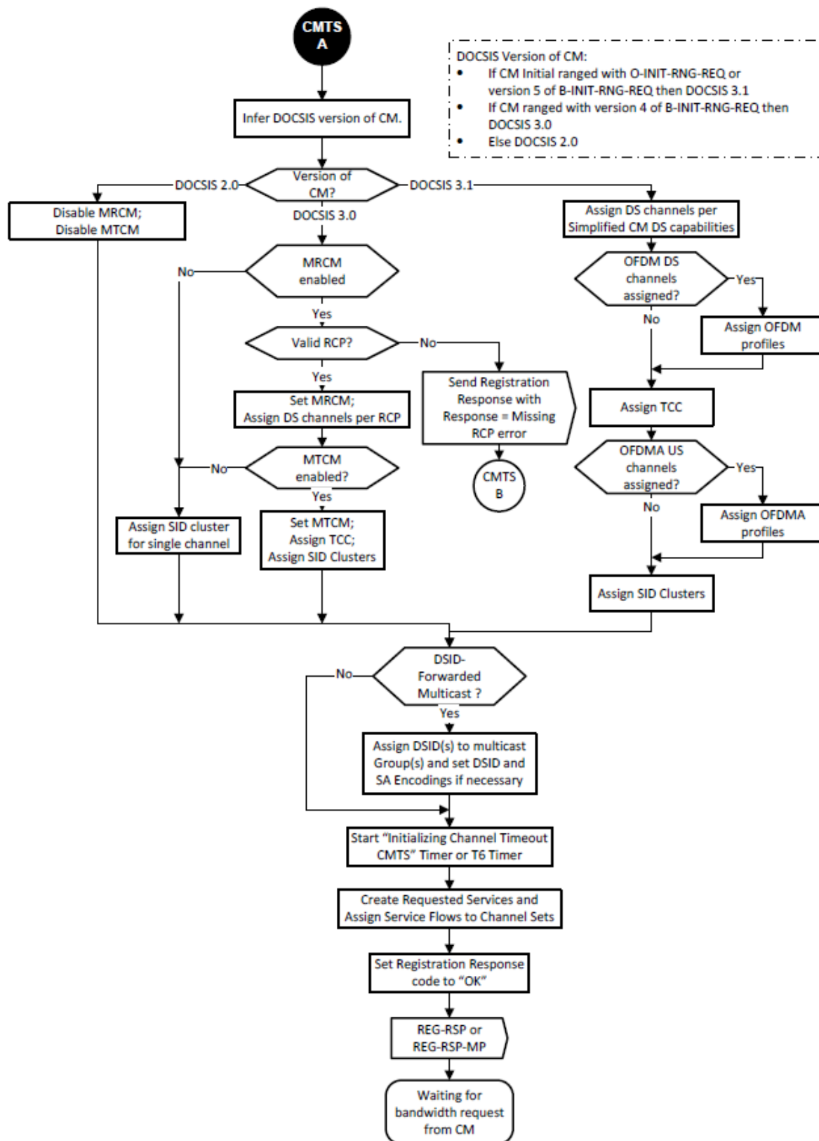
Figure 176 - CMTS Registration – Continued
