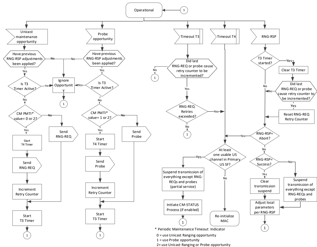
Figure 179 - Periodic Ranging - CM View
