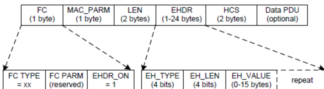
Figure 30 - Extended MAC Format
