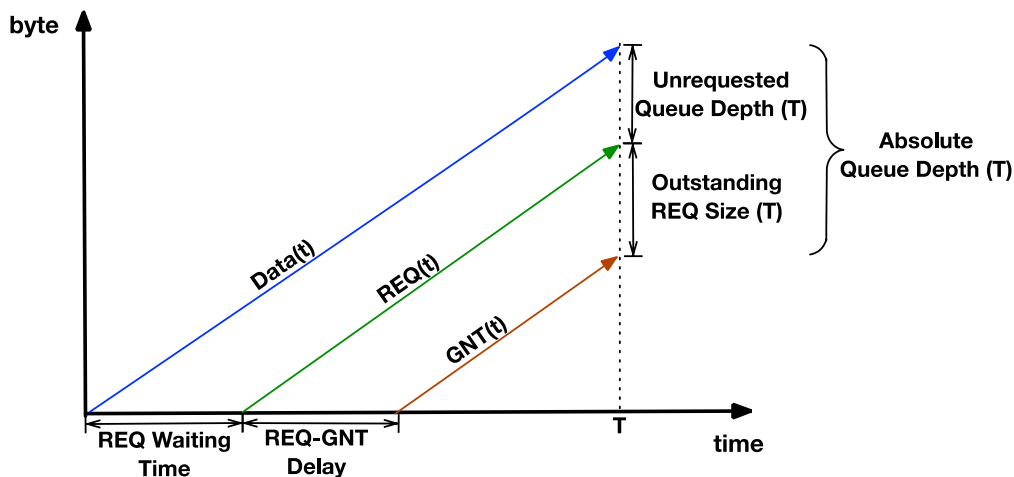
Figure 108 - Relationship Between the Unrequested Queue Depth and the Absolute Queue Depth With Respect to Requests and Grants
