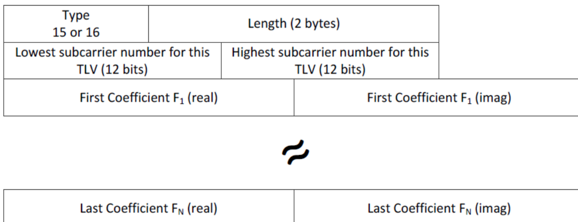
Figure 53 - Equalization Coefficient Encodings for OFDMA Channels
