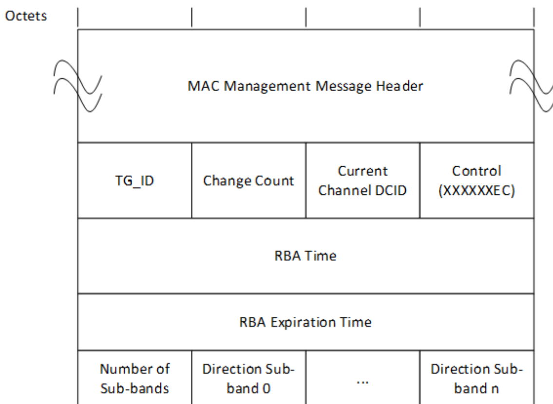
Figure 93 - Resource Block Assignment Message
