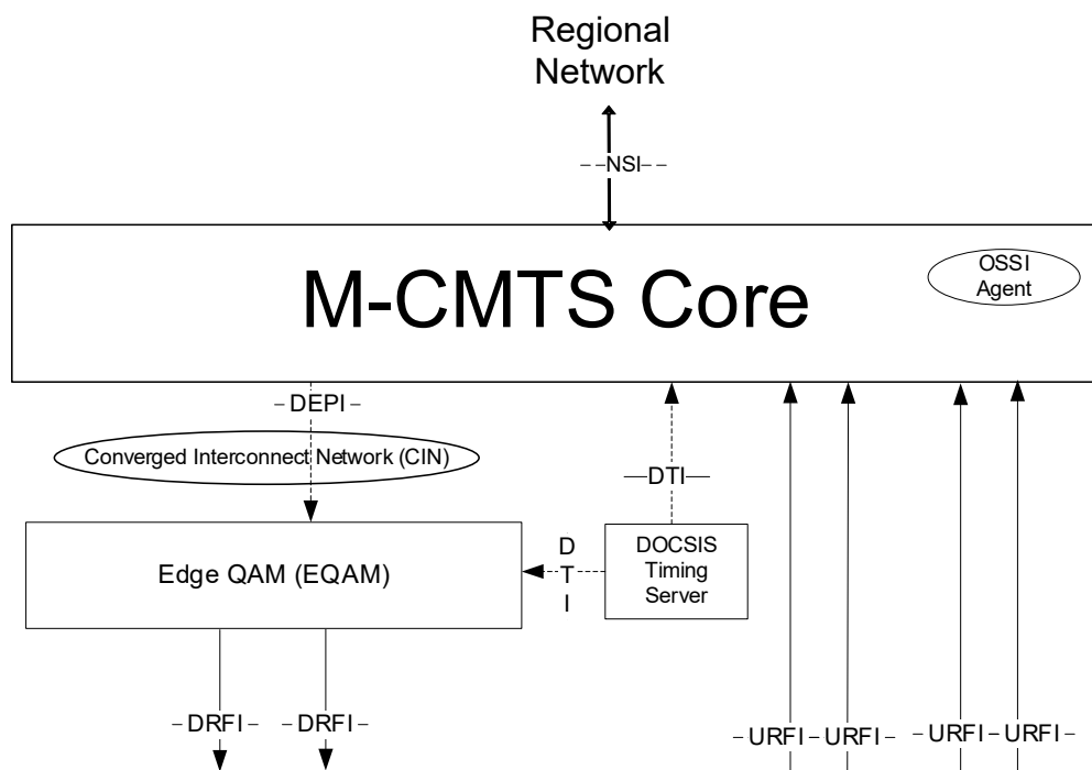
Figure 7 - Modular CMTS Network Diagram (Legacy)
