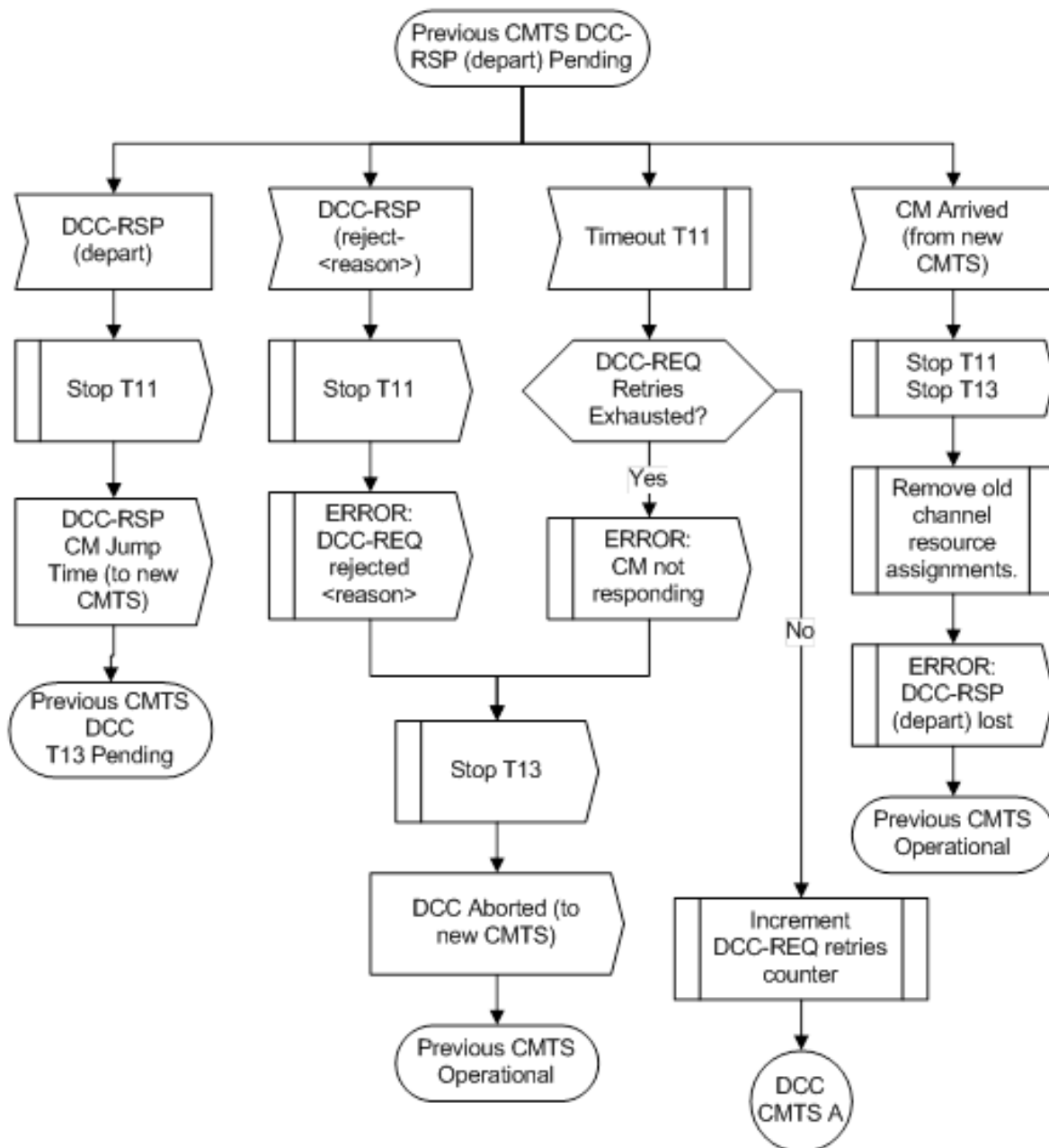
Figure 240 - Dynamically Changing Channels: CMTS View Part 2
