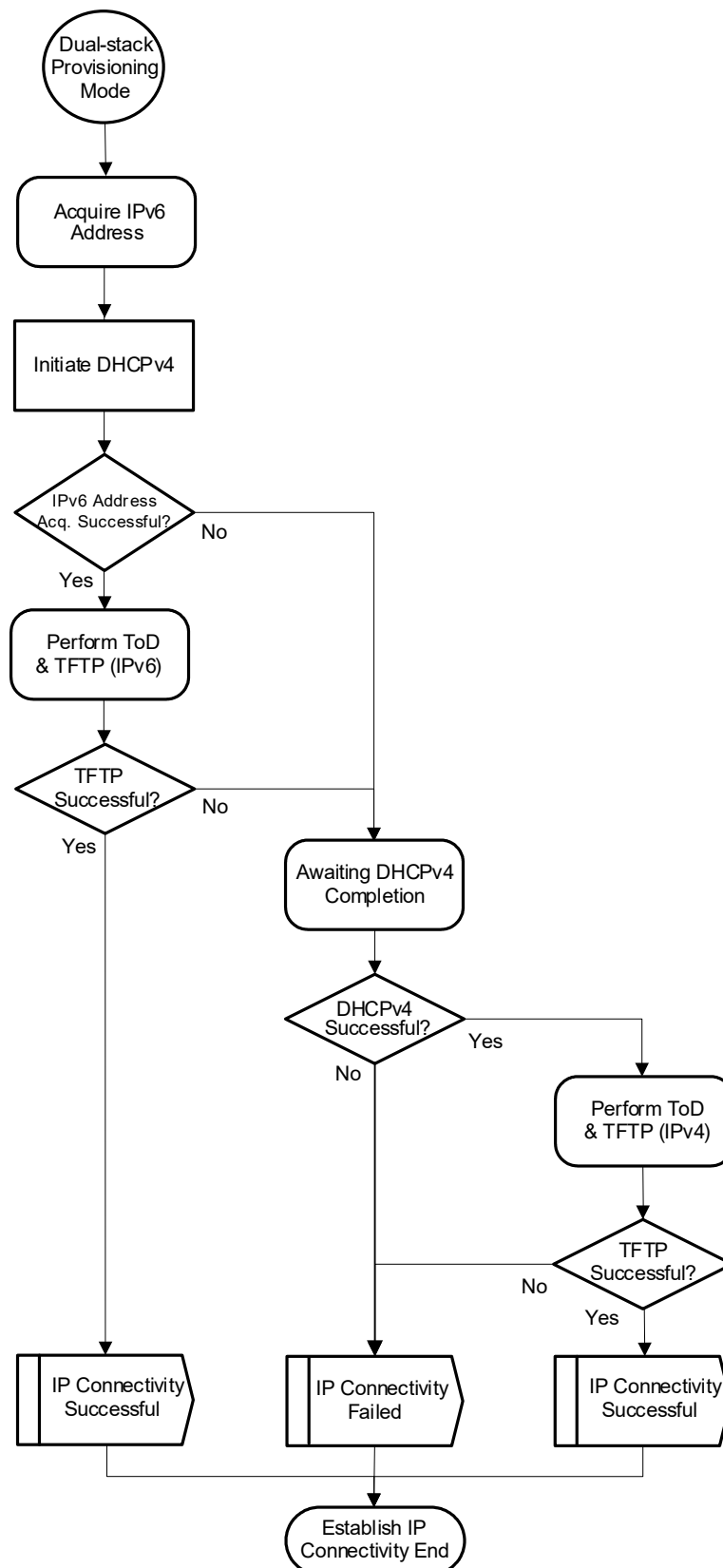
Figure 163 - Dual-stack Provisioning Mode
