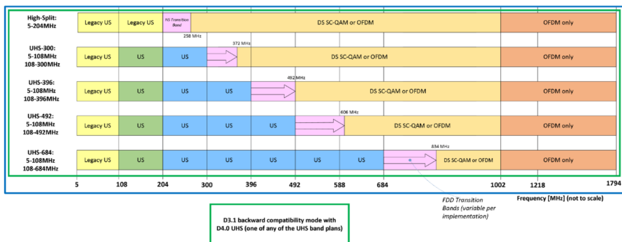
Figure 292 - FDD Spectrum Usage Alternatives: CMTS/RPD Node View
