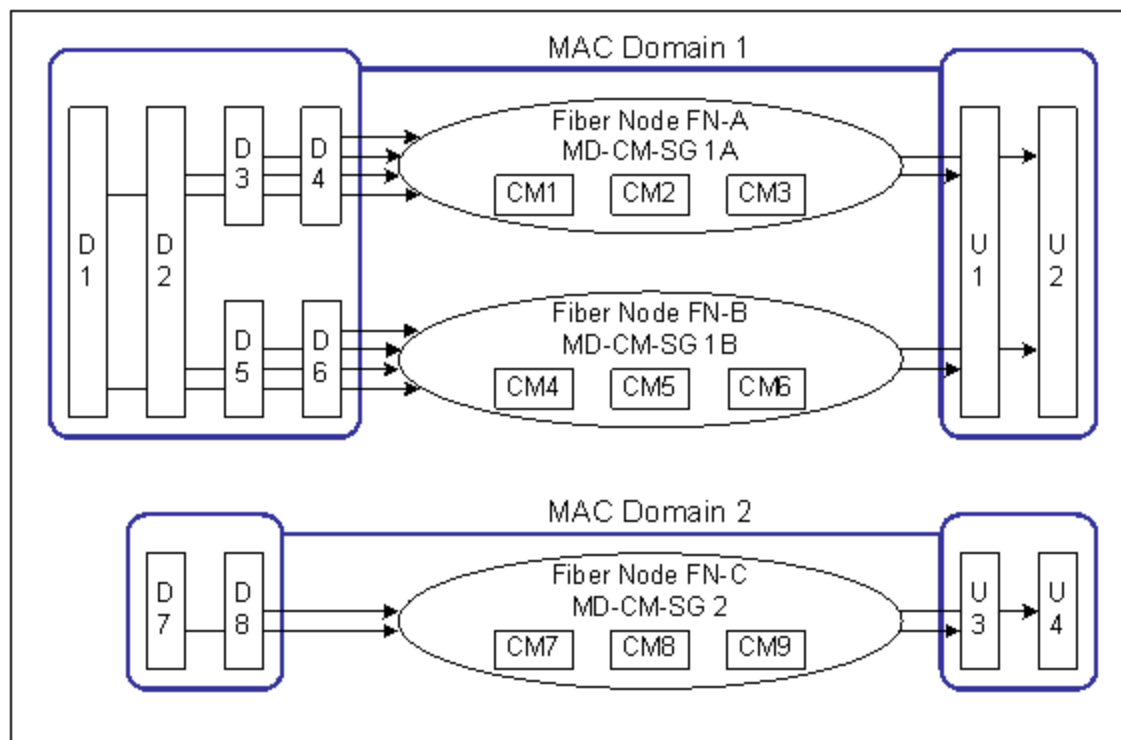
Figure 17 - Example MAC Domain Channel Assignment
