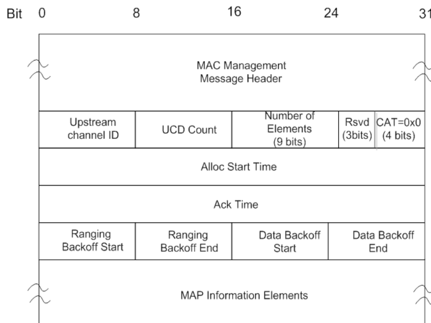
Figure 40 - Version 5 MAP Format for Non-Probe Frames
