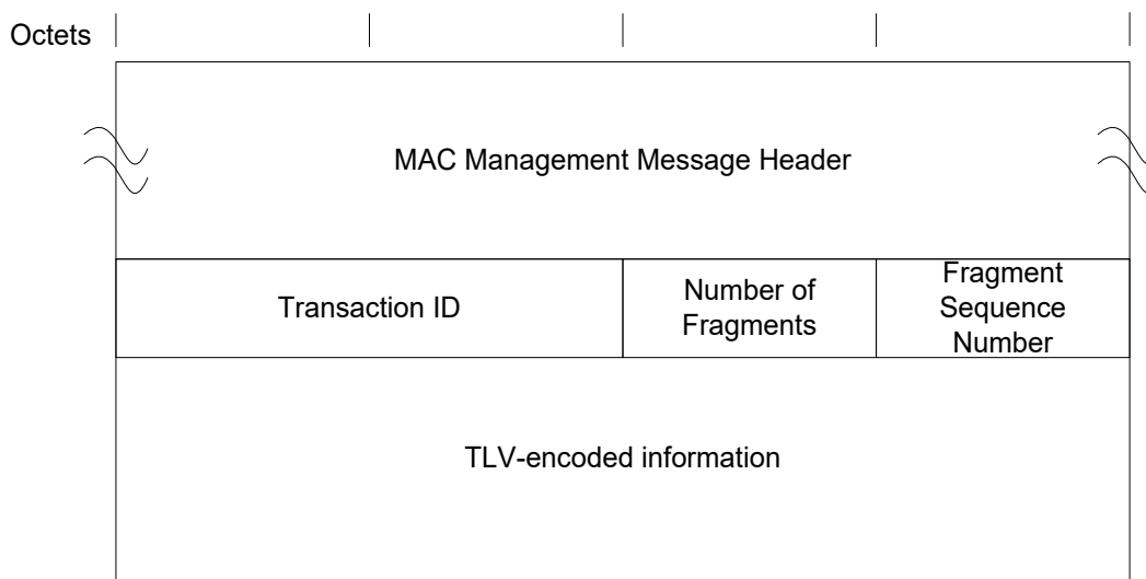
Figure 72 - Dynamic Bonding Change Request Message
