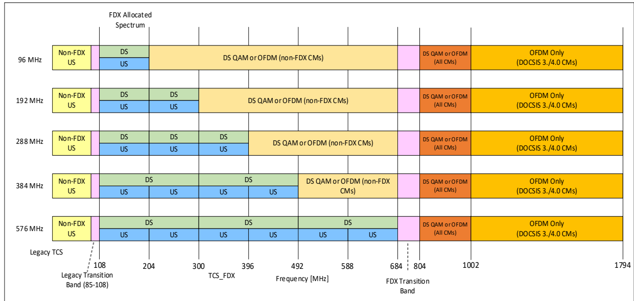
Figure 265 - Configurable FDX Allocated Spectrum Bandwidths for CFDX Band Plan with 1794 MHz Downstream Upper Band Edge
