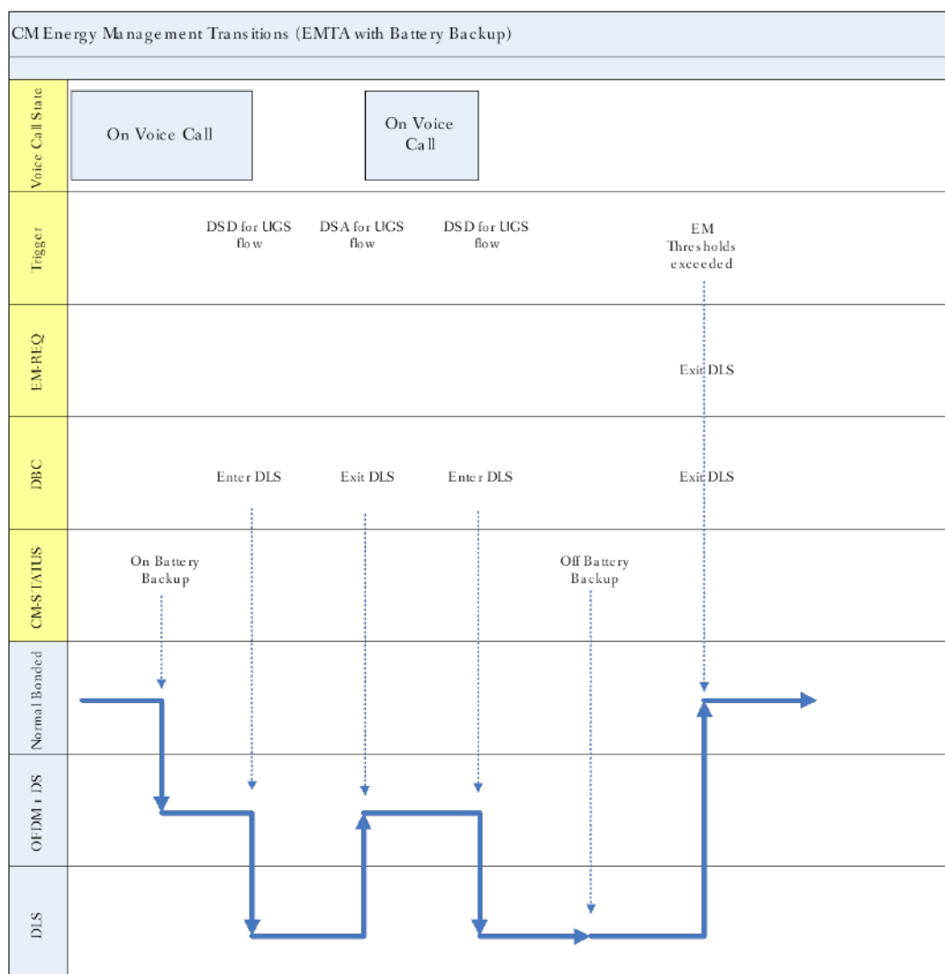
Figure 263 - Example Interaction Between Battery Backup and DLS Mode
