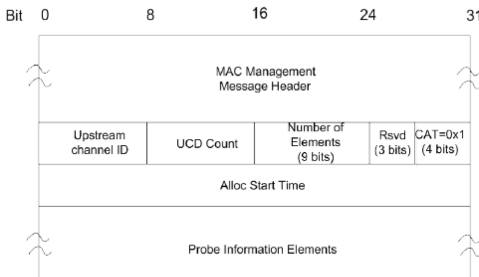
Figure 42 - Version 5 MAP Format for Probe Frames (P-MAPs)
