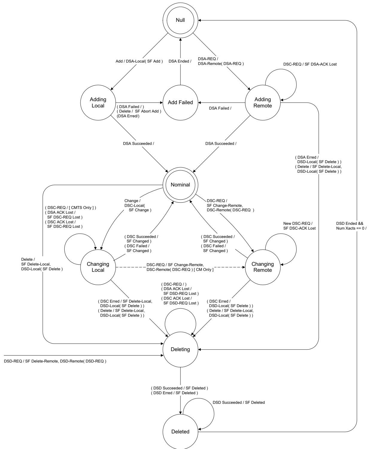
Figure 202 - Dynamic Service Flow State Transition Diagram
