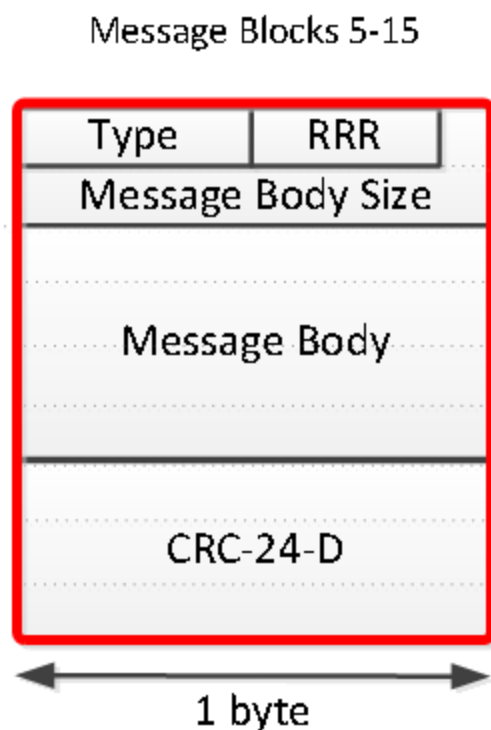
Figure 105 - Generic Format for Message Blocks 5–15
