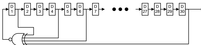
Figure 185 - Linear Feedback Shift Register for Synthetic Data Generation
