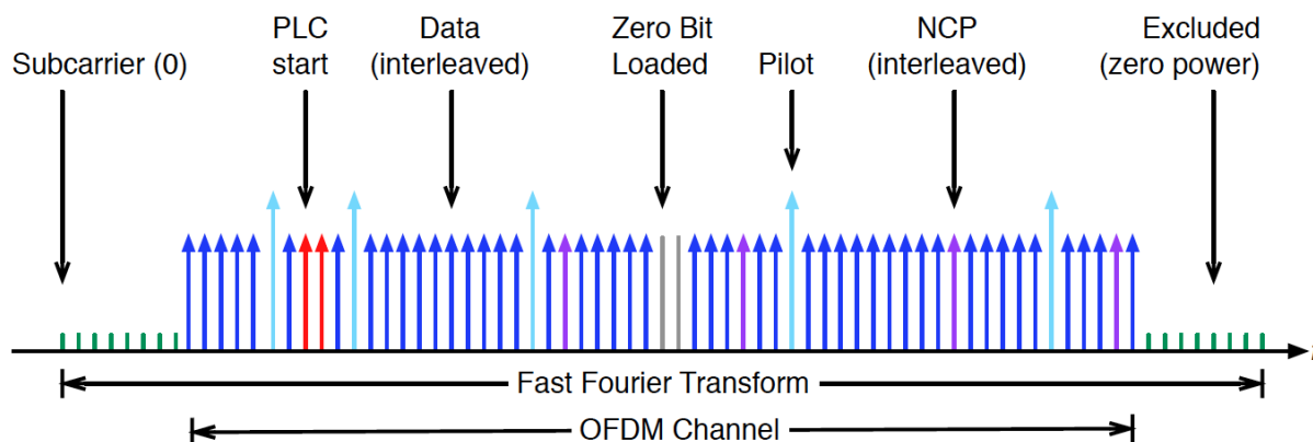
Figure 85 - OFDM Channel with PLC After Interleaving
