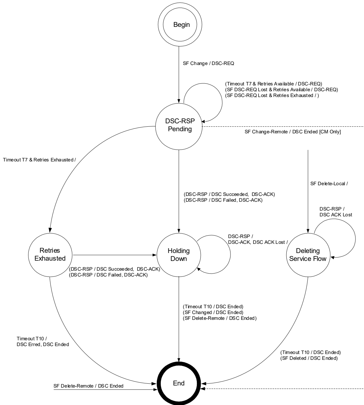
Figure 205 - DSC-Locally Initiated Transaction State Transition Diagram
