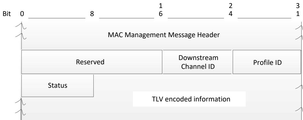
Figure 87 - The OFDM Profile Test Response (OPT-RSP) Message
