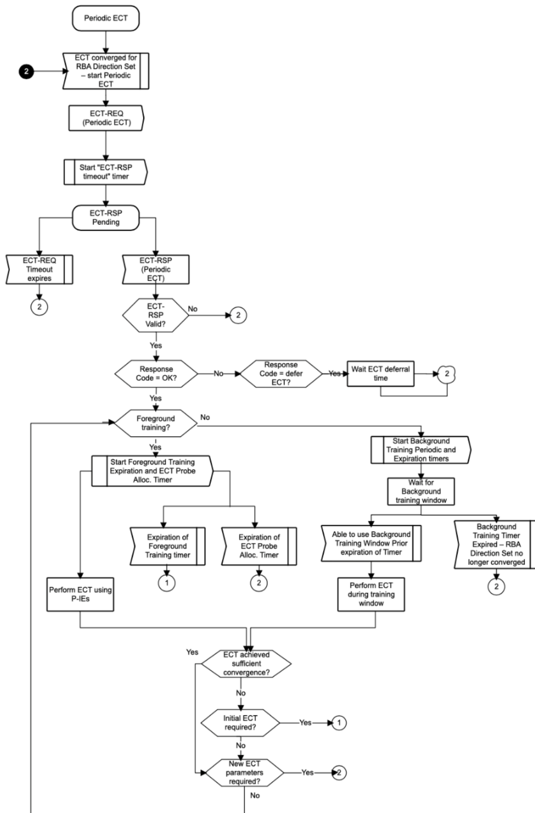
Figure 284 - CM Periodic EC Training SDL
