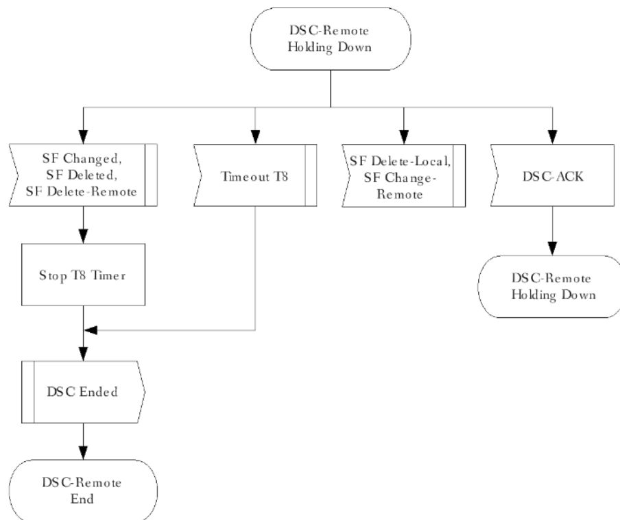
Figure 230 - DSC-Remotely Initiated Transaction Holding Down State Flow Diagram
