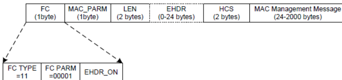
Figure 25 - Management MAC Header
