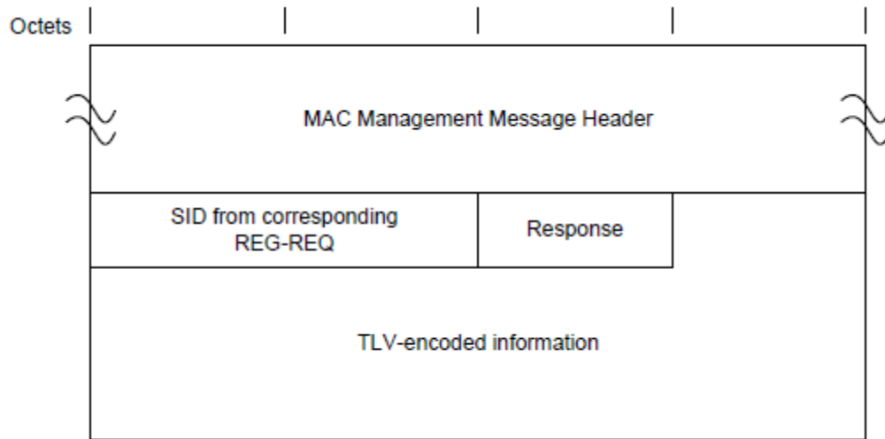
Figure 56 - Registration Response Format
