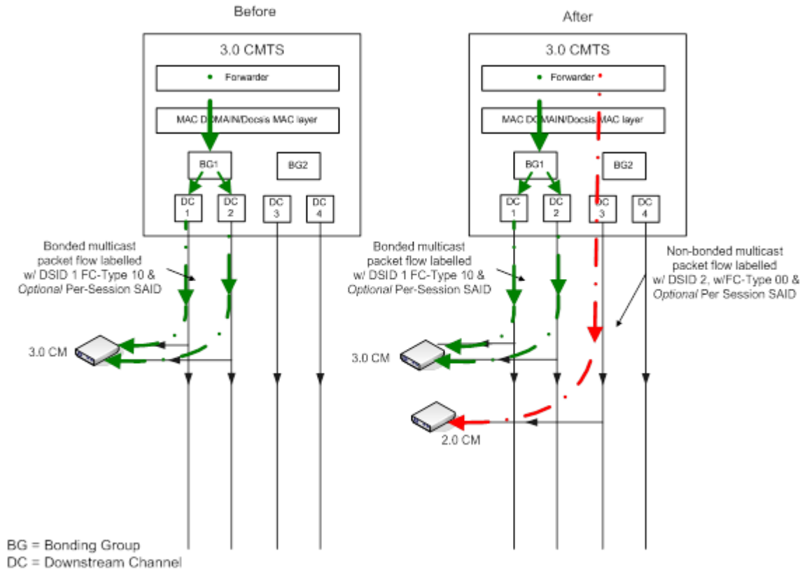
Figure 317 - Multicast Session Replications to Clients Behind Both a 3.0 CM and a 2.0 CM on Different Downstream Channel (Subcase 3)
