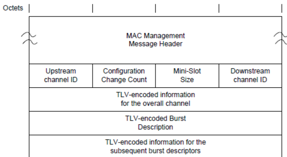
Figure 34 - Upstream Channel Descriptor
