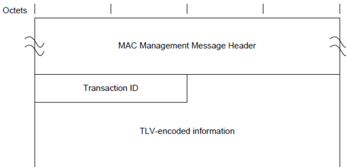
Figure 67 - Dynamic Channel Change Request
