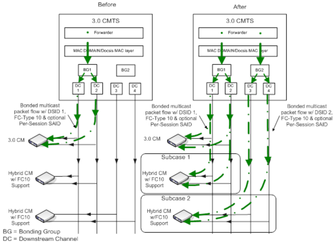
Figure 318 - Multicast Session Replication to Clients Behind Both a 3.0 CM and a Hybrid CM w/ FC-Type 10 Support
