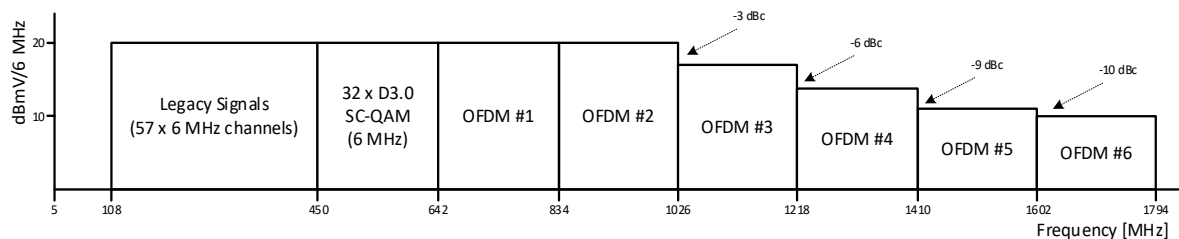
Figure 33 - Example Transmission Profile at Interface C (Multiple Step-down)
