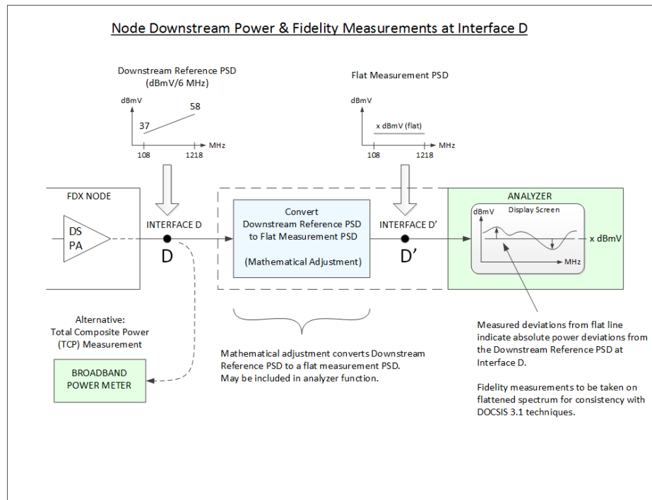
Figure 14 - FDX Node Downstream Power Measurement at Interface D
