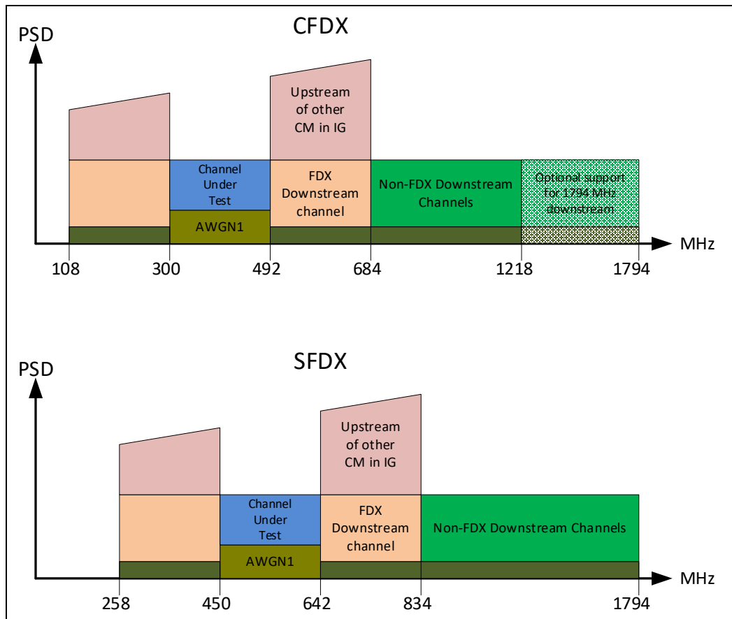
Figure 17 - State 1 for the External ACI Test
