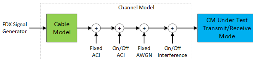
Figure 19 - Test Set-Up for Self ACI Test
