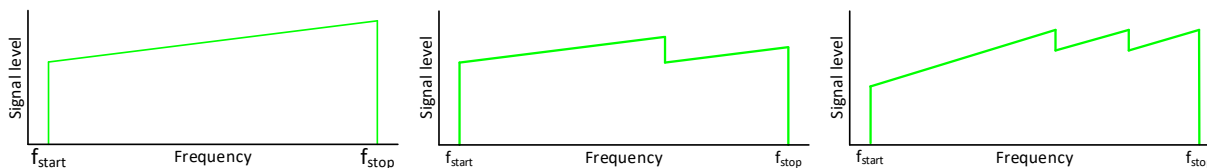
Figure 37 - Examples of Ways to Manage Maximum TCP: Constant Tilt (left), Tilt with Single Stepdown (center), and Tilt with Multiple Stepdowns (right)
