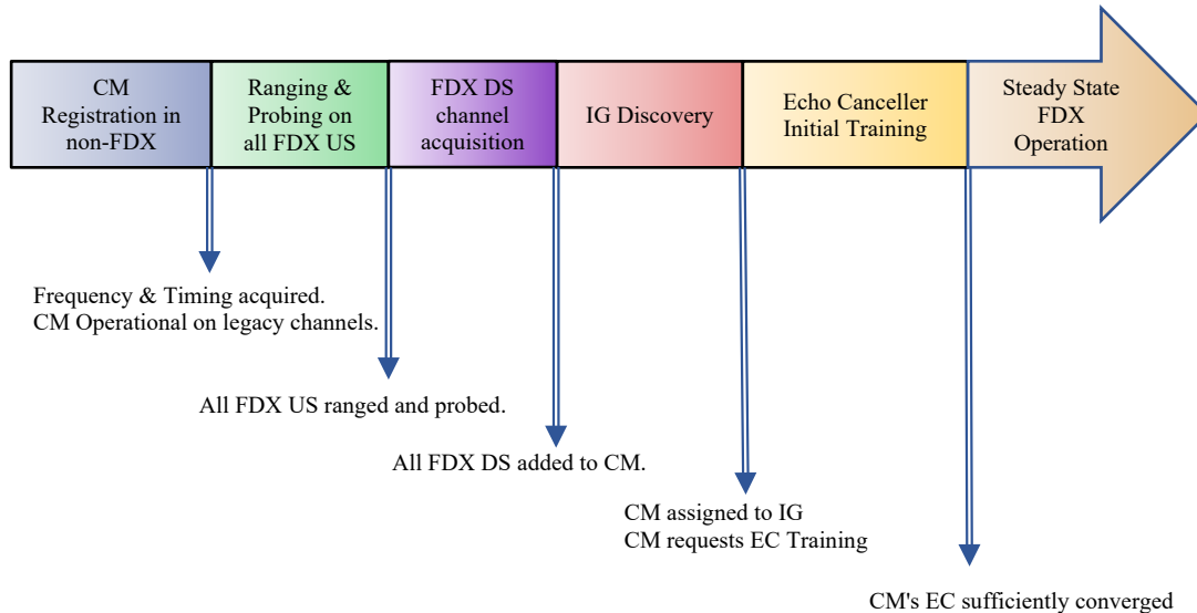
Figure 24 - CM FDX Entry Sequence
