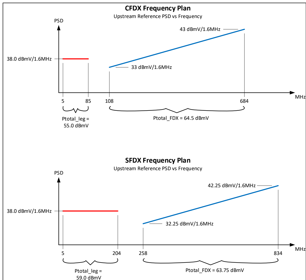
Figure 9 - Upstream Reference PSD for CFDX and SFDX Frequency Plans
