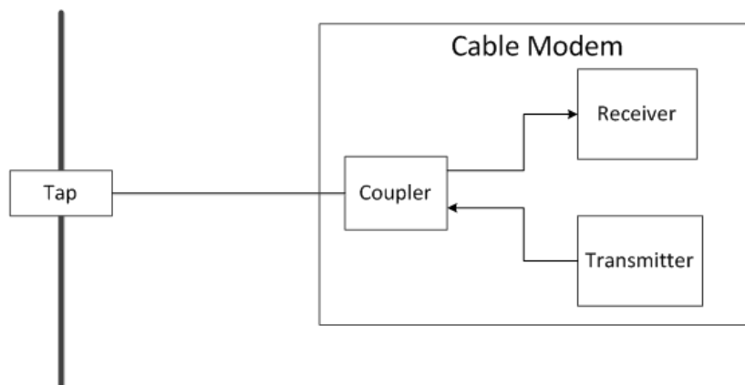
Figure 22 - Cable Modem and Drop Cable Schematic
