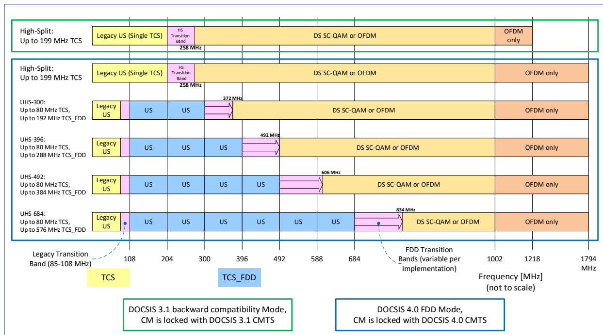
Figure 29 - Configurable FDD Upstream Allocated Spectrum Bandwidths
