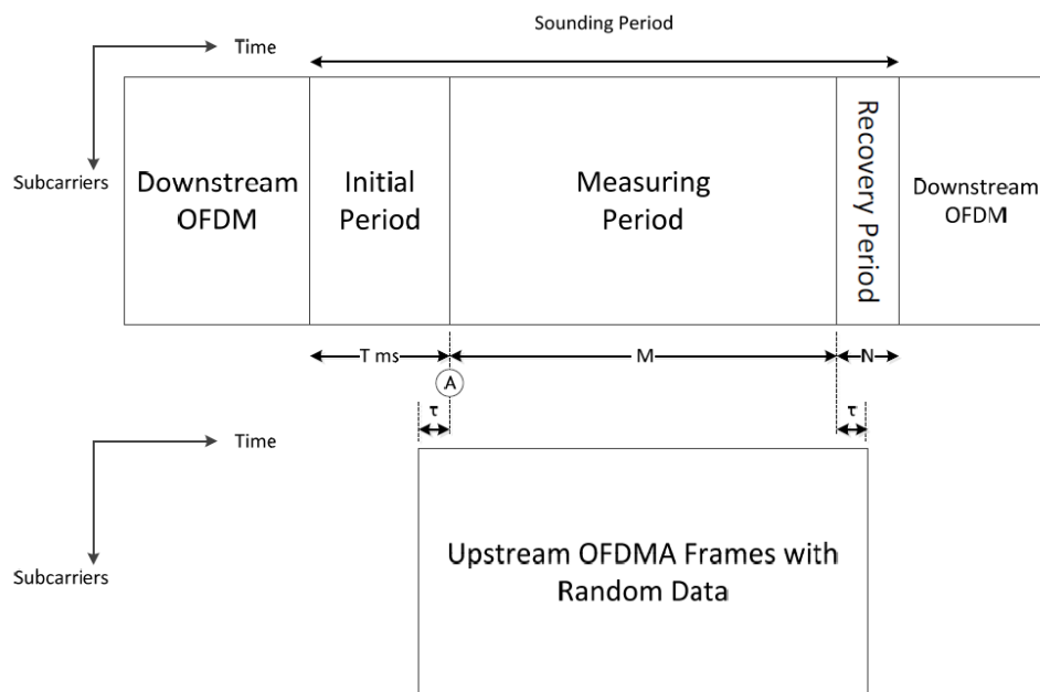
Figure 26 - Sounding Period for OUDP Method
