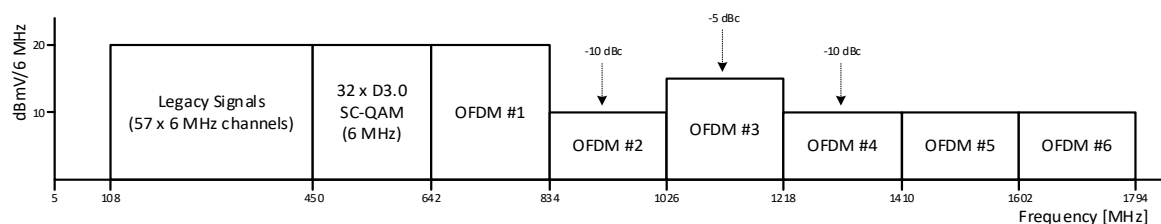
Figure 34 - Example Transmission Profile at Interface C (Step-up)
