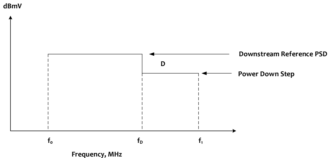
Figure 31 - Downstream Power RPD Step Down with D dB at F(D) MHz
