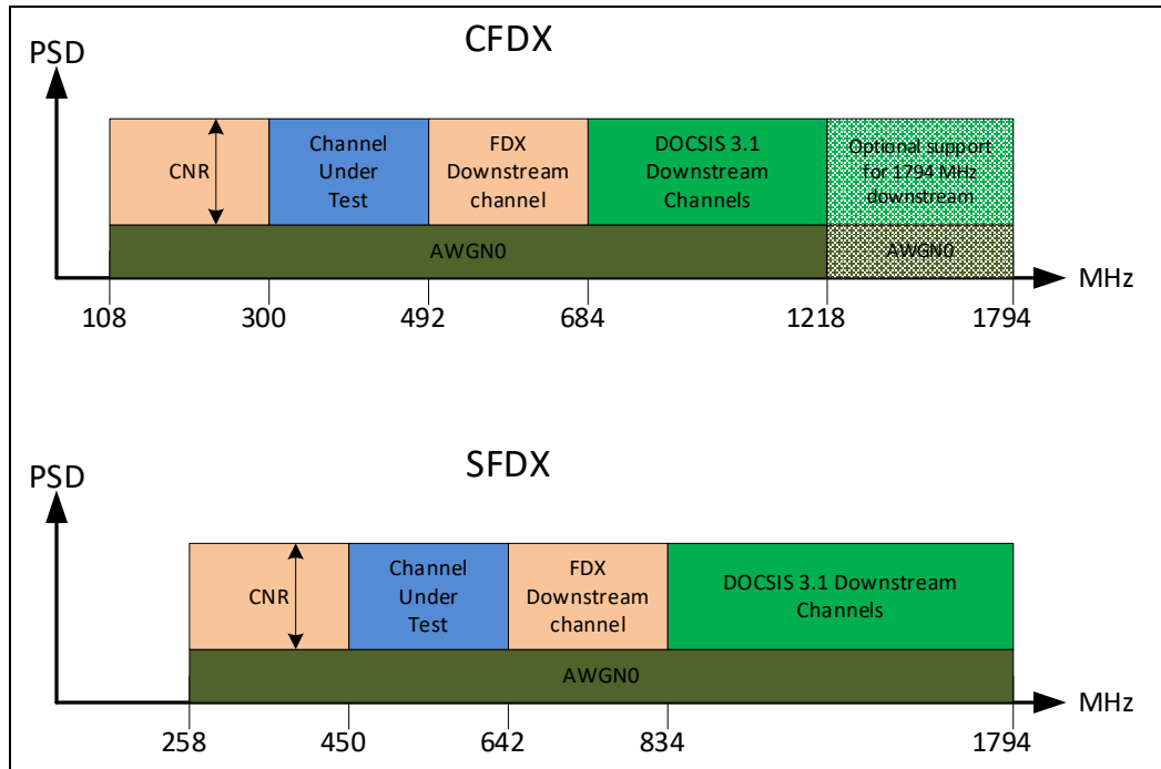
Figure 16 - State 0 for the External ACI Test
