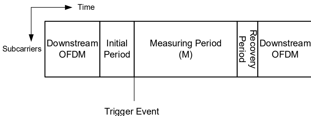
Figure 27 - Generic Triggered Measurement
