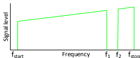
Figure 38 - Example of a Gap in the Power Spectrum Lowering TCP
