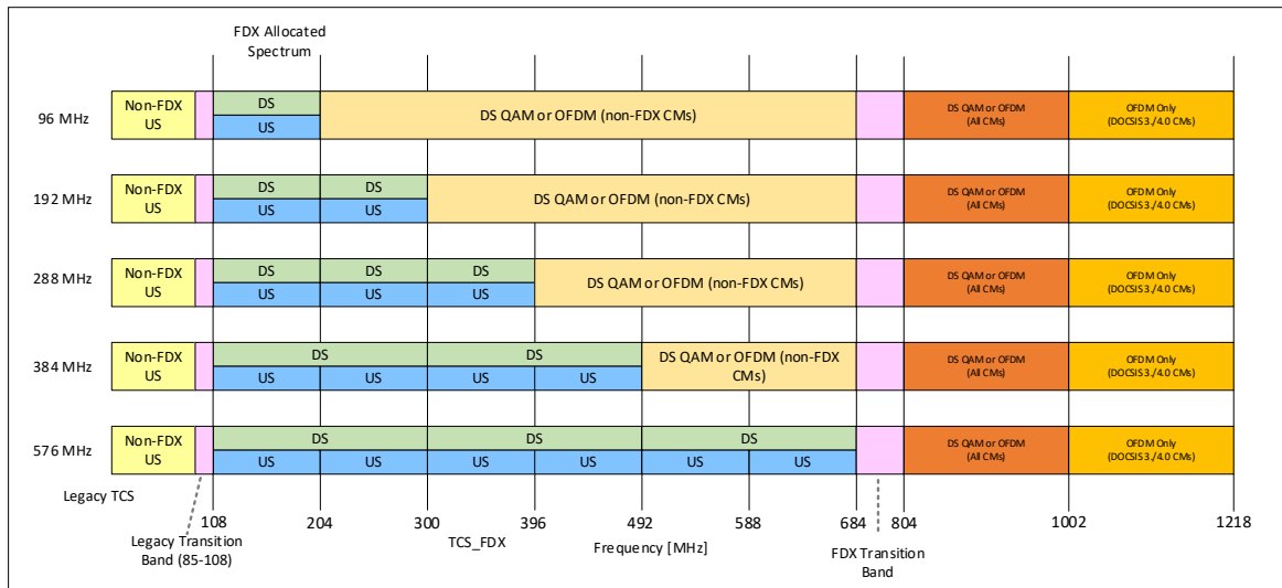
Figure 5 - Configurable FDX Allocated Spectrum Bandwidths for CFDX Frequency Plan - 1218 MHz Downstream
