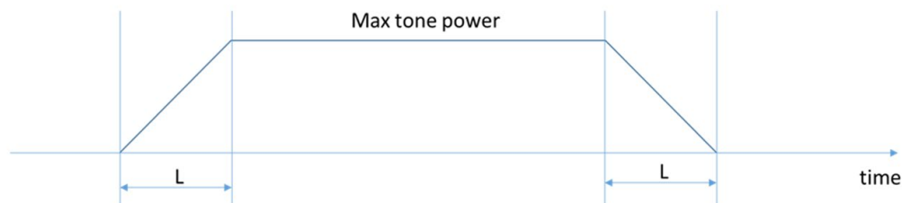
Figure 21 - CW Tone Power Ramp Up and Ramp Down in Start and End to Reduce ICI to Adjacent Subcarriers
