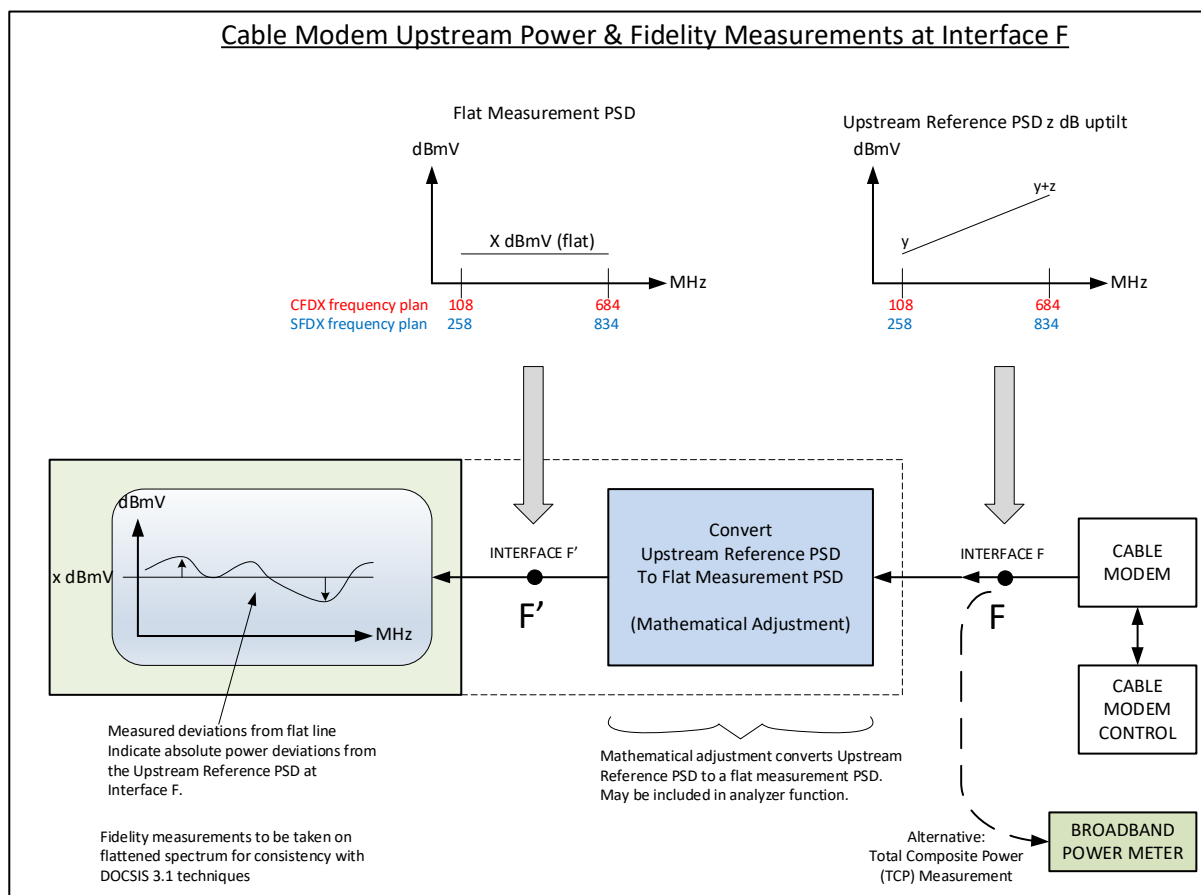
Figure 8 - FDX Cable Modem Upstream Power and Fidelity Measurements at Interface F
