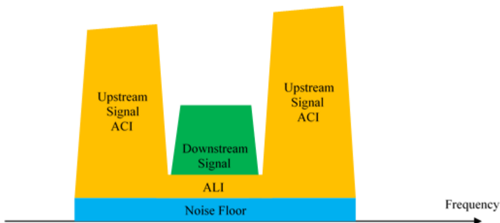
Figure 23 - ALI and ACI Illustrated in the Spectral Plane
