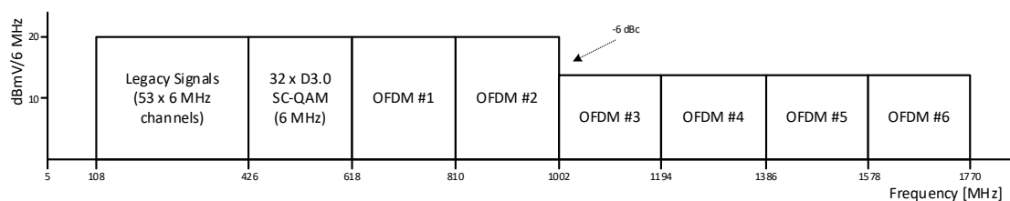
Figure 35 - Example Transmission Profile at Interface C (Single 6-dB Step-down at 1002 MHz)
