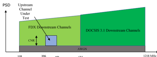
Figure 11 – Example Spectrum at Interface D for the Node Receiver PER Test, CFDX Frequency Plan
