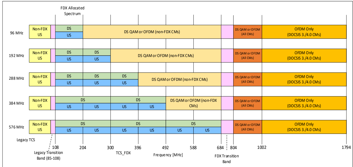
Figure 6 - Configurable FDX Allocated Spectrum Bandwidths for CFDX Frequency Plan - 1794 MHz Downstream
