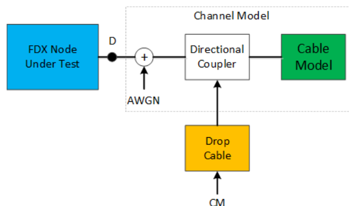
Figure 10 - Set-up for the FDX Node Packet-Error-Ratio Performance Test
