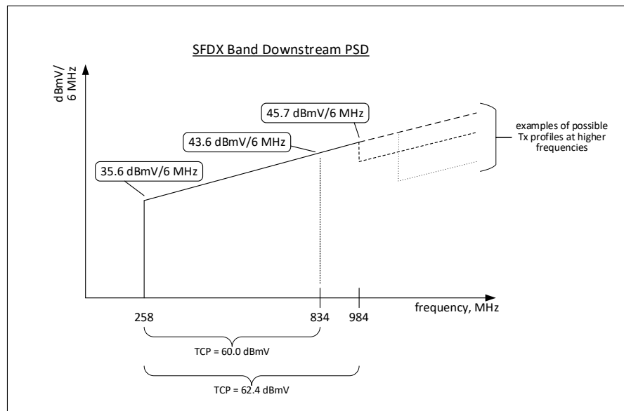
Figure 12 - The SFDX Band Downstream PSD vs. Frequency
