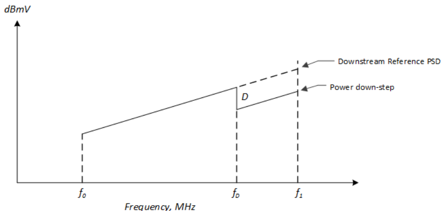
Figure 13 - Downstream Power Profile with D dB Step-down at f_D MHz
