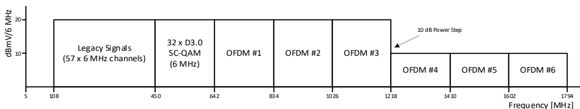
Figure 32 - Example Transmission Profile at Interface C (Single Step-down at 1218 MHz)
