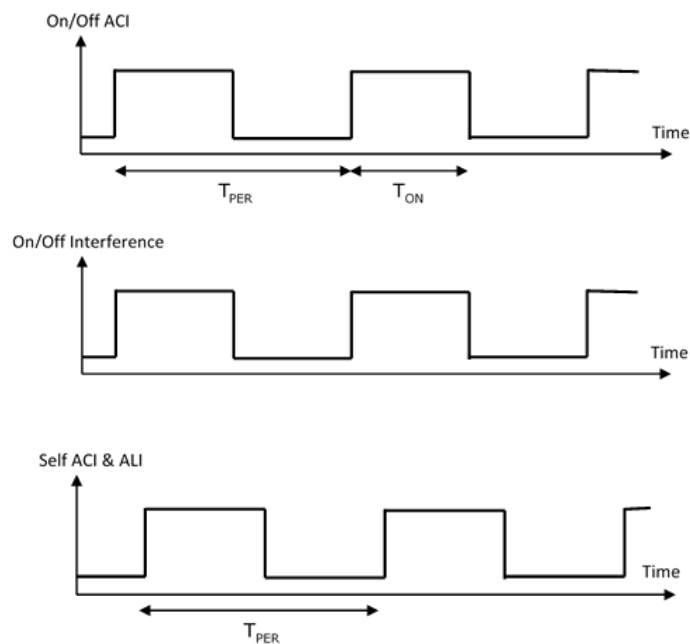
Figure 20 - Time-Varying ACI and AWGN for Self ACI Test
