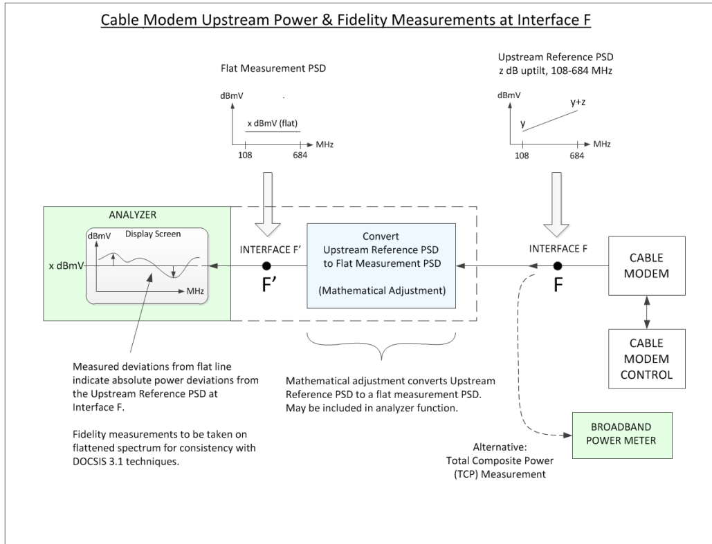
Figure 30 - FDD Cable Modem Upstream Power and Fidelity Measurements at Interface F'
