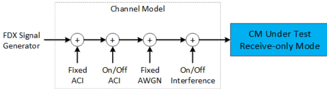
Figure 15 - Test Set-Up for External ACI Test
