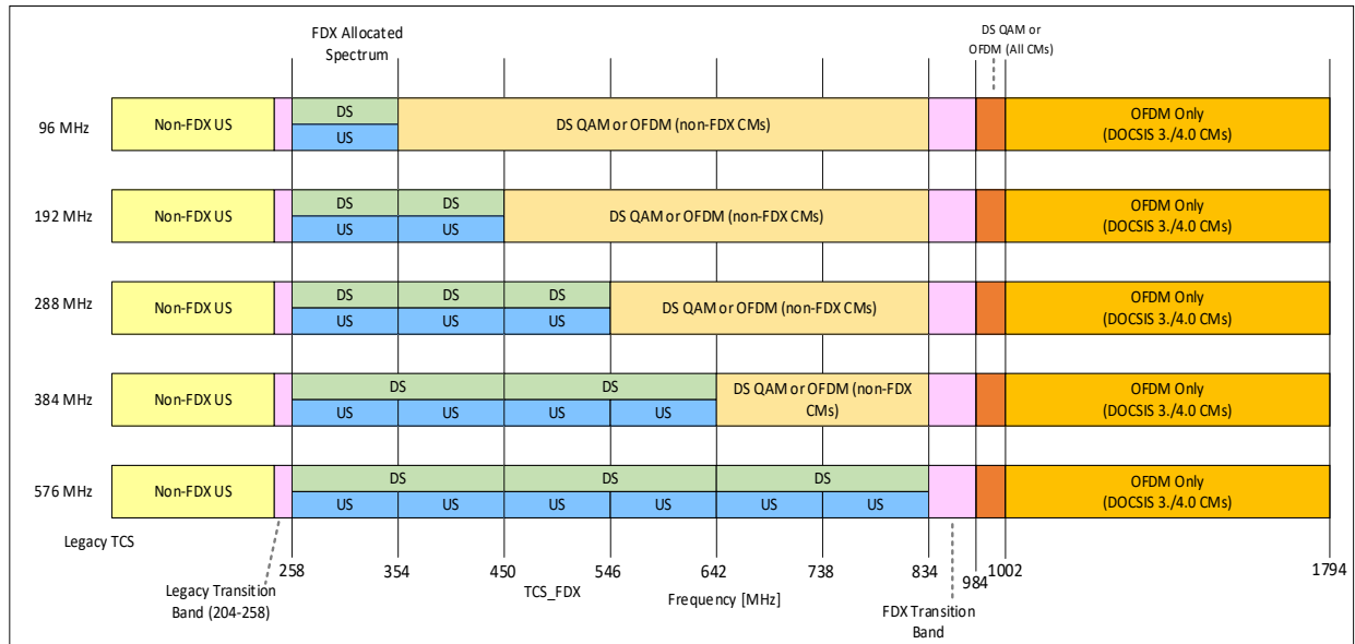
Figure 7 - Configurable FDX Allocated Spectrum Bandwidths for SFDX Frequency Plan
