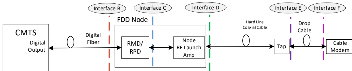
Figure 28 - FDD Node Reference Interfaces
