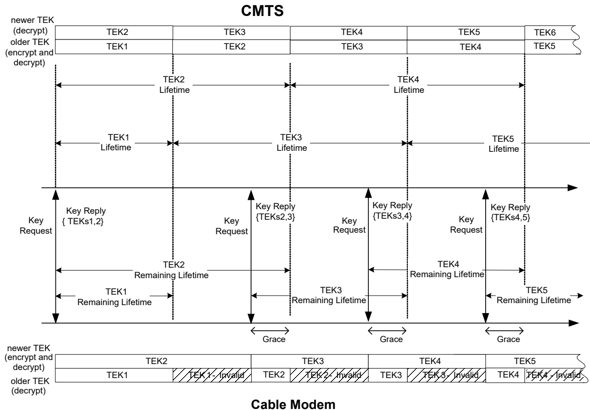
Figure 13 - TEK Management in CMTS and CM
