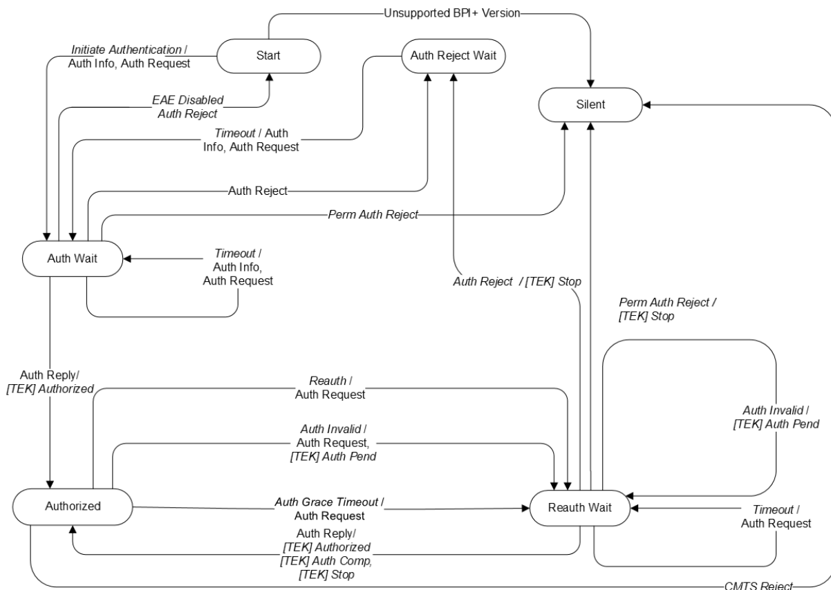
Figure 9 - Authorization State Machine Flow Diagram
