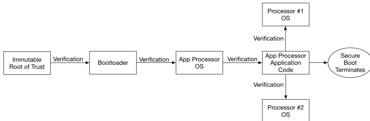
Figure 17 - Immutable Root of Trust Example
