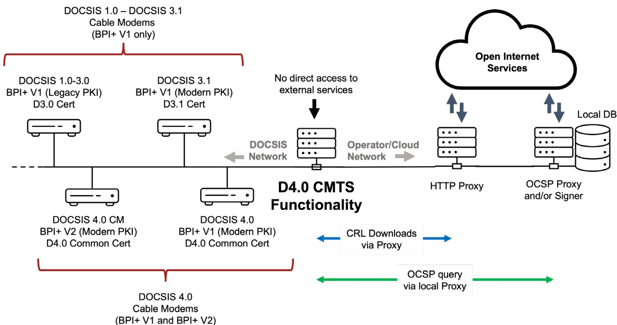
Figure 24 - Example Deployment with Revocation Checking Support and Local Overrides
