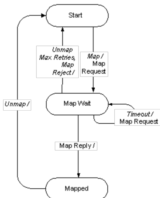
Figure 22 - SA Mapping State Machine Flow Diagram
