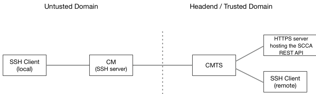
Figure 19 - TLS-Based Authentication Architecture
