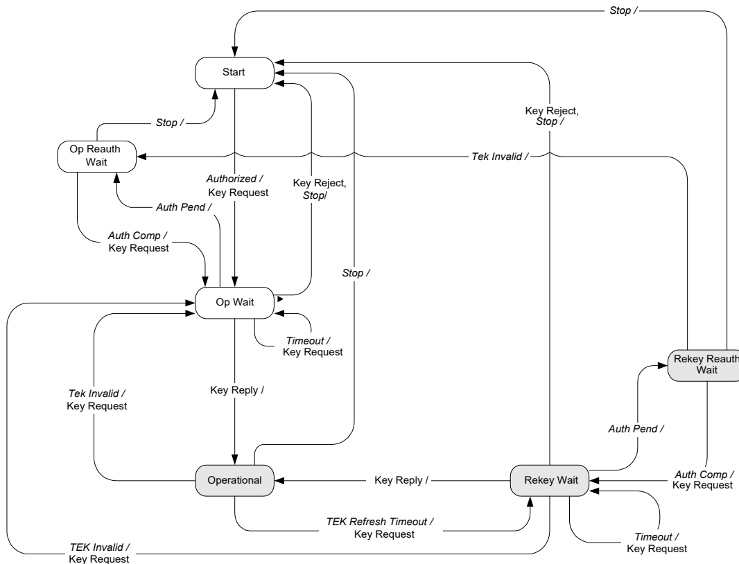
Figure 10 - TEK State Machine Flow Diagram
