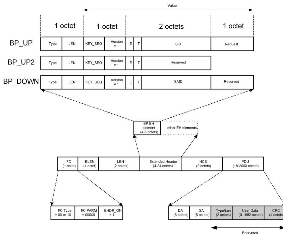
Figure 5 - Format of DOCSIS Variable-Length PDU with Baseline Privacy EH Element
