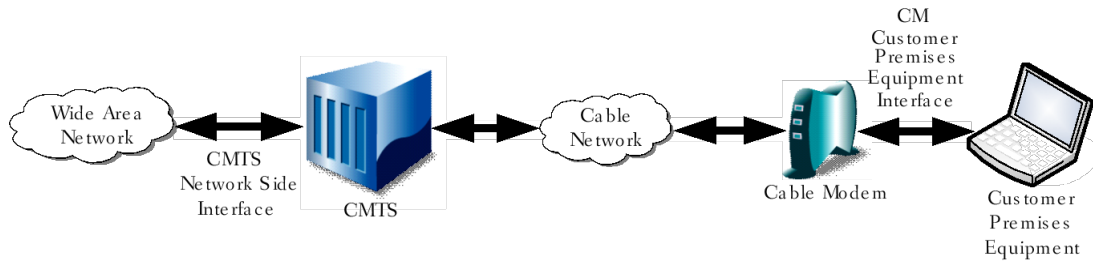
Figure 3 - Transparent IP Traffic Through the Data-Over-Cable System
