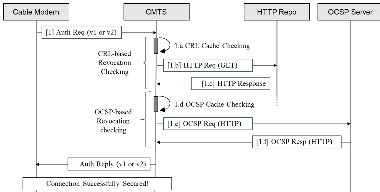
Figure 23 - Integrated BPI+ and Revocation Checking Flow
