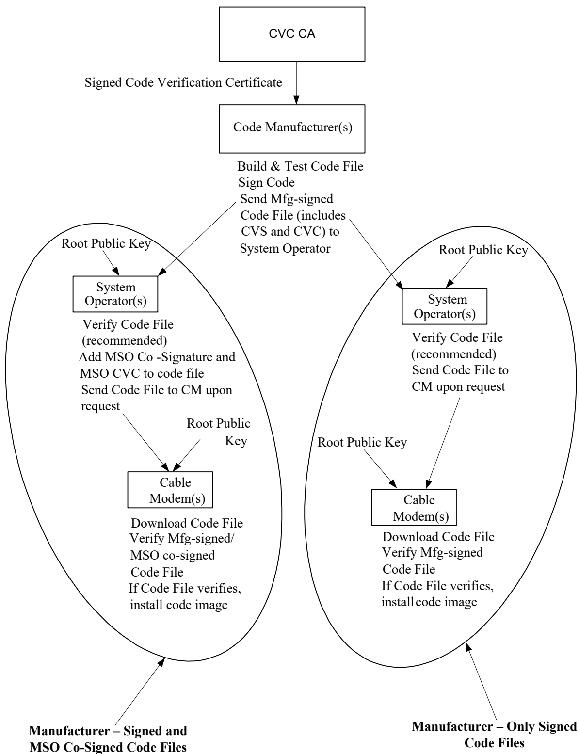
Figure 16 - Typical Code Validation Hierarchy
