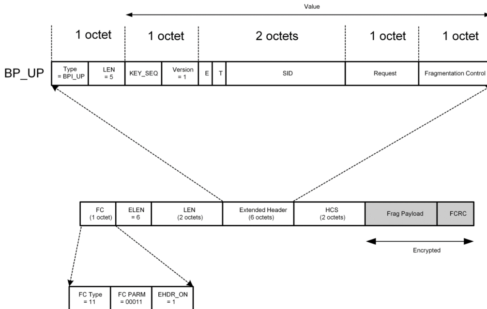
Figure 6 - Format of a DOCSIS MAC Fragmentation Frame with an Encrypted Payload
