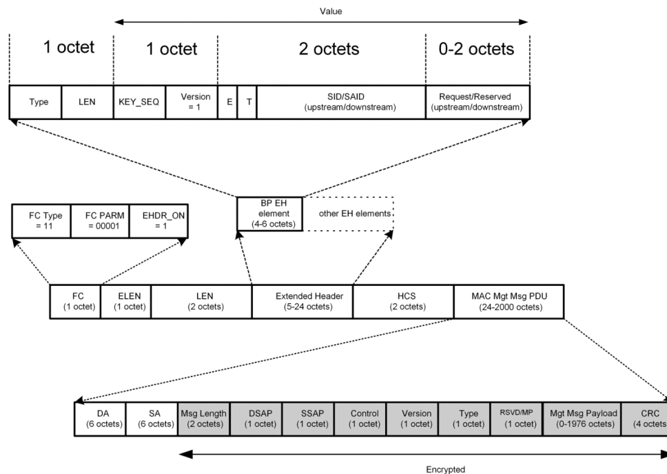
Figure 7 - Format of a DOCSIS MAC Management Message Frame with Encrypted Payload
