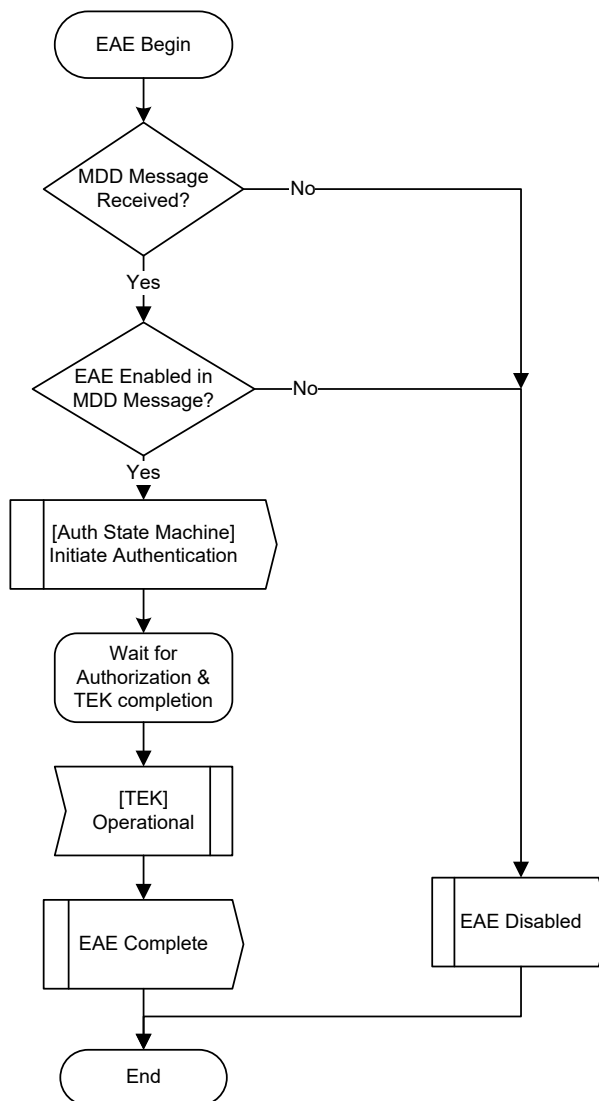
Figure 11 - EAE Signaling Flow Chart for CM
