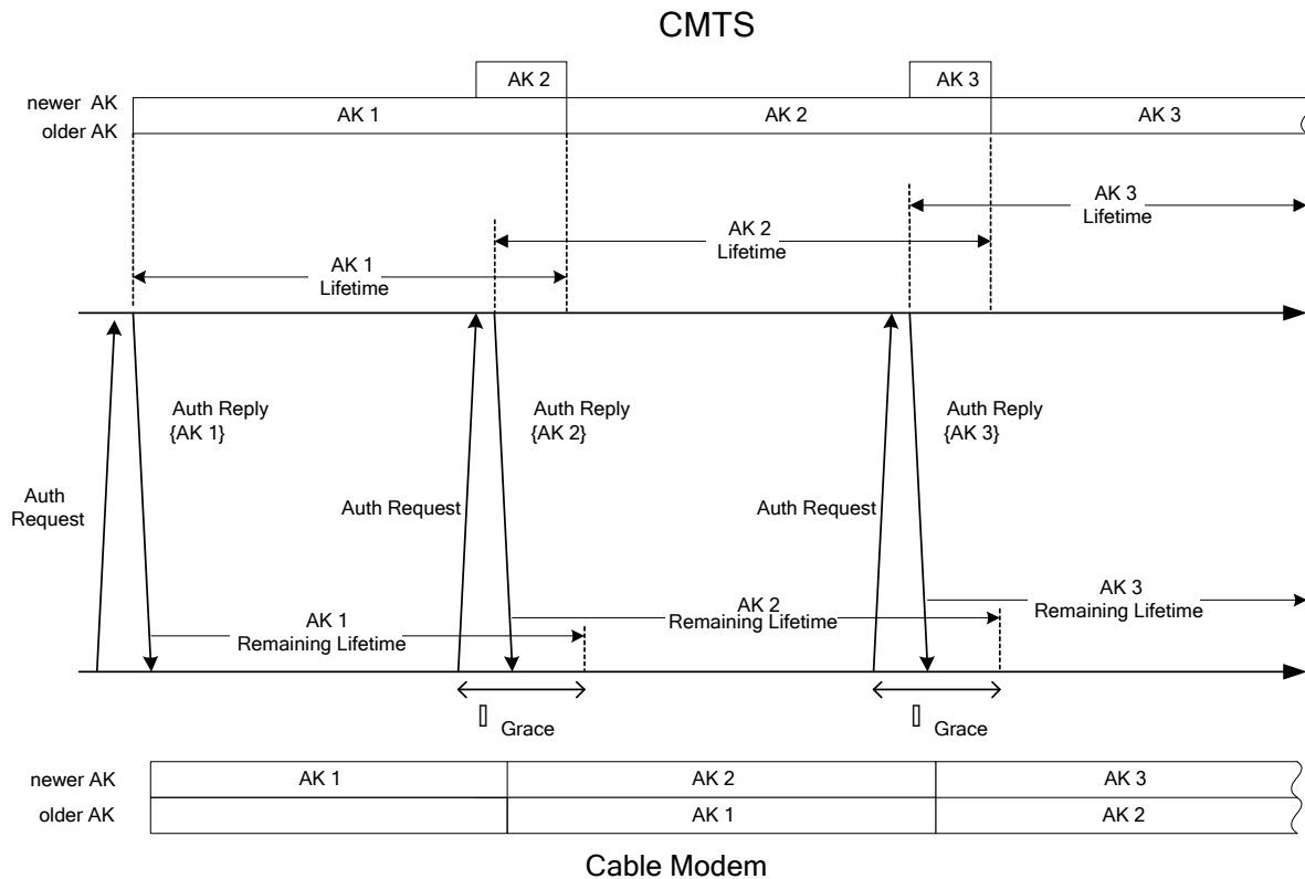
Figure 12 - Authorization Key Management in CMTS and CM
